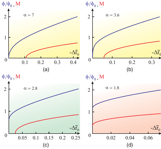
FIG. 9. (Color online) Nematic order parameter \phi (blue/dark gray curves) and magnetic order parameter M (red/light gray curves) as functions of -\Delta\bar{r}_0 = r_{0,cr} - r_0 \propto (T_s - T) for four different values of \alpha at d = 2.5 . In (a) and (b), we use \alpha > \alpha_{c2} = 3.5 (region III of the phase diagram), in (c), we use \alpha_{c2} > \alpha > \alpha_{c1} = 2 (region II of the phase diagram), and in (d), we use \alpha < \alpha_{c1} (region I of the phase diagram). \phi_0 is the value of \phi corresponding to \phi = r .
