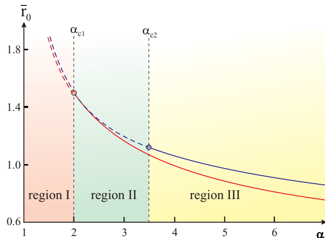
FIG. 8. (Color online) The calculated phase diagram in the (\alpha, \bar{r}_0) plane for the representative case d = 2.5 . In region I, there is a simultaneous nematic and magnetic first-order transition. In region II, the two transitions split, but the nematic transition remains first order, while the magnetic transition becomes second order. In region III, the nematic transition also becomes second order. The three regions are separated by two tricritical points. The temperature behavior of the nematic and magnetic order parameter in each region is shown in Fig. 9 below.
