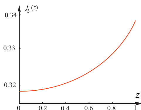
FIG. 17. (Color online) The function f_3(z) from Eq. (62).
