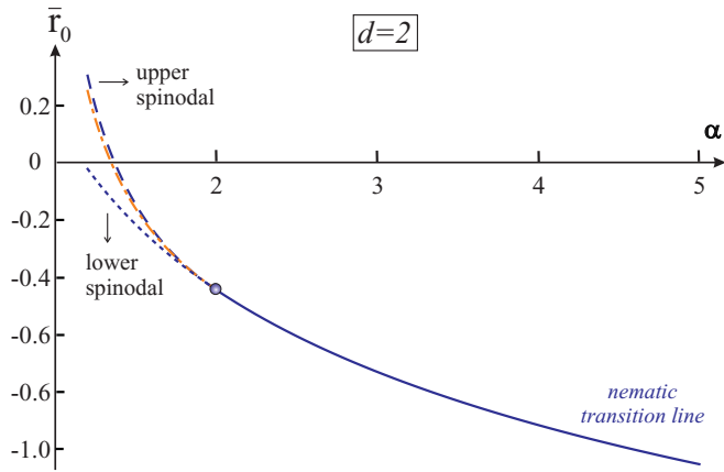
FIG. 5. (Color online) Calculated phase diagram in the (\alpha, \bar{r}_0) plane for the d = 2 case and high enough temperatures, where classical fluctuations dominate. In the region \alpha < 2 , the nematic transition is first order. The dashed blue/dark line represents the upper spinodal (where the ordered state becomes metastable), while the dotted blue/dark line denotes the lower spinodal (where the disordered state ceases to be metastable), and the dashed-dotted orange/light line is the actual transition line where the global minimum of S_{\text{eff}} shifts from \phi = 0 to \phi \neq 0 . We recall there is no magnetic order at a finite temperature in d = 2 . In this figure, we fixed \bar{u} = 1 and changed \bar{g} .
