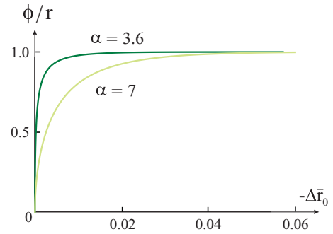
FIG. 10. (Color online) Nematic order parameter \phi , in units of the renormalized magnetic mass term r , as function of the reduced temperature -\Delta\bar{r}_0 = r_{0,cr} - r_0 \propto (T_s - T) at d = 2.5 for two different values of \alpha : \alpha = 7 , which is far from the nematic tricritical point \alpha_{c2} = 3.5 (light-green/light gray curve), and \alpha = 3.6 , which is very close to the nematic tricritical point (dark-green/dark gray curve). In both cases, \phi evolves continuously from zero, but the slope is very large for \alpha only slightly above \alpha_{c2} .
