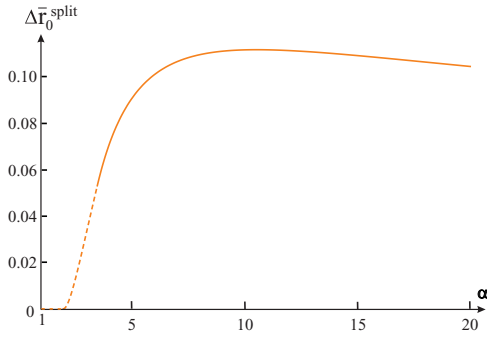
FIG. 11. (Color online) Splitting between the nematic and magnetic transitions, \Delta\bar{r}_0^{\text{split}} \equiv \bar{r}_0^{\text{nem}} - \bar{r}_0^{\text{mag}} , as function of \alpha \equiv u/g , for the case d = 2.5 . The dashed line refers to regions I and II of the phase diagram of Fig. 8, whereas the solid line refers to region III.
