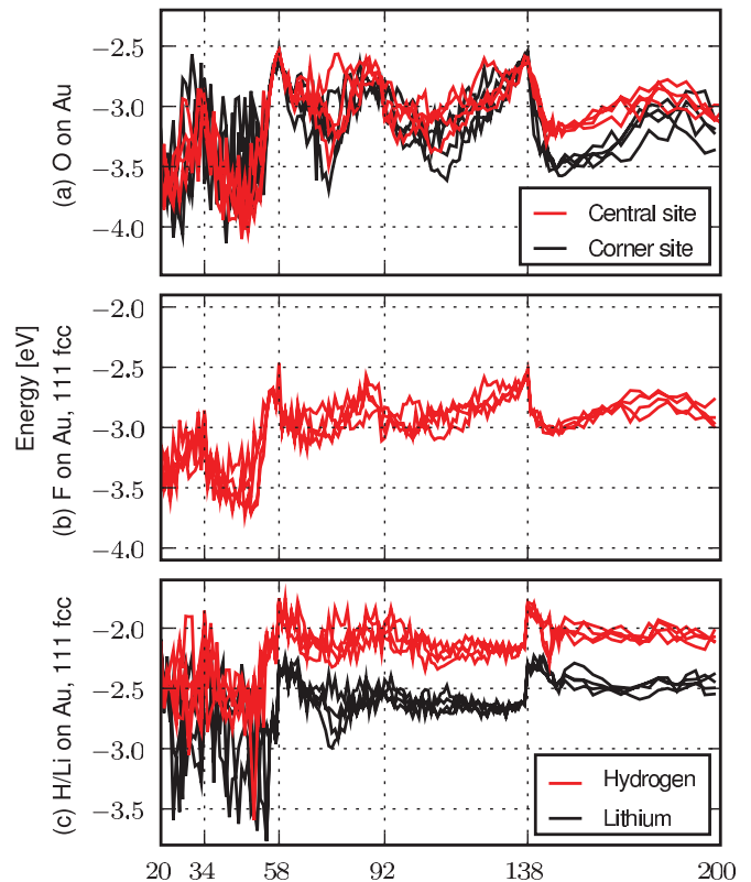
FIG. 12. (Color online) Adsorption energies as a function of Au cluster size. (a) O on the fcc site closest to the center of an (111) facet and the hcp site at the corner of an (111) facet. (b) F on the central (111) fcc site. (c) H and Li.
