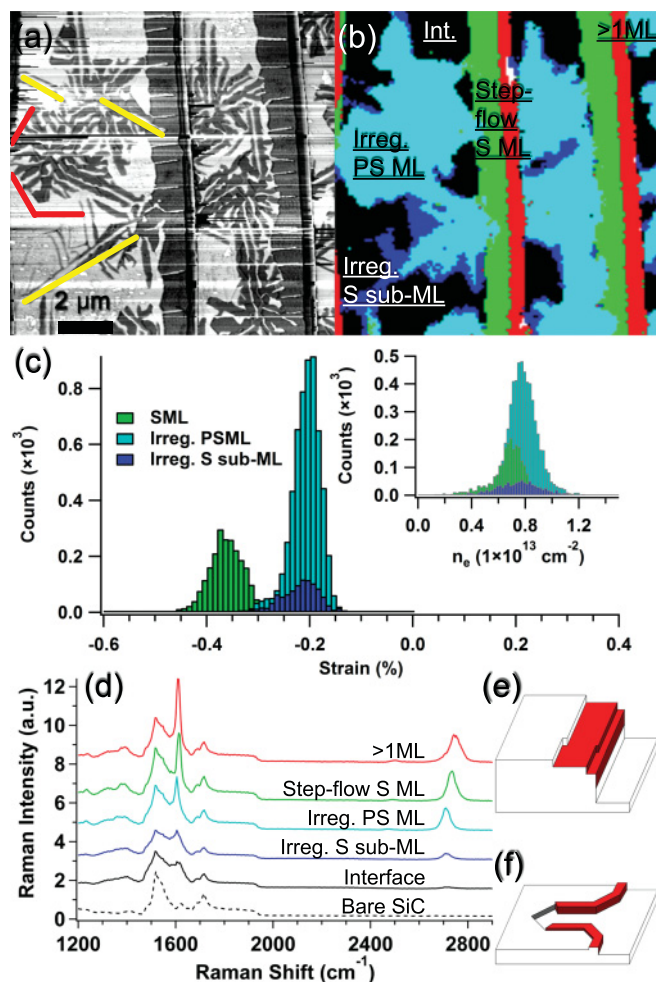
FIG. 3. (Color online) The surface of partially graphitized SiC: (a) AFM phase map; (b) false-color Raman cluster map; (c) strain and carrier concentration (inset) histograms of the clusters shown in (b); (d) average spectra from strain clusters in (b) with bare SiC (dashed curve) for reference, color coding same as (b); and (e-f) schematic of the step-flow and irregular growth mode fronts, respectively. Scan size in (a) and (b) is 12 \times 12 \mu\text{m}^2 . Labels of clusters in (b) correspond to the spectra shown in (d).
