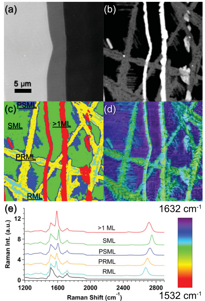
FIG. 1. (Color online) Inhomogeneous Raman spectra in IML epitaxial graphene: (a) AFM topography; (b) Raman G -band intensity map integrated over 1580\text{--}1605\text{ cm}^{-1} ; (c) false-color Raman cluster map; (d) overlay of G -band peak position map (color scale below; blue: shift to higher wave number, yellow: unshifted with respect to \omega_G^0 = 1582\text{ cm}^{-1} ) on AFM phase image shown in gray scale; and (e) average spectra from clusters in (c) with bare SiC (black) for reference, color coding same as in (c). Scan size is 30 \times 30\ \mu\text{m}^2 . Labels in (c) and (e) correspond to each cluster categorized by its strain state. RML stands for relaxed ML (cyan); PRML, partially relaxed ML (yellow); PSML, partially strained ML (blue); SML, strained ML graphene (green); and greater than 1ML coverage (red). Note the lack of any significant defect-induced D band for all clusters.
