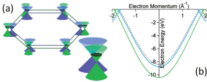
FIG. 5. (Color online) A model accounting for the strain-doping correlation based on v_F renormalization. (a) Schematic illustration of the \pi and \pi^* states (Dirac cone) for 1ML graphene with and without compressive strain. Inner cones (blue) show unstrained, doped 1ML, and outer cones (green) compressively strained, doped 1ML (corresponding to the cases of, for example, RML and SML, respectively). Varying the v_F changes the opening of the cones, thus modifying the carrier concentration for the doped graphene. (b) Tight-binding (TB) band structure for unstrained (inner band, blue) and compressively strained (outer band, green) 1ML for the parameters described in the text. The dash line is the unstrained, undoped case. The electron energy is plotted with respect to the Fermi level.
