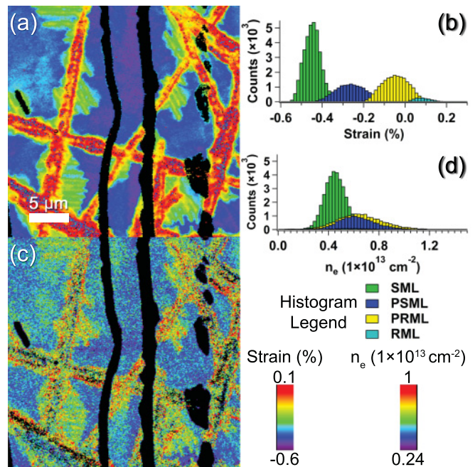
FIG. 2. (Color online) Strain and carrier concentration mapping: (a) mechanical strain-field map; (b) histogram of strain values for (a) categorized by the clusters in Fig. 1(c); (c) electron concentration map; and (d) histogram of electron concentrations for (c) categorized by the clusters in Fig. 1(c). Regions of more than 1ML graphene are not shown [blacked out in (a) and (c)]. Scan size is 30 \times 30 \mu\text{m}^2 . Right bottom: legend for the histogram plots and color-bar scales for strain and carrier concentration.
