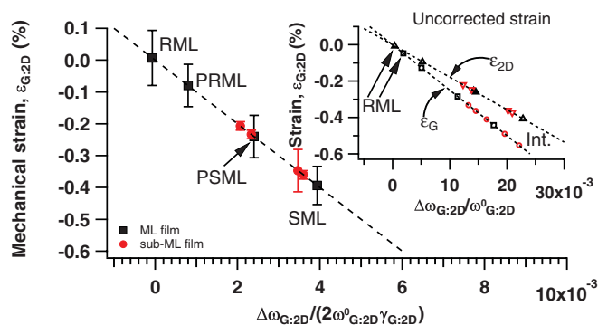
FIG. 4. (Color online) Residual mechanical strain vs normalized relative peak shift as determined from the G - and 2D -band peak shifts for sub-ML (red) and ML coverage (black). Inset: uncorrected strain vs relative peak shift not considering carrier concentration dependence of the Raman peak shift. Circles and squares correspond to G -band positions, and up- down-triangles to 2D -band positions. The interface (Int.) and relaxed monolayer (RML) data points are noted for reference. The dashed lines are linear fits to the data points, with their slopes proportional to the Grüneisen parameters for the G and 2D bands.
