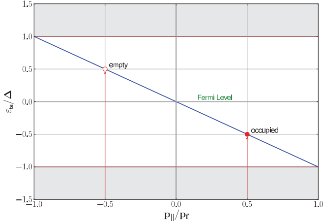
FIG. 2. (Color online) Chiral edge state dispersion, \varepsilon_{bs}(\mathbf{p}) = -c p_{||} , illustrating the asymmetry in the occupation of pairs of time-reversed states.
