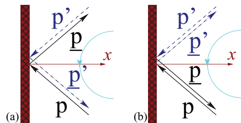
FIG. 3. (Color online) (a) Time-reversed trajectory pairs that define the spectral current density, \mathcal{J}(x, \mathbf{p}; \varepsilon) , for specular reflections. (b) Retroreflections are time-reversed partners for any incident angle. The chirality of the bulk order parameter is indicated by the direction of the arc.
