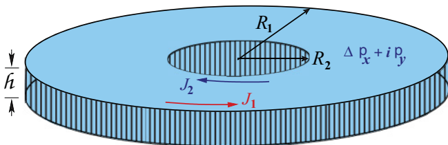
FIG. 9. (Color online) A thin film of chiral p -wave superfluid (“2D ^3\text{He-A} ”) with h \ll \xi , inner and outer radii R_2, R_1 , and area \mathcal{A} = \pi(R_1^2 - R_2^2) bounded by specular surfaces that reflect quasiparticles \mathbf{p} \rightarrow \underline{\mathbf{p}} = \mathbf{p} - 2\hat{\mathbf{x}}(\hat{\mathbf{x}} \cdot \mathbf{p}) . For R_1, R_2, R_1 - R_2 \gg \xi , only single reflections are relevant in determining the surface spectrum and edge currents on the inner and outer boundaries.
