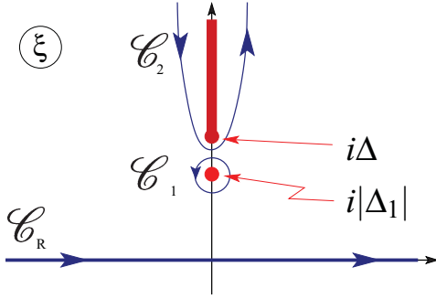
FIG. 5. (Color online) Integration in the complex \xi plane. Integration along the real axis ( \mathcal{C}_R ) is transformed into the sum of an integral around the isolated pole at i|\Delta_1| and the branch cut along the imaginary \xi axis.
