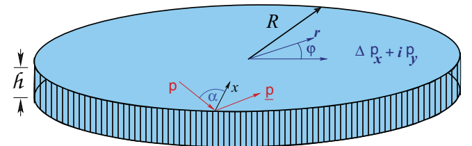
FIG. 1. (Color online) A thin film of p_x + i p_y superfluid (“2D ^3\text{He-A} ”) confined in a cylindrical geometry with thickness h \ll \xi and radius R \gg \xi bounded by specular surfaces that reflect excitations, \mathbf{p} \rightarrow \mathbf{p} .
