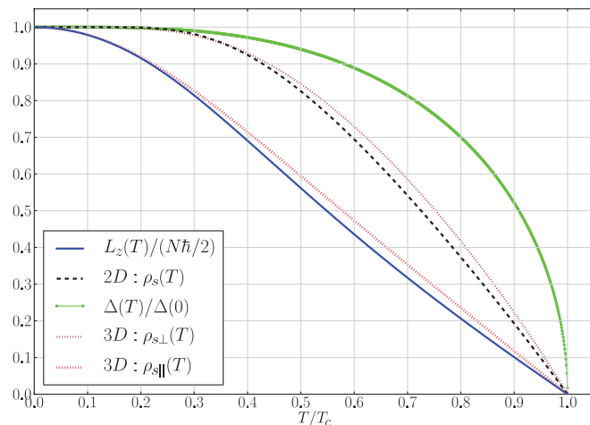
FIG. 6. (Color online) Temperature dependence of the angular momentum, L_z(T) , for the 2D chiral p -wave superfluid (blue line). Also shown is the superfluid stiffness (black dashed line) and the bulk gap (green dots and line) for the fully gapped 2D chiral p -wave state. Shown for comparison are the two components of the superfluid stiffness for the 3D chiral p -wave superfluid phase ( ^3\text{He-A} ): \rho_{s,\parallel} for \mathbf{p}_s \parallel \hat{\mathbf{I}} (red dotted line) and \rho_{s,\perp} for \mathbf{p}_s \perp \hat{\mathbf{I}} (brown dotted line).
