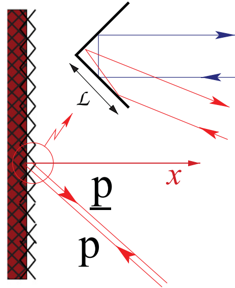
FIG. 8. (Color online) Mesoscopic facets of dimension \hbar/p_f \ll \mathcal{L} \ll \xi are retroreflectors of quasiparticles.
