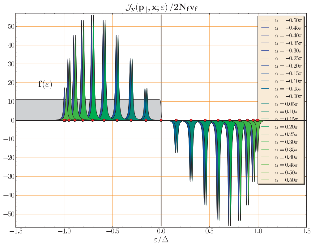
FIG. 4. (Color online) Spectral current density \mathcal{J}_y for x = 0 as a function of p_{\parallel} = p_f \sin \alpha for linewidth \gamma = 0.025\Delta . States with \pm p_{\parallel} are slightly offset to show the contributions to the current from time-reversed pairs.
