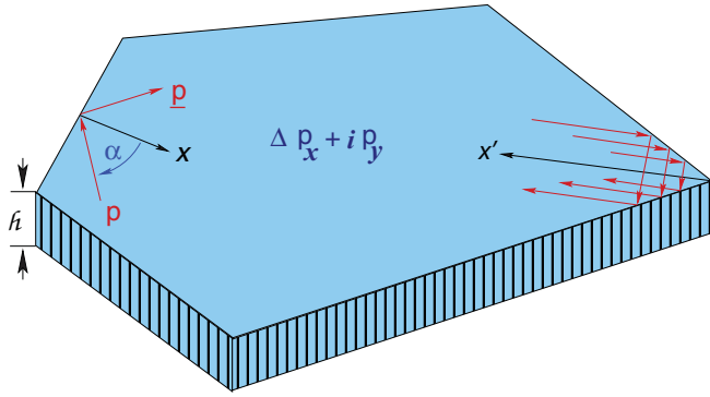
FIG. 7. (Color online) A thin film ( h \ll \xi ) of p_x + ip_y superfluid (“2D ^3\text{He-A} ”) confined in a noncylindrical geometry with area \mathcal{A} \gg \xi^2 bounded in the x - y plane by specular surfaces. Double reflections are important in determining the surface spectrum and edge current near a corner.
