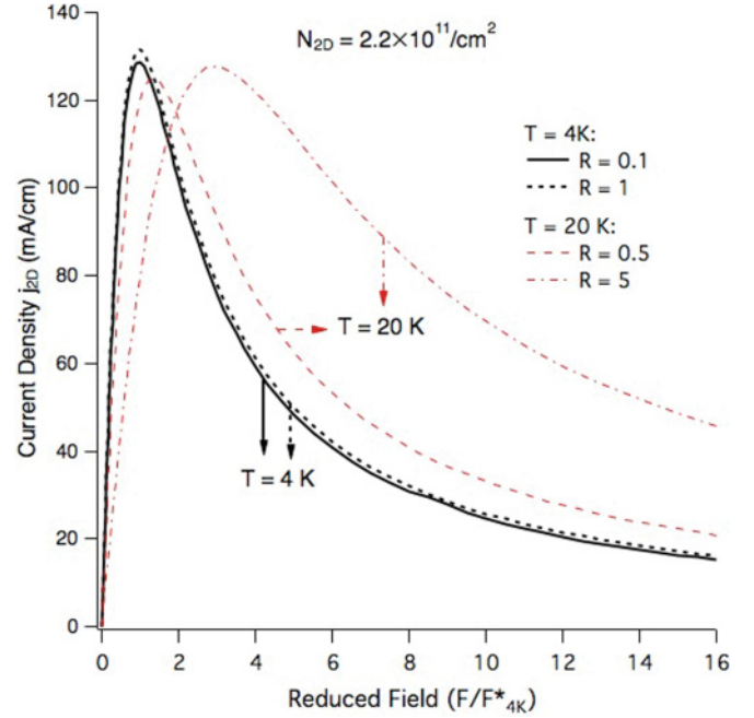
FIG. 2. (Color online) Field dependence of the current at two temperatures: at T = 4\text{ K} for R_{4K} = v_{in}/v_{el} = 0.1 (thick black solid curve), and R_{4K} = 1 (thick black dotted curve) with a fixed total scattering rate; and at T = 20\text{ K} for R_{20K} = 0.5 (thin red dashed curve), and R_{20K} = 5 (thin red dashed-dotted curve), assuming that v_{el} is insensitive to T and v_{in} is linear in T (e.g., R_{20K} = 5R_{4K} ). The current decays as \propto 1/F asymptotically. Other parameters are given in the text.
