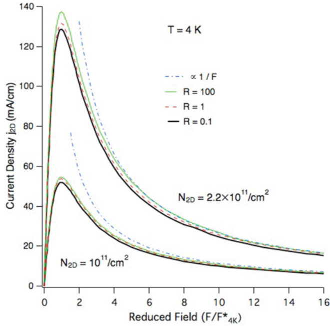
FIG. 1. (Color online) Current density vs reduced field \mathcal{F} = F/F^* for several values of R = v_{in}/v_{el} = 0.1 (thick black solid curve), R = 1 (red dashed curve), and R = 100 (thin green solid curve) for a fixed total scattering rate at 4 K for N_{2D} = 2.2 \times 10^{11}/\text{cm}^2 (upper curves) and N_{2D} = 10^{11}/\text{cm}^2 (lower curves). The scale factor F_{4K}^* can be different for the two densities. The blue dashed-dotted curves show the asymptotic behavior of the current \propto 1/F . Other parameters are given in the text.
