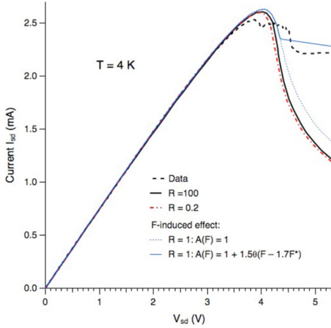
FIG. 3. (Color online) Total current I vs source-drain voltage V_{sd} for R = 0.2 (thick red dashed-dotted curve), R = 100 (thick black solid curve), and the data (thick black dashed curve) at 4 K for N_{2D} = 2.2 \times 10^{11}/\text{cm}^2 . The thin blue dotted and solid curves are plotted for R = 1 and include the effect of field-induced v_{in} for A(F) = 1 and A(F) given in Eq. (29), respectively. Other parameters are given in the text.
