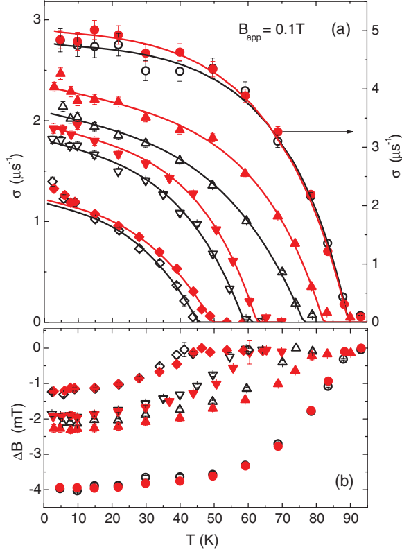
FIG. 3. (Color online) (a) Temperature dependence of \sigma of \text{YBa}_2\text{Cu}_3\text{O}_x measured at B_{\text{app}} = 0.1 T at zero and applied hydrostatic pressures for x = 6.45 ( \diamond , P = 0 GPa; \blacklozenge , P = 1.1 GPa), x = 6.6 ( \nabla , P = 0 GPa; \blacktriangledown , P = 1.1 GPa), x = 6.8 ( \triangle , P = 0 GPa; \blacktriangle , P = 1.1 GPa), and x = 6.98 ( \circ , P = 0 GPa; \bullet , P = 1.4 GPa). The data were analyzed with Eq. (1). The solid curves are fits to the data with Eq. (2). (b) Diamagnetic shift of the field \Delta B = B_1 - B_{\text{app}} in the corresponding samples. B_1 is the mean field in the centre of the sample (see text and the appendix).
