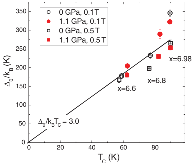
FIG. 6. (Color online) Relation between \Delta_0 and T_c for \text{YBa}_2\text{Cu}_3\text{O}_x with x = 6.6, 6.8, and 6.98 . The solid line corresponds to \Delta_0/k_B T_c = 3 (weak-coupling BSC superconductor: \Delta_0/k_B T_c = 1.76 ). Both \Delta_0 and \Delta_0/k_B T_c increase with increasing pressure.
