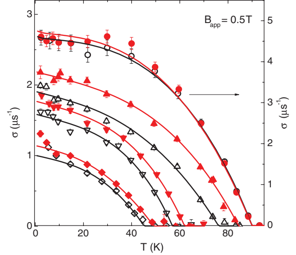
FIG. 4. (Color online) Temperature dependence of \sigma of \text{YBa}_2\text{Cu}_3\text{O}_x measured at B_{\text{app}} = 0.5 T. The meanings of the symbols and the solid lines are the same as in Fig. 3(a).
