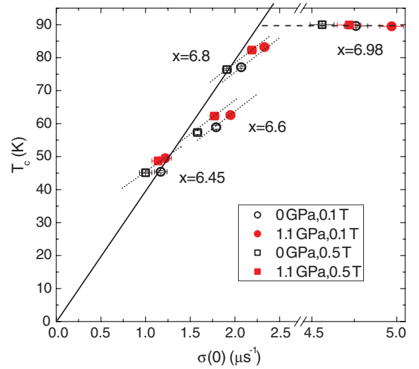
FIG. 5. (Color online) T_c vs \sigma(0) (Uemura plot) at zero and applied pressure for \text{YBa}_2\text{Cu}_3\text{O}_x with x = 6.45, 6.6, 6.8, and 6.98 . The solid line is the Uemura line while the dashed line is a guide to the eye. The dotted lines represent the pressure effects on T_c and \sigma(0) .
