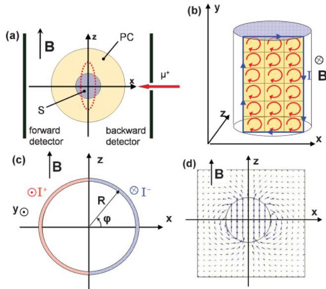
FIG. 8. (Color online) (a) Schematic sketch of the \mu SR pressure instrument GPD at the Paul Scherrer Institute: Cylindrical sample (S), pressure cell (PC), muon stopping distribution (dotted ellipse), and forward and backward positron detectors. (b) Illustration of the surface current on a slice of a homogeneously magnetized cylindrical sample. The magnetic field induced by this slice is equivalent to the magnetic field of the surface currents. (c) Cross section of the cylindrical sample and the surface current distribution in xz plane. (d) Magnetic field map of the surface currents as illustrated in panels (b) and (c).
