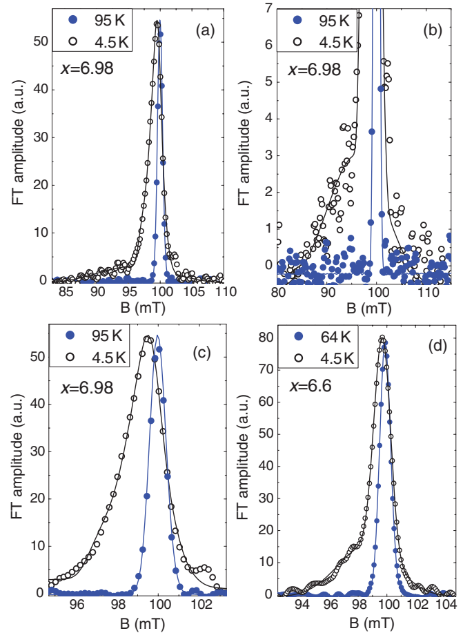
FIG. 2. (Color online) Fourier transform (FT) amplitude as a function of field for the spectra shown in Fig. 1 [panels (a), (b), and (c)]. Panel (b) is the expanded view (along the y axis) of panel (a) showing the signal from the sample. Panel (c) is the expanded view (along the x axis) of panel (a) showing the signal of the pressure cell. Panel (d) shows the FT of the sample with x = 6.6 below and above T_c = 60 K. The solid lines are the FTs of the fitted curves shown in Fig. 1. The FT spectra are slightly broadened due to a FT apodization of 4 \mu\text{s}^{-1} .
