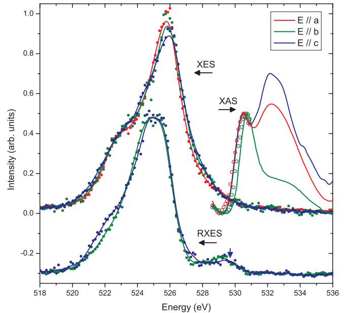
FIG. 5. (Color online) Polarization-dependent above-threshold O K -edge XES spectra of \beta - Sr_{0.17}V_2O_5 recorded with the sample at room temperature, alongside RXES spectra recorded with a photon energy of 529.7 eV (the arrow indicates the location of elastically scattered x-rays). The solid line is a guide to the eye and represents a binomial smoothing of the raw XES data. Also shown are the O K -edge TEY XAS spectra from Fig. 3. For comparison, the leading edge of the TFY data is also displayed by the empty circles. Note that the XAS spectra have been offset by +1 eV with respect to Fig. 3 to account for the core-hole shift (see text).
