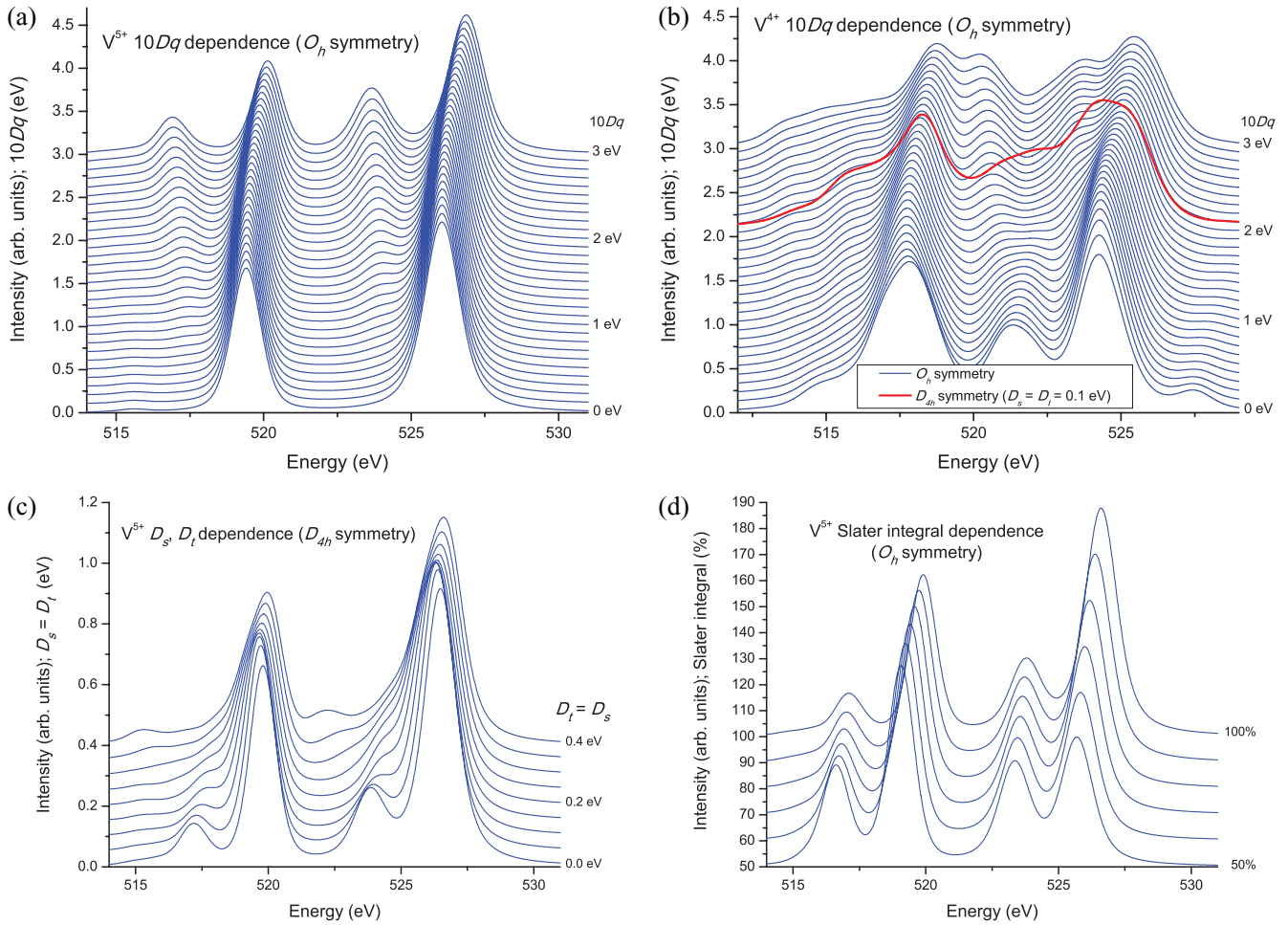
FIG. 3. (Color online) V L_{3,2} -edge atomic multiplet calculations of V^{5+} and V^{4+} in octahedral ( O_h ) and tetragonal ( D_{4h} ) symmetry. (a) The dependence of the calculated spectra of V^{5+} on the crystal field splitting, 10Dq , in O_h symmetry. Spectra are shown vertically offset for clarity. (b) Dependence of the V^{4+} spectra on 10Dq . Also shown in thick red is the V^{4+} spectrum in D_{4h} symmetry for D_t = D_s = 0.1 eV. (c) The dependence of V^{5+} spectra on D_s and D_t ( D_{4h} symmetry). (d) The effect of reducing the magnitude of the Slater integral in O_h symmetry for V^{5+} .
