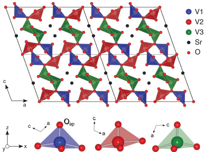
FIG. 1. (Color online) The crystal structure of \beta - \text{Sr}_{0.17}\text{V}_2\text{O}_5 projected along the b crystallographic axis, showing the orientation of the \text{VO}_5 square pyramids. At the bottom, the orientation of each of the \text{V1O}_5 , \text{V2O}_5 , and \text{V3O}_5 pyramids are shown with the vanadyl bond ( \text{V-O}_{\text{ap}} ) aligned with the paper vertical, representing their local quantification axes ( x , y , and z ). The Sr positions are partially occupied.
