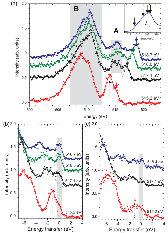
FIG. 6. (Color online) V L_3 -edge RIXS spectra for (a), and (b) E\parallel a , and (c) E\parallel b recorded at the incident photon energies shown on the V L_3 -edge XAS spectrum in the inset to (a). The data are shown on an absolute energy scale in (a), and on a loss energy scale in (b) and (c). The regions marked A and B represent the occupied V 3d states and their hybridization with the O 2p states, respectively. The gray regions in (b) and (c) show the elastically scattered light, and the dotted line at -1.1 eV demonstrates the dd^* excitation feature. In (b) the dotted lines correspond to the data with the elastic peak and V 3d fluorescent contribution removed (see text), demonstrating the presence of the -1.1 eV RIXS peak at other photon energies.
