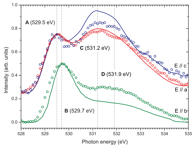
FIG. 4. (Color online) Polarization dependence of O K -edge XAS spectra, recorded in both TEY (solid lines) and TFY (circles) modes.
