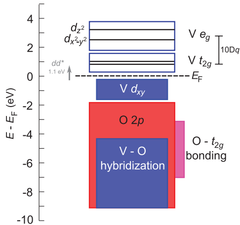
FIG. 7. (Color online) Schematic energy level diagram for \beta - \text{Sr}_{0.17}\text{V}_2\text{O}_5 based on the experimental results. The locations of the occupied states are estimated from the onset of the XES and RIXS spectra. Similarly, the unoccupied states are derived from the O K -edge XAS spectra; the black solid lines represent the peak positions within the approximate bandwidth of the state. Also shown is the dd^* excitation revealed by RIXS measurements.
