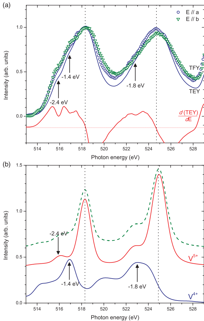
FIG. 2. (Color online) (a) V L_{3,2} -edge XAS spectra of \beta - \text{Sr}_{0.17}\text{V}_2\text{O}_5 recorded in TEY (solid lines) and TFY (open symbols) modes. To illustrate the isotropy at this edge, the TFY data is shown for light incident parallel to both the a - and b -axes. The first derivative of the TEY data is shown at the bottom of the figure for E\parallel a ; the arrows indicate features associated with local minima. (b) V L_{3,2} -edge atomic multiplet calculations for \text{V}^{5+} and \text{V}^{4+} in a tetragonal ( D_{4h} ) distortion to octahedral symmetry (the parameters of the calculation are 10Dq = 2.1 eV, D_t = D_s = 0.1 eV) using the CTM4XAS program. 33 These spectra have been shifted by -1.4 eV to align with the measured L_3 -edge. The dashed (green) line in (b) shows the linear superposition of the \text{V}^{5+} and \text{V}^{4+} spectra at a ratio of 0.83:0.17 according to the stoichiometry.
