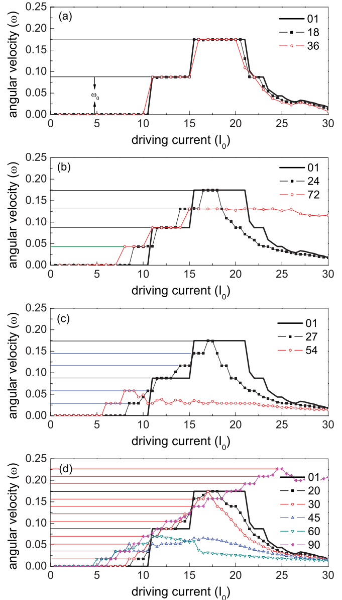
FIG. 7. (Color online) The \omega - I_0 curve for a channel with g = 0.1 and different k : k = 1 (a), 2 (b), 3 (c), and 5 (d). L is the vorticity, i.e., the number of vortices. N is the number of cells in the circular chain. If L/N = 1/m , e.g., L = 1, 36 , the \omega - I_0 curve shows several steps and the height of each integer step is \omega_0 . When L/N = k/m ( k = 2, 3, 5 ), the height of each fractional step is \omega_0/k [e.g., as shown in (b), (c), and (d)].
