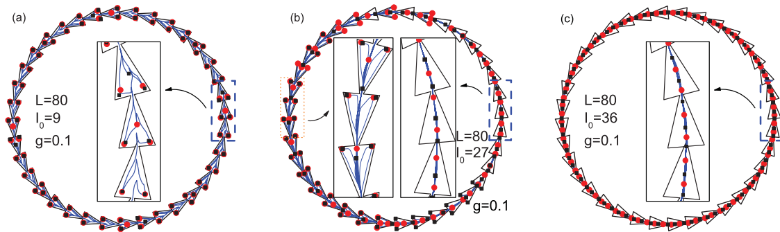
FIG. 5. (Color online) Trajectories of vortex motion during one ac period in the case of high density of vortices ( L = 80 ), i.e., the multivortex regime, for different values of the driving current, I_0 = 9 (a), 27 (b), and 36 (c). When the current is in a certain range I_0 = 5 – 19 [see Fig. 3(c)], the vortices move along a 2D trajectory [e.g., I_0 = 9 , shown in (a)], which is different from the circular 1D trajectories in the low-density case. With increasing current, more vortices start to move along circular trajectories and thus 2D trajectories finally turn to a 1D circle [e.g., see (c)]. During the transition from the 2D to 1D motion, the distribution of vortices becomes inhomogeneous [shown in (b)].
