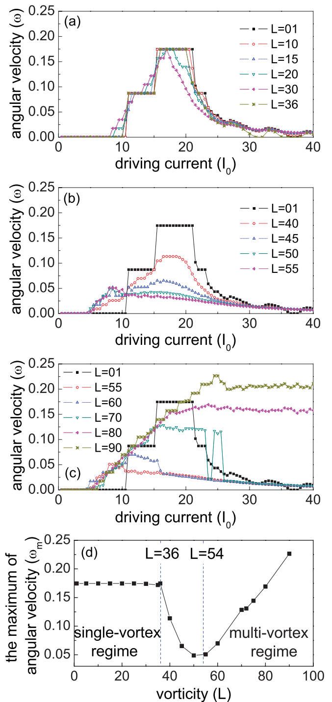
FIG. 3. (Color online) The \omega - I_0 curves for different density of vortices: (a) the density of vortices is low, L = 1-36 (in the single-vortex regime), the angular velocity reaches the same maximum, (b) the density increases, L = 40-55 , the maximum of the angular velocity decreases, (c) for further increasing density, i.e., high density of vortices, L = 55-90 , the maximum starts to increase and the critical value of the driving current, when the angular velocity starts decreasing, becomes larger, (d) the maximum of the angular velocity \omega_m first remains the same until the number of vortices L > 36 . Then the maximum \omega_m first decreases, but for L > 55 , it starts to increase.
