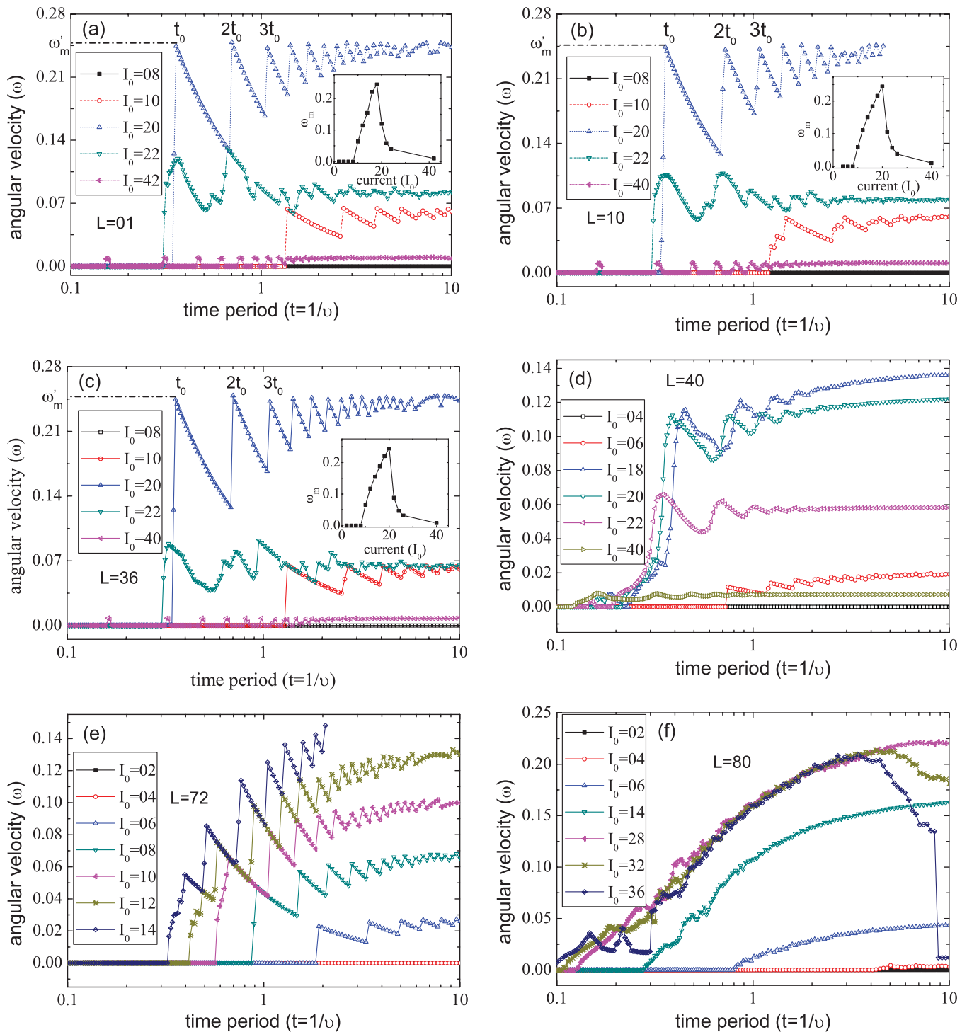
FIG. 10. (Color online) The \omega - t curves in a channel with g = 0.1 for different density of vortices: L/N \ll 1 (a), L/N < 1 (b), L/N = 1 (c) (commensurate), 2 > L/N > 1 (d), L/N = 2 (e) (commensurate), and L/N > 2 (f). When the density L/N \leq 1 , i.e., in the single-vortex regime, the angular velocity \omega(t) first reaches the maximum and then oscillates [see (a), (b), and (c)]. With increasing current, the maximum velocity increases until the driving force reaches a value larger than f_m^- . For high density, the angular velocity \omega(t) does not reach the maximum because the vortex motion in the easy direction is compensated by that in the hard direction. \omega(t) increases when the frequency decreases. In commensurate cases [(c) and (e)], \omega(t) oscillates with sharp jumps, which are not observed in incommensurate cases for high vortex density (f).
