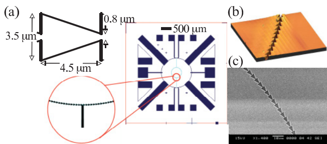
FIG. 12. (Color online) (a) Detail of a single ratchet cell of channel and schematic of a Corbino ratchet chip layout; extra pads and leads beyond disk were not used for the measurements presented here. (b) Atomic force microscopy image of a portion of Corbino ratchet channel. (c) Scanning electron micrograph of a portion of Corbino ratchet channel.
