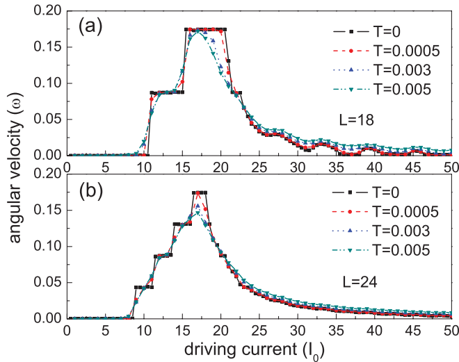
FIG. 9. (Color online) The effect of temperature fluctuations: the \omega - I_0 curves for different temperatures for (a) L = 18 and (b) L = 24 . Both the integer and fractional steps are smeared out, i.e., the commensurability effect is reduced by increasing temperature. When large enough, the thermal fluctuations reduce the ratchet effect, e.g., for L = 24 and T = 5 \times 10^{-3} (b).
