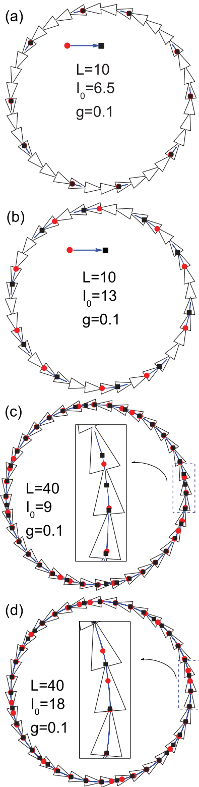
FIG. 4. (Color online) Trajectories of vortex motion, in the case of the low density of vortices ( L = 10 ) (a) and (b), in the intermediate case ( L = 40 ) (c) and (d), for different values of driving current: I_0 = 6.5 (a), 13 (b), 9 (c), and 18 (d). The initial positions of the vortices are marked by the gray circles and the final positions after one period of ac current are marked by the black squares. The trajectories of vortices, which are plotted by solid lines, are nearly circular no matter whether the current is large or small.
