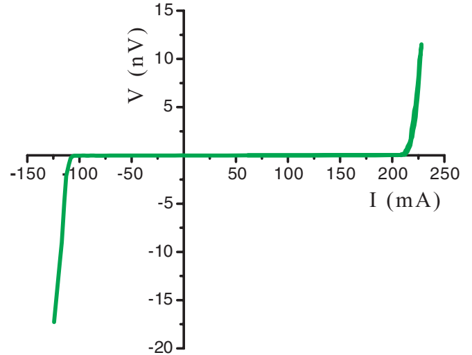
FIG. 13. (Color online) Current-voltage characteristic of a Corbino ratchet channel cooled to 1.60 K in an external magnetic field of 0.26 Oe as described in text.
