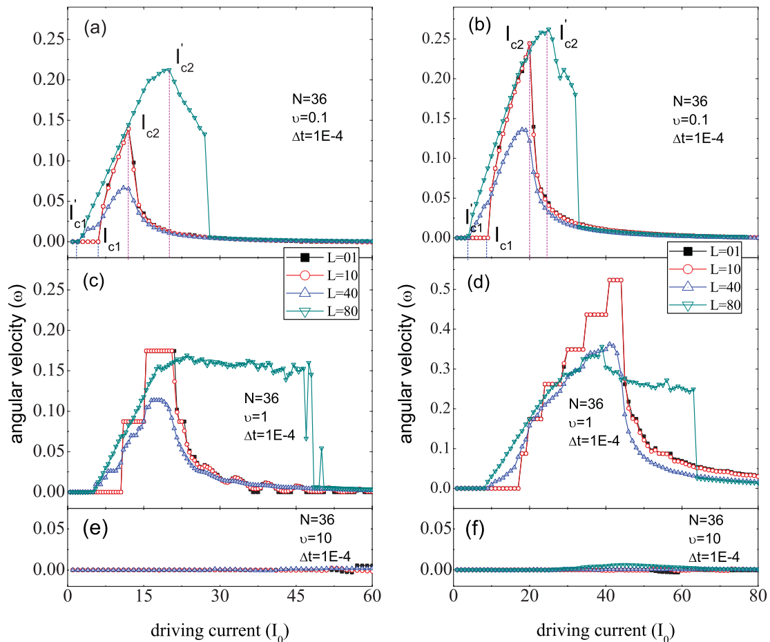
FIG. 6. (Color online) The \omega - I_0 curves for different frequencies: \nu = 0.1 (a) and (b), \nu = 1 (c) and (d), and \nu = 10 (e) and (f). (a), (c), and (e) are in the system with a wider neck, g = 0.1 , and (b), (d), and (f) are in the system with a narrower neck g = 0.05 . The scale of \omega in panel (d) is different from the others. For low-frequency current (e.g., \nu = 0.1 ), the ratchet effect is clearly seen [as shown in (a) and (b)]. In this case, the angular velocity first increases continuously to the maximum and then decreases to zero. For intermediate frequency \nu = 1 , besides the ratchet effect, the effect of commensurability, i.e., discontinuity in the angular velocity \omega(I_0) (see Sec. IV), has a clear influence on the \omega - I_0 curve [e.g., see (c) and (d) for L = 1 or 10 ]. For high-frequency current (e.g., \nu = 10 ), vortices are confined in their initial TCs and only oscillate in a single potential well. Therefore the effect of the periodic ratchet potential disappears [shown in (e) and (f)].
