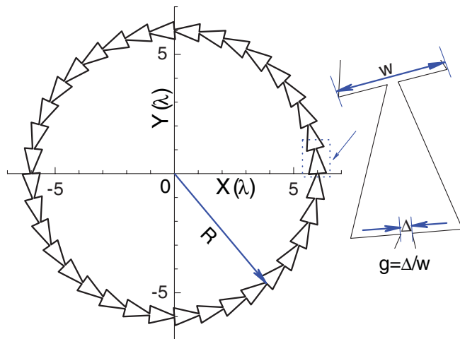
FIG. 1. (Color online) The geometry of the system. The widths of the wide part w and narrow part \Delta are shown in the figure, where g = \Delta/w is the ratio between the two parts. Here, g = 0.1 , the radius of the channel R = 6\lambda , and the channel is constructed by 36 TCs, i.e., N = 36 .
