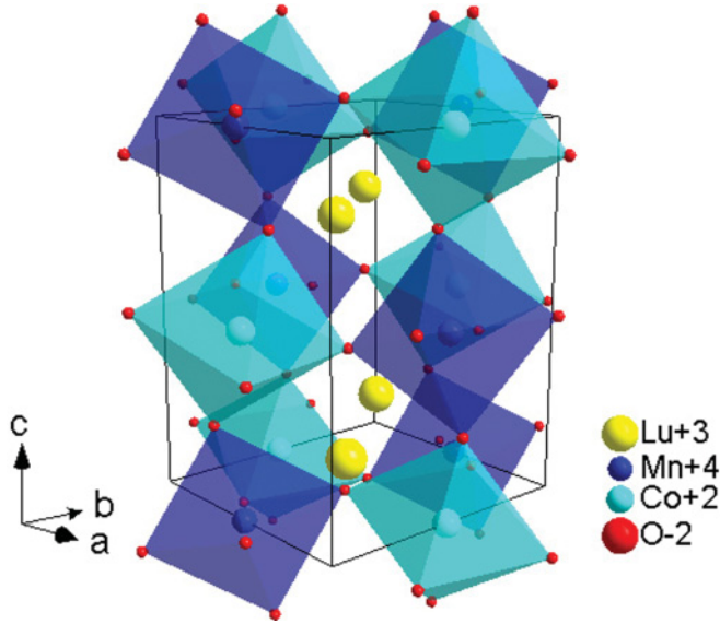
FIG. 2. (Color online) Monoclinic crystal structure of \text{Lu}_2\text{MnCoO}_6 , showing the tilted oxygen octahedra surrounding alternating \text{Mn}^{4+} (dark blue) and \text{Co}^{2+} (light blue) ions. Yellow Lu ions are also shown. Oxygen ions are small red dots at the corners of the octahedra, and Lu ions are the largest yellow balls interstitial between the octahedra.
