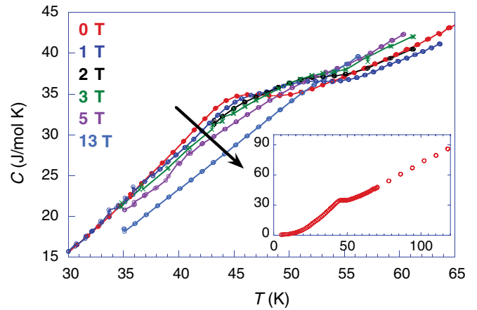
FIG. 5. (Color online) Total specific heat C vs temperature T at various magnetic fields between 0 and 13 T for \text{Lu}_2\text{MnCoO}_6 showing a magnetic-ordering peak that broadens and evolves to higher temperatures in applied magnetic fields.
