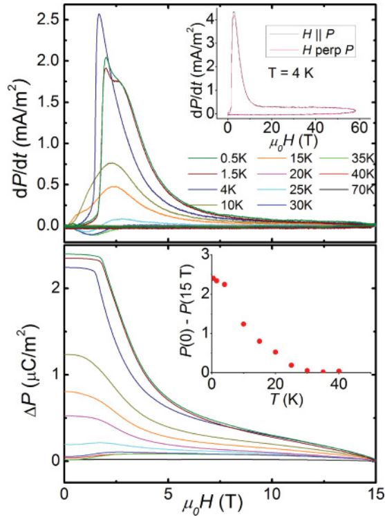
FIG. 8. (Color online) (a) Measured change in electric polarization with time, dP/dt as a function of magnetic field H for various temperature T during a rapid magnetic-field pulse for the geometry P \parallel \vec{H} . Before measuring dP/dt , the sample was poled by applying an electric field of 2 MV/m in zero magnetic field while cooling from 70 K to the intended measuring temperature, at which point the electric field was removed and both sides of the sample were shorted. The inset shows data up to 60 T for \vec{P} parallel and perpendicular to \vec{H} at 4 K, with a 2 MV/m poling voltage. (b) \Delta P(H) determined by integrating the data in (a). The inset shows P(H = 0 \text{ T}) - P(H = 15 \text{ T}) as a function of temperature.
