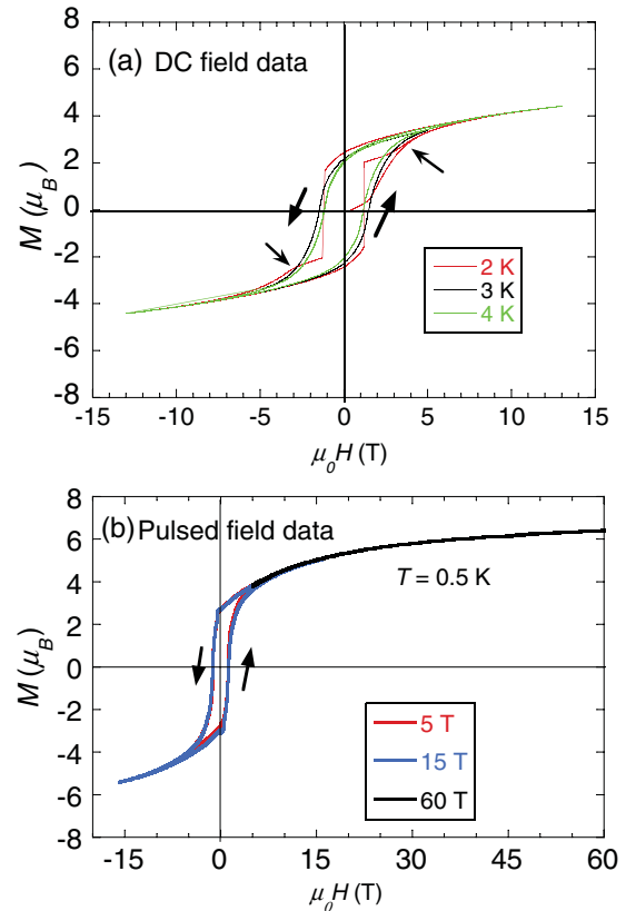
FIG. 7. (Color online) Magnetic hysteresis loops measured in dc magnetic fields (a) and pulsed magnetic fields (b) with maximum pulses of 5, 15, and 60 T (see text). Thick arrows show the direction of the data. A coercive magnetic field of 1.21 T is observed in both data sets, and a magnetic moment of \sim 6 \mu_B is achieved by 0.5 K and 60 T, which would be expected from the combined \text{Mn}^{4+} S = 3/2 and \text{Co}^{2+} S = 3/2 moments (neglecting orbital effects). Thin arrows indicate a slight plateau in the magnetization.
