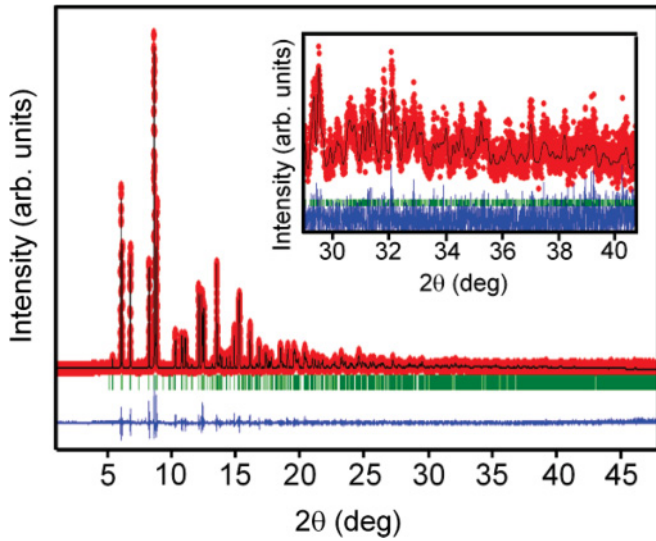
FIG. 3. (Color online) Room-temperature SXRPD patterns of \text{Lu}_2\text{MnCoO}_6 and corresponding Rietveld refinement. Key: Observed (dots), calculated (solid line), and difference (at the bottom) profiles. The tick marks indicate the positions of the allowed Bragg reflections.
