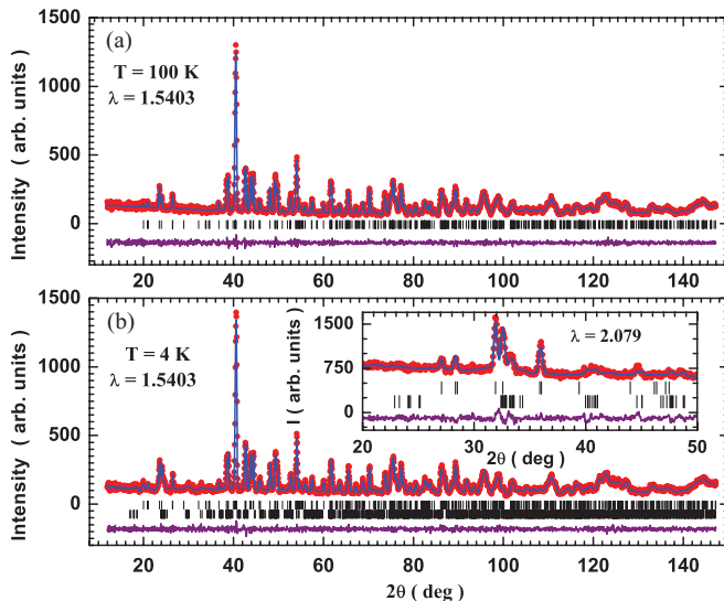
FIG. 4. (Color online) Elastic neutron-diffraction data for polycrystalline \text{Lu}_2\text{MnCoO}_6 at 100 K (a) and 4 K (b). The main panels show data taken with \lambda = 1.540 Å neutrons, while the inset to Fig. 4(b) shows data taken with \lambda = 2.079 Å neutrons. Red circles are experimental data, and the blue lines are fits to the data from Rietveld refinements. Ticks underneath the data indicate symmetry-allowed Bragg positions, and purple lines beneath the ticks show the differences between the data and fits.
