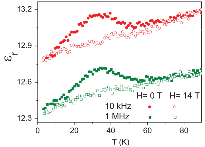
FIG. 9. (Color online) Influence of an external magnetic field ( \mu_0 H = 14 \text{ T} ) on the temperature dependence of the dielectric constant \epsilon_r(T) , measured at frequencies of 10 kHz and 1 MHz.
