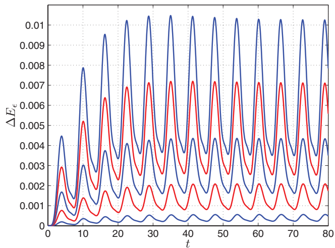
FIG. 2. (Color online) Relative energy \Delta E_\epsilon(t) of the perturbed DW for five different values of the hard-axis anisotropy constant K_2 . See text for discussion.
