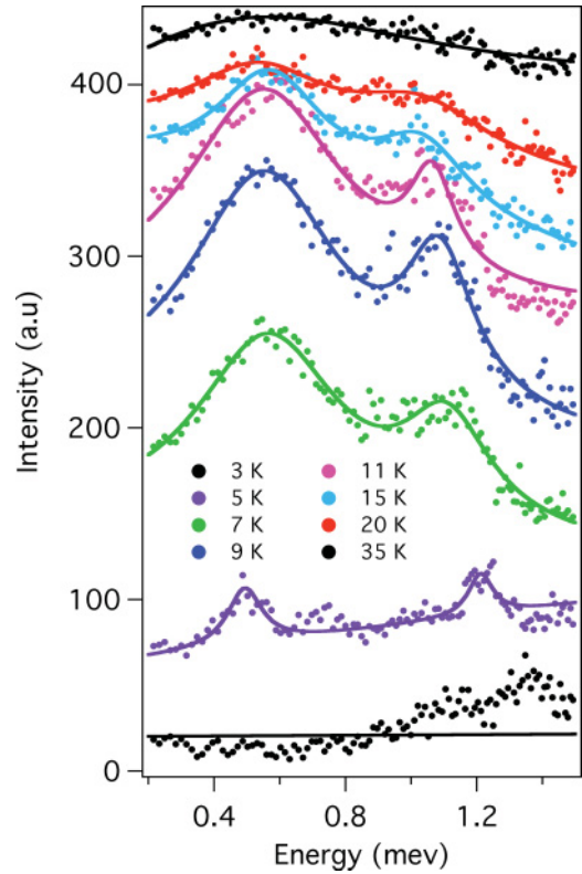
FIG. 8. (Color online) The results of the inelastic neutron scattering experiment using the low-energy configuration of IN5 for a range of temperatures. The data are presented in the form of constant Q = 1.3 \pm 0.1 \text{ \AA}^{-1} and have been corrected for the effects of temperature using Eq. (3). The lines show the results of fitting Lorentzian functions and a sloping background.
