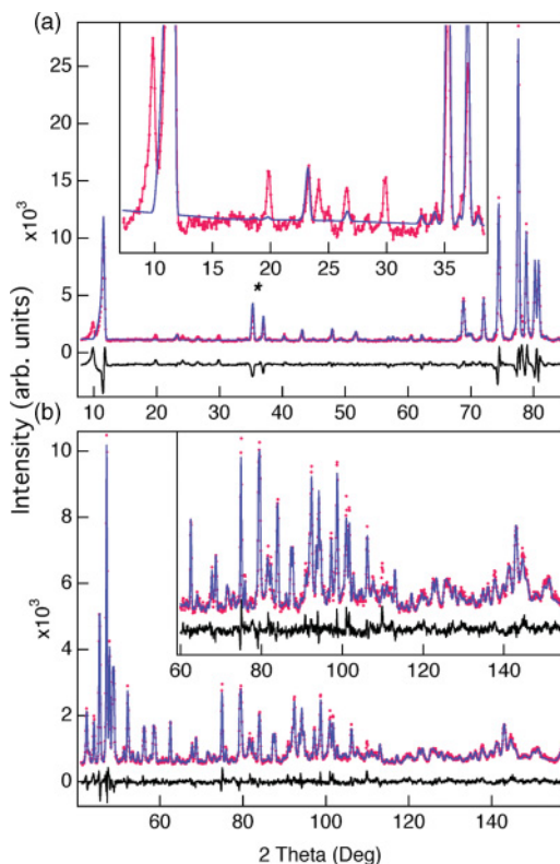
FIG. 4. (Color online) Observed, calculated, and difference plots for Rietveld fit to (a) 2.8 Å and (b) 1.79 Å neutron powder diffraction profiles of \text{CoV}_2\text{O}_6 at 2 K. Insets show unindexed magnetic satellite reflections and fit to high-angle data, respectively. The star in (a) marks the magnetic reflections followed to determine the order parameter using E6.
