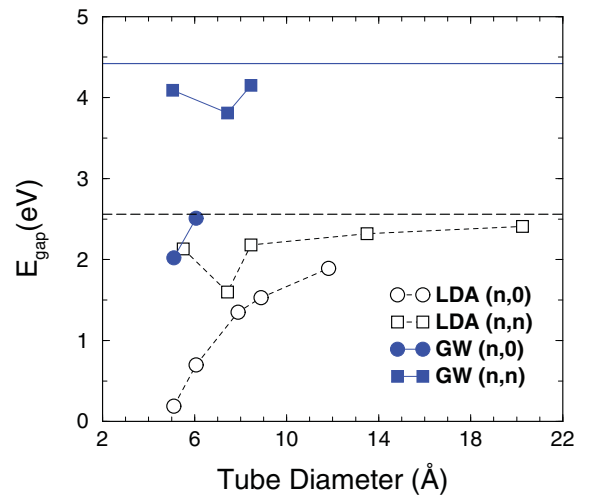
FIG. 4. (Color online) Fundamental band gaps of some zigzag ( n,0 ) and armchair ( n,n ) SiC nanotubes as a function of the tube diameter from the GW (filled symbols) and LDA 17 (open symbols) calculations. The band gap of the isolated SiC sheet obtained from the GW and LDA calculations is also displayed as the solid and the dashed line, respectively. Dotted lines between the symbols are a guide for the eye only.
