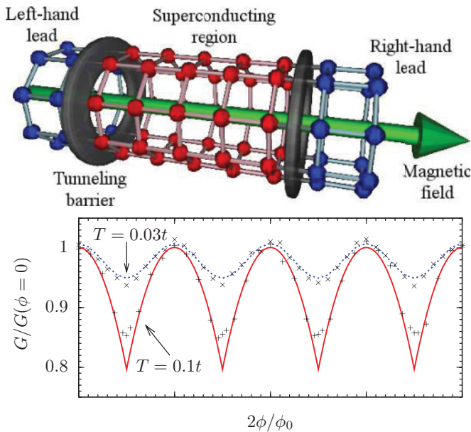
FIG. 7. (Color online) Upper: Schematic of the cylindrical wire within the negative- U Hubbard model. The left- and right-hand metallic leads are shown in blue, from which electrons can tunnel through the gray toroids into the central SC region, which is shown in red. The magnetic flux threading the cylinder is shown as a green arrow. Lower: Variation of conductivity with flux. The computational points are (+) for T = 0.1t , where the data reasonably fit the mean-field Little-Parks model (red solid line), and (x) for T = 0.03t , well below the mean-field transition temperature T_c \simeq 0.09t , where the numerics is best fit by the sinusoidal blue dashed line.
