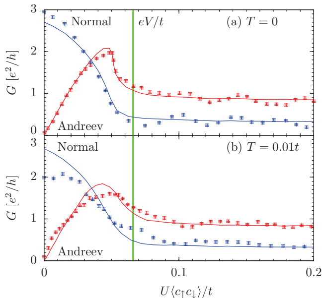
FIG. 2. (Color online) Variation of conductance G with the average superconducting order parameter U\langle c_{\uparrow}c_{\downarrow} \rangle as the interaction strength is increased. The normal current is shown in blue and the supercurrent (Andreev) in red. The numerical results are shown with error bars, and BTK theory by the solid line. The green vertical line denotes the chemical potential difference across the sample. The upper plot (a) is at “zero” temperature, with no thermal or quantum fluctuations, and the lower (b) at T = 0.01t , showing a marked difference between the mean-field BTK formula and the numerical data that include thermal fluctuations.
