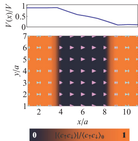
FIG. 9. (Color online) The upper panels in each figure show the potential difference V(x) across the sample with total potential drop V . The lower panels show current maps for (a) short and (b) long normal intermediate regions. Supercurrent is shown by cyan darts and normal current by violet pointers; the arrow length corresponds to current magnitude and orientation to the direction of current flow. Color density corresponds to the order parameter U \langle c_{\uparrow} c_{\downarrow} \rangle_0 , which has peak value U \langle c_{\uparrow} c_{\downarrow} \rangle_0 .
