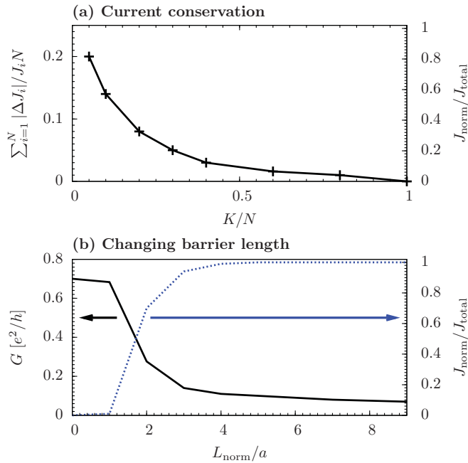
FIG. 8. (Color online) (a) Average fractional error in conservation of current \sum_{i=1}^N |\Delta J_i|/J_i N on each site against the fraction of total states K/N included in the calculation of the current. (b) The changing conductance (black line with arrow toward left) of a Josephson junction with width L_{\text{norm}} of central normal region (left axis), and the fraction of the normal current J_{\text{norm}}/J_{\text{total}} (blue dashed line with arrow toward right) flowing through the central region (right axis).
