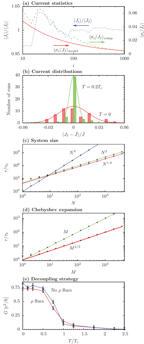
FIG. 11. (Color online) (a) Estimate of the current with number of Monte Carlo iterations, i , out of a total number I = 1000 . The primary y axis shows the best estimate of the current (blue). The secondary y axis shows the estimated standard deviation in this estimate (green) and idealized improvement in the accuracy (red). (b) Distribution of 50 separate current estimates at T = 0 (red) and T = 0.2T_c (green) with best-fit Gaussian distributions. (c) and (d) Time \tau to perform a run on a 32 \times 32 system renormalized by the time \tau_0 for a M = 512 , N = 1 system. In (c) the change with varying the system size N , where the blue line is for the standard O(N^4) method of finding all of the energy eigenvalues, the green is the O(N^2) standard Chebyshev expansion method, 47 and the blue is the O(N^{1.9}) extended Chebyshev approach. In (d) the two Chebyshev expansion method approaches are compared by varying the expansion order M ; the upper (green) line is the standard O(M) approach, 47 and the lower (red) line is the new O(M^{2/3}) algorithm. In (e) we compare the conductivity at the superconductor-insulator transition studied in Fig. 10 with and without density fluctuations.
