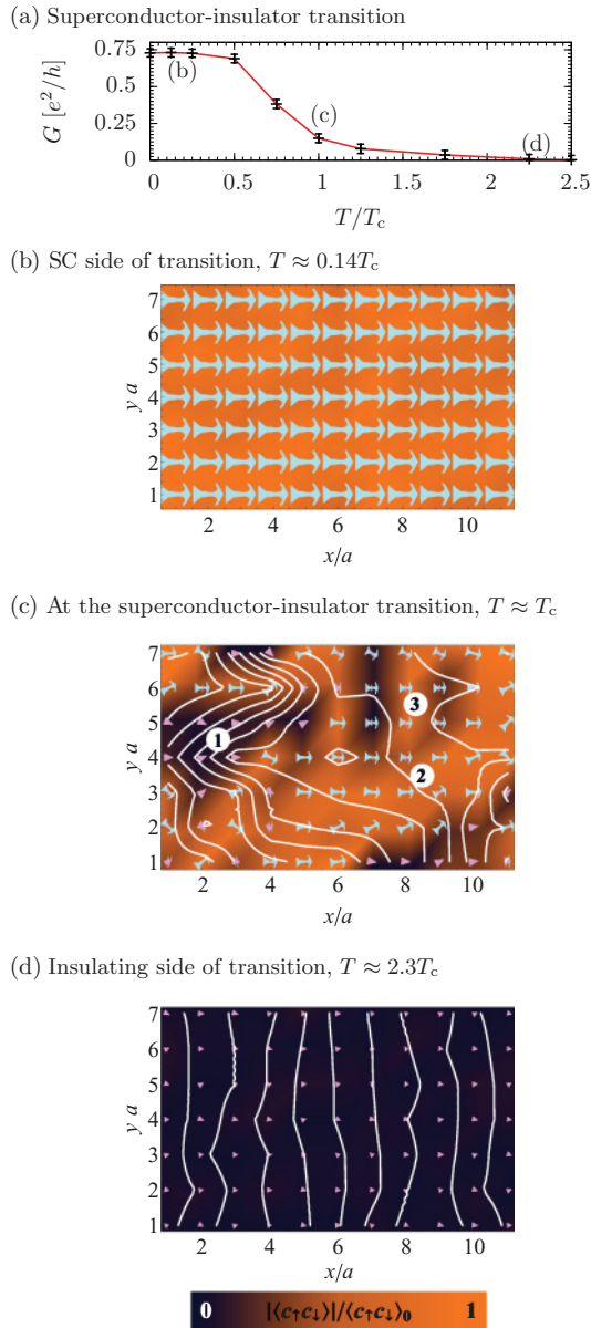
FIG. 10. (Color online) (a) The fall in conductance across the superconductor-insulator transition. Current maps on tuning temperature from (b) a superconductor at T \approx 0.14T_c through to (d) an insulator at T \approx 2.3T_c . At T \approx T_c the superconductor-insulator transition takes place. Supercurrent is shown by cyan darts and normal current by violet pointers, arrow length corresponds to current magnitude and orientation to the direction of current flow. Color density corresponds to the order parameter U \langle c_\uparrow c_\downarrow \rangle . Lines of equal chemical potential are shown in white. In the current map (b) three points of interest are labeled: (1) the normal state, (2) the superconductor state, and (3) Josephson tunneling.
