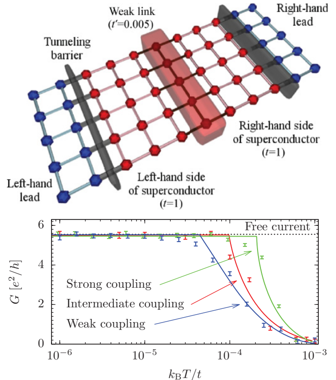
FIG. 3. (Color online) Upper: Setup to model the Josephson junction. Traversing the center of the SC region is a Josephson junction (opaque cuboid). The junction is modeled by the reduction of the matrix hopping elements to t' = 0.005 (brown interconnects) compared to t = 1 in the superconductor. The two metallic leads are shown on the far left and right (in blue), and the lead-superconductor tunneling barrier by the gray cuboids. Lower: The variation of conductance with temperature for the Josephson junction. Results of the numerical computation (points) and of the theoretical model (solid lines) are shown for a weak, intermediate, and strong coupling between the two superconductors.
