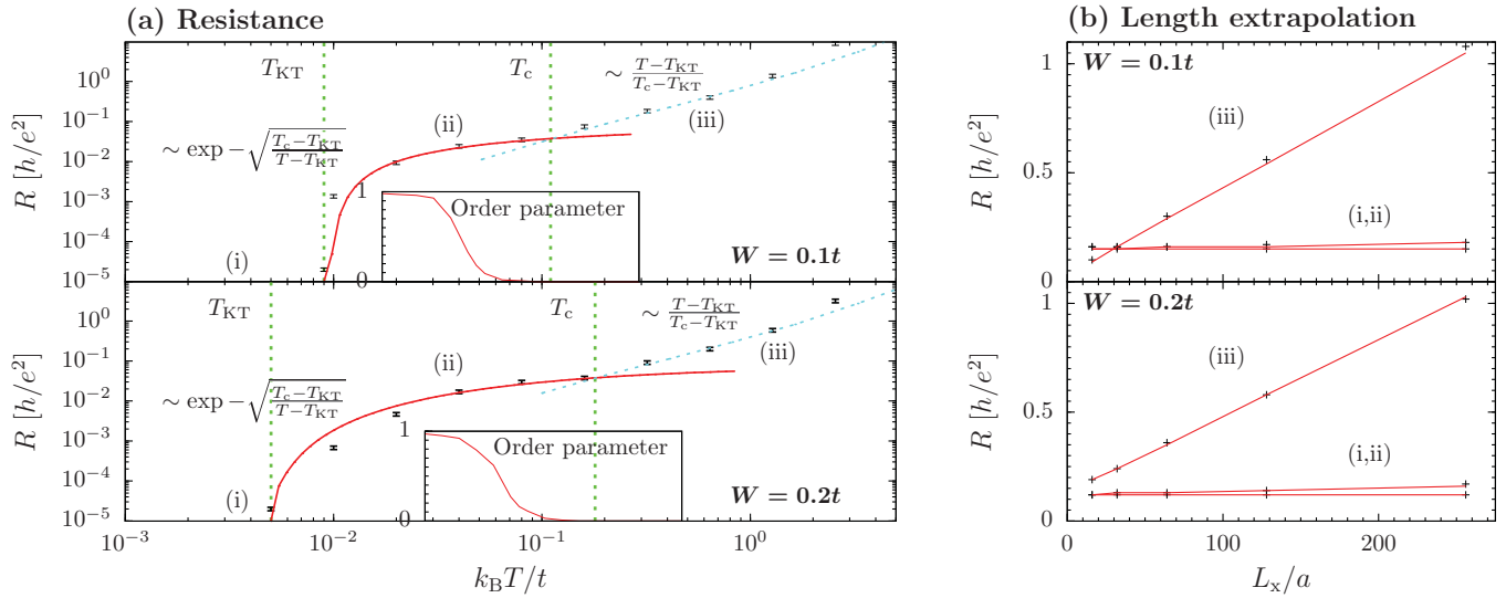
FIG. 6. (Color online) (a) Variation of resistance with temperature for two different values of disorder calculated numerically (points). The red solid line shows the theoretical low-temperature behavior, and the blue dotted line the theoretical high-temperature behavior. The dashed vertical green lines show the BKT T_{KT} and mean-field T_c temperatures. The insets show the variation of the superconducting order parameter U \langle c_\uparrow c_\downarrow \rangle renormalized by its T = 0 value. (b) Numerical results (black points) and the deduced linear length dependence (red solid line) of the resistance for three different temperatures (i) T < T_{KT} , (ii) T_{KT} < T < T_c , and (iii) T > T_c . The L \rightarrow 0 values correspond to the contact resistance, which is eliminated in the values plotted in (a).
