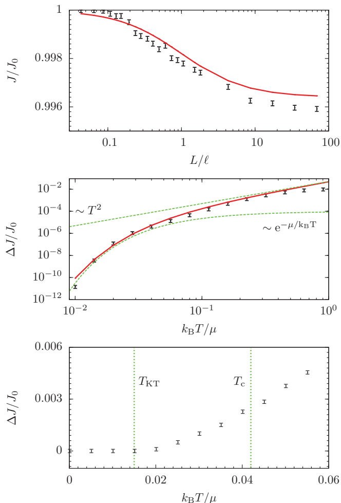
FIG. 4. (Color online) Upper: Relative fall in current in a one-dimensional sample due to the introduction of self-energy at k_B T = 0.1\mu . The black points show the numerical results, and the solid red line highlights the expected theoretical variation with length, 37 where J_0 is the current that flows when impeded solely by the contact resistance. Middle: Relative change ( \Delta J \equiv J_0 - J ) in current as a function of temperature in a one-dimensional normal phase sample. The black points show the numerical results, and the red solid line the expected model variation. The two green dashed lines show the \exp(-\mu/k_B T) and T^2 behavior. Lower: Changing current in the presence of a SC phase in a two-dimensional sample. The vertical green dashed lines show the BKT and normal phase transitions.
