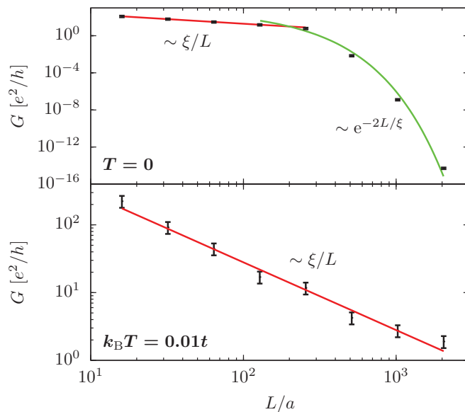
FIG. 5. (Color online) Fall in conductance with length in a noninteracting one-dimensional wire with disorder W = 0.2t at two different temperatures. The straight (red) trend lines show a linear drop off in conductance with length, and the curved (green) an exponential decay.
