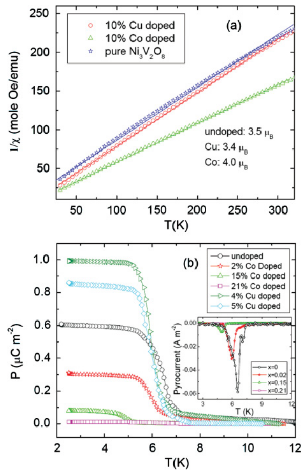
FIG. 2. (Color online) (a) Inverse magnetic susceptibility plotted as a function of temperature for pure \text{Ni}_3\text{V}_2\text{O}_8 and Co- and Cu-substituted \text{Ni}_3\text{V}_2\text{O}_8 to 10 at%. (b) Ferroelectric polarization measured for pure \text{Ni}_3\text{V}_2\text{O}_8 and Cu- and Co-substituted \text{Ni}_3\text{V}_2\text{O}_8 . Inset: Pyroelectric current for pure and Co-substituted \text{Ni}_3\text{V}_2\text{O}_8 .
