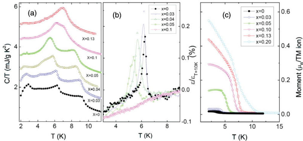
FIG. 4. (Color online) (a) Heat capacity measurements for several Cu-substituted \text{Ni}_3\text{V}_2\text{O}_8 samples, as indicated. The curves have been vertically offset for clarity. (b) Dielectric constant measured as a function of temperature for different compositions of Cu-substituted \text{Ni}_3\text{V}_2\text{O}_8 . The values plotted are scaled to those measured at T = 10 K. (c) Magnetization measured as a function of temperature for several Cu-substituted \text{Ni}_3\text{V}_2\text{O}_8 samples.
