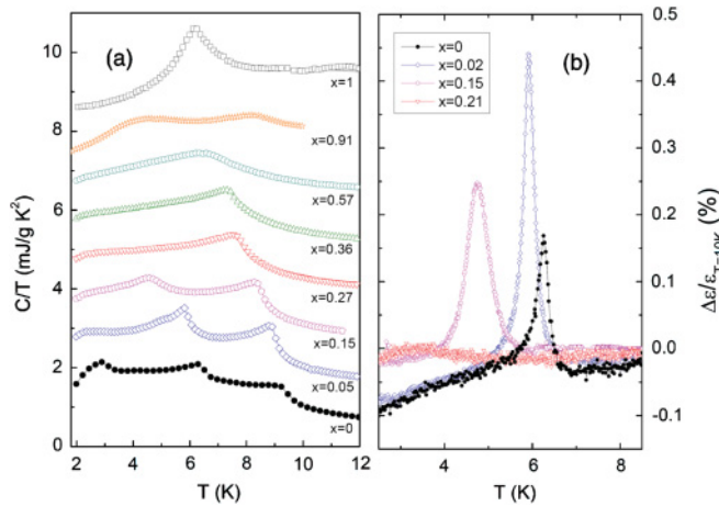
FIG. 3. (Color online) (a) Heat capacity measurements for several Co-substituted \text{Ni}_3\text{V}_2\text{O}_8 samples, as indicated. The curves have been vertically offset for clarity. (b) Dielectric constant measured as a function of temperature for different compositions of Co-substituted \text{Ni}_3\text{V}_2\text{O}_8 . The values plotted are scaled to those measured at T = 10 K.
