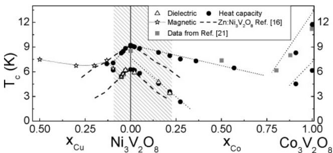
FIG. 5. (Color online) Composite phase diagram for Cu- and Co-substituted \text{Ni}_3\text{V}_2\text{O}_8 . The left panel shows the transition temperatures determined from the measurements listed for Cu-substituted \text{Ni}_3\text{V}_2\text{O}_8 . The right panel shows the transition temperature for Co-substituted \text{Ni}_3\text{V}_2\text{O}_8 . The dashed lines indicated the transition temperatures found for \text{Ni}_3\text{V}_2\text{O}_8 substituted with nonmagnetic Zn, and the hashed region indicates the composition range that appears to exhibit coexisting magnetic and ferroelectric order.
