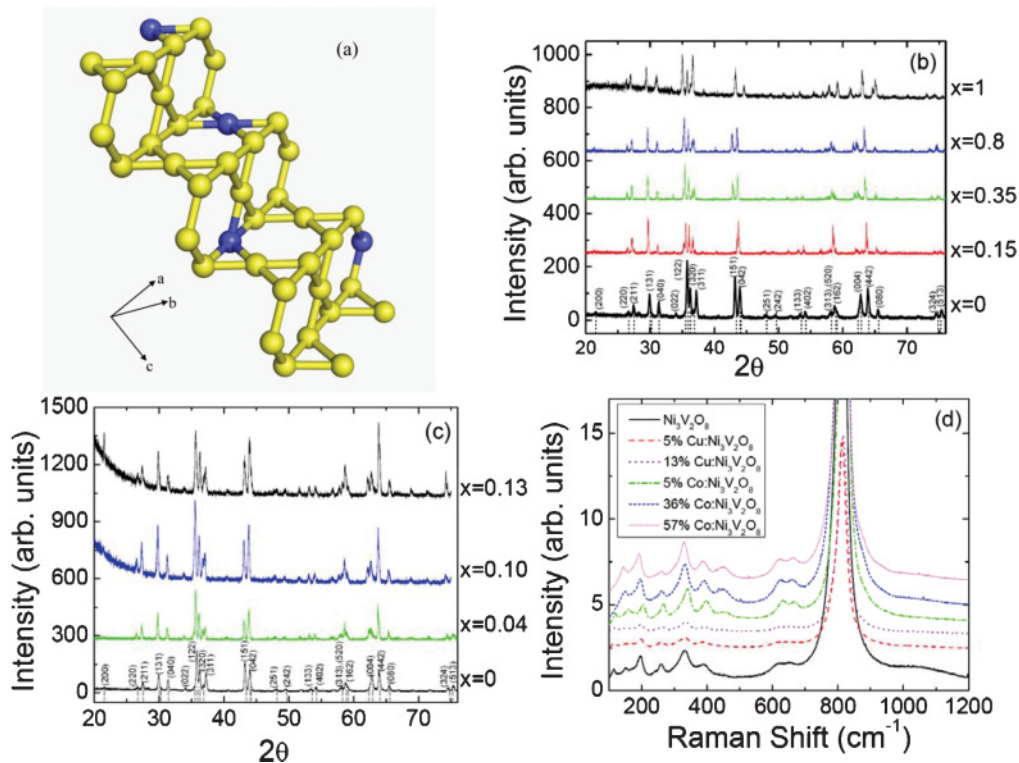
FIG. 1. (Color online) (a) Representation of a single plane of the \text{Ni}^{2+} Kagome lattice with random 10% transition metal doping, (b) XRD spectra for selected Co-substituted \text{Ni}_3\text{V}_2\text{O}_8 samples, (c) XRD spectra for selected Cu-substituted \text{Ni}_3\text{V}_2\text{O}_8 samples, and (d) Raman spectra for pure \text{Ni}_3\text{V}_2\text{O}_8 , and Co and Cu-substituted \text{Ni}_3\text{V}_2\text{O}_8 at different compositions, as indicated.
