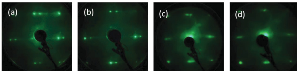
FIG. 1. (Color online) LEED patterns taken at \sim 123 eV at each stage of the FeMn(10ML)/Fe(2ML)/Co(20ML)/Cu(1,1,10) sample growth. (a) Cu(1,1,10) substrate, (b) after 20 ML Co growth, (c) after 2 ML Fe growth, and (d) after 10 ML FeMn growth.
