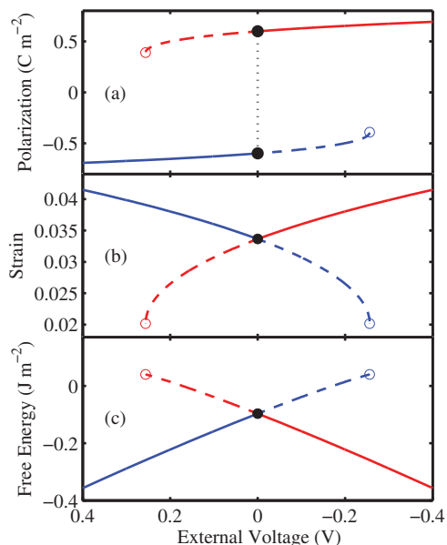
FIG. 4. (Color online) Equilibrium solutions for (a) polarization P , (b) strain x_3 , and (c) Gibbs free energy \mathcal{G} as a function of V_{\text{ex}} , calculated for PbTiO 3 coherently strained to SrTiO 3 at 644 K with t = 3.2 nm and \lambda/t = 10^{-4} . Red (blue) curves are positive (negative) polarization; solid (dashed) segments are stable (metastable); closed (open) circles show equilibrium transition (instability) points.
