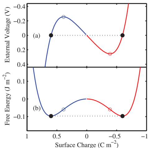
FIG. 8. (Color online) Equilibrium solutions for (a) external voltage V_{\text{ex}} and (b) Helmholtz free energy \mathcal{A} as a function of surface charge \sigma corresponding to Fig. 7. Red (blue) curves are positive (negative) polarization; all values are stable with respect to P variations when \sigma is spatially uniform. Closed (open) circles show the equilibrium transition (instability) points when \sigma can be nonuniform.
