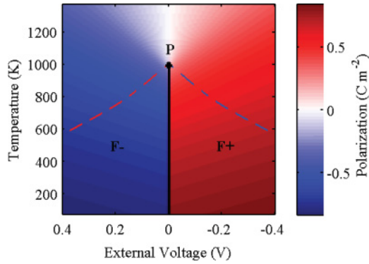
FIG. 5. (Color online) Equilibrium polarization phase diagram as a function of V_{\text{ex}} and T for \text{PbTiO}_3 coherently strained to \text{SrTiO}_3 with t = 3.2 nm and \lambda/t = 10^{-4} . Color scale gives polarization of stable phase. Solid black line is phase boundary between positive and negative polar ferroelectric (F+ and F-) phases, terminating at T_C . Dashed red and blue curves are metastability limits of the F+ and F- phases, respectively.
