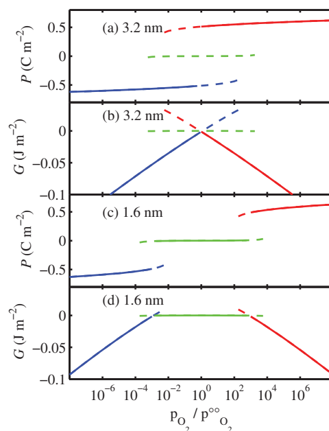
FIG. 16. (Color online) Polarization P and free energy \mathcal{G} of the (meta-)stable equilibrium solutions as a function of p_{O_2}/p_{O_2}^{\circ} . Blue, green, and red curves are for negative, zero, and positive polarization solutions; solid and dashed regions are stable and metastable, respectively. Parameter values used are given in Tables I and II, with T = 644 K, and t = 3.2 nm for plots (a) and (b), t = 1.67 nm for plots (c) and (d).
