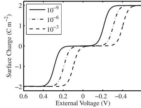
FIG. 12. Surface charge density \sigma as a function of V_{\text{ex}} at three values of p_{O_2} , corresponding to the concentrations shown in Fig. 11. Parameter values used are given in Table II.
