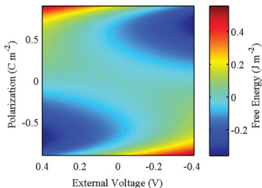
FIG. 3. (Color online) Gibbs free energy \mathcal{G} vs. P and V_{\text{ex}} for a t = 3.2 nm PbTiO 3 film coherently strained to SrTiO 3 at 644 K, with \lambda/t = 10^{-4} . Color scale gives values of \mathcal{G} .
