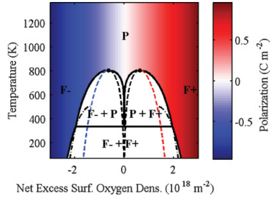
FIG. 20. (Color online) Phase diagram as a function of net excess surface oxygen density \rho_0 and T for 1.6 nm of PbTiO 3 coherently strained to SrTiO 3 , corresponding to Fig. 17(b). Color scale gives polarization in single-phase region; three two-phase regions are marked. Solid and dash-dot black curves are stable and metastable phase boundaries, respectively, between non-polar paraelectric (P) and positive and negative polar ferroelectric (F+ and F-) phases. Dashed red, blue, and black curves are metastability limits of the F+, F-, and P phases, respectively.
