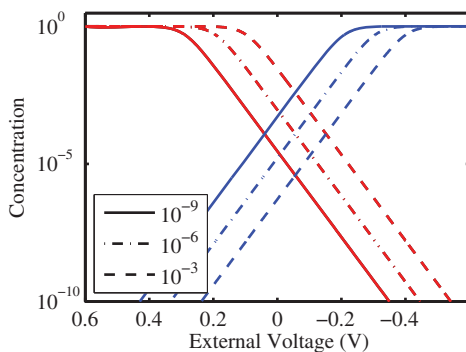
FIG. 11. (Color online) Concentrations of positive \theta_{\oplus} (red curves) and negative \theta_{\ominus} (blue curves) surface ions as a function of V_{\text{ex}} , calculated for the values of p_{O_2} (bar) given in the legend at T = 644 K, t = 3.2 nm. Parameter values used are given in Table II.
