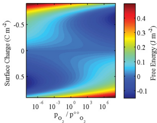
FIG. 14. (Color online) Free energy as a function of \sigma and p_{O_2}/p_{O_2}^{\circ} . Parameter values used are given in Tables I and II, with T = 644 K, t = 3.2 nm. Color scale gives values of \mathcal{G} .
