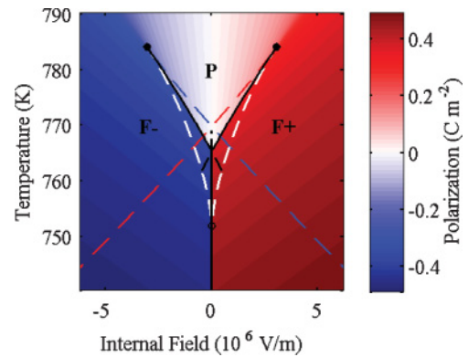
FIG. 23. (Color online) Region near critical points on equilibrium polarization phase diagram as a function of E_{in} and T for unstressed bulk PbTiO_3 with ideal electrodes ( \lambda = 0 ). Color scale gives polarization of stable phase. Solid and dash-dot black curves are stable and metastable phase boundaries, respectively, between nonpolar paraelectric (P) and positive and negative polar ferroelectric (F+ and F-) phases. Dashed red, blue, and white curves are metastability limits of the F+, F-, and P phases, respectively.
