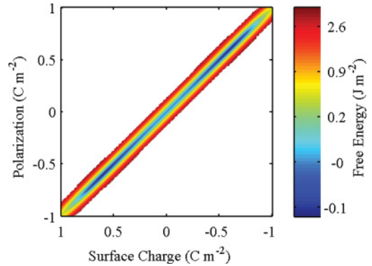
FIG. 7. (Color online) Helmholtz free energy \mathcal{A} vs. polarization P and surface charge \sigma for a t = 3.2 nm \text{PbTiO}_3 film coherently strained to \text{SrTiO}_3 at 644 K, with \lambda/t = 10^{-4} . Color scale gives values of \mathcal{A} . To emphasize the equilibrium solutions, only the region near P = -\sigma is plotted since \mathcal{A} is very large outside this region.
