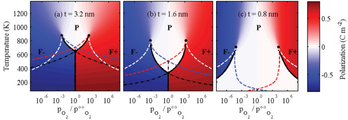
FIG. 17. (Color online) Phase diagrams as a function of p_{O_2}/p_{O_2}^{\infty} and T for three thicknesses of PbTiO_3 coherently strained to SrTiO_3 , using parameters in Tables I and II. Color scale gives polarization. Solid and dash-dot black curves are stable and metastable phase boundaries, respectively, between non-polar paraelectric (P) and positive and negative polar ferroelectric (F+ and F-) phases. Dashed red, blue, and white curves are metastability limits of the F+, F-, and P phases, respectively.
