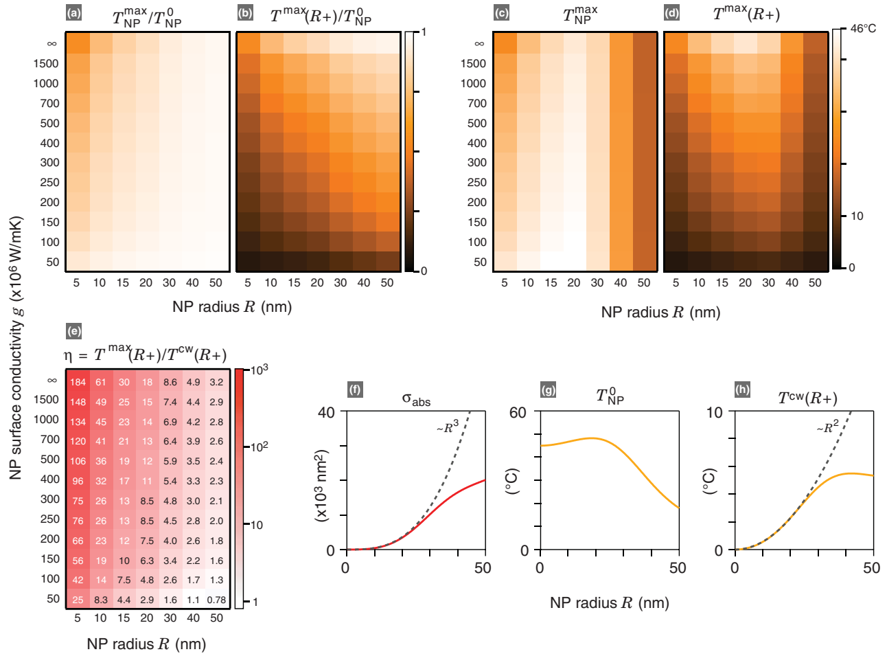
FIG. 7. (Color online) (a) Numerical calculations of the temperature maximum of the NP normalized by the ideal temperature increase T_{\text{NP}}^0 for a set of different NP radii and surface conductivities. (b) Numerical calculations of the temperature maximum achieved in the surrounding medium normalized by the ideal temperature increase T_{\text{NP}}^0 . (c) NP maximum temperature when illuminated by a pulsed laser, at a pulse repetition rate f = 86 MHz and an irradiance I = 0.1 mW/ \mu\text{m}^2 . (d) Maximum temperature of the surrounding medium under the same illumination conditions. (e) Ratio between the maximum temperature on the NP surface achieved under pulsed illumination and the temperature on the NP surface under cw illumination [Eq. (17)]. (f) Absorption cross section of a spherical gold NP as function of radius obtained from Mie theory [Eq. (24)] (solid line). The deviation from the R^3 law is represented by a dashed line. (g) Ideal temperature increase T_{\text{NP}}^0 as function of NP radius. (h) Temperature on the NP surface under cw illumination [calculated from Eq. (17)]. The deviation from the R^2 law [see Eq. (23)] is represented by a dashed line.
