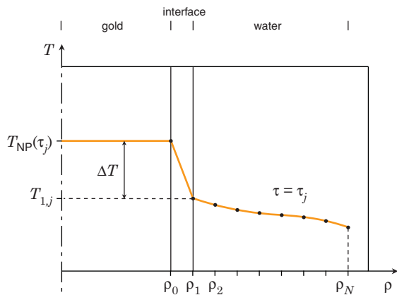
FIG. 9. (Color online) Schematic of the temperature profile at time \tau_j around a spherical gold NP as modeled in the FDM-RK4 algorithm. In this first model, the NP temperature T_{\text{NP}}(\tau_j) is assumed to be uniform and a temperature discontinuity \Delta T occurs at the nanoparticle interface to take into account a finite interface conductivity.
