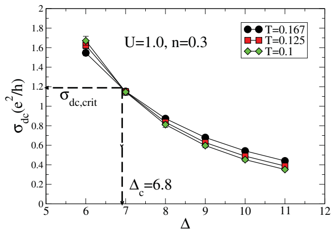
FIG. 4. (Color online) Plot of the critical conductivity \sigma_{dc} vs disorder strength \Delta for three temperatures and the same values of U and n as in Fig. 3. The well-defined crossing point determines the critical disorder strength as \Delta_c = 6.8 . The conductivity at the critical disorder has the value \sigma_{dc,crit} = 1.19e^2/h .
