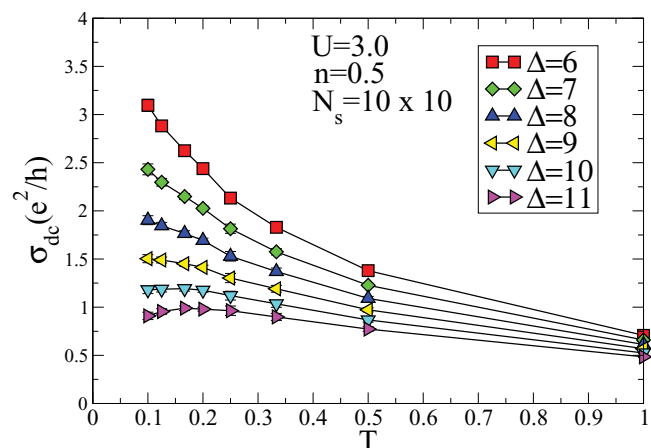
FIG. 1. (Color online) Curves of the dc conductivity vs temperature at electron density n = 0.5 (quarter filling) and interaction U = 3 on a 10 \times 10 square lattice computed for different values of the disorder strength \Delta (see inset).
