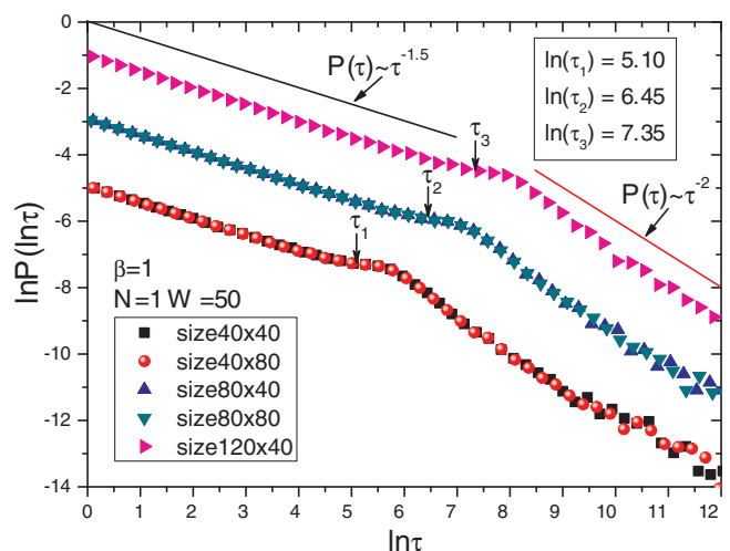
FIG. 5. (Color online) Comparison of \tau_0 for different system sizes at the same disorder strength W = 50 and channel number N = 1 . Black and red curves are downshifted by -2 , and the pink one is upshifted by 2 .
