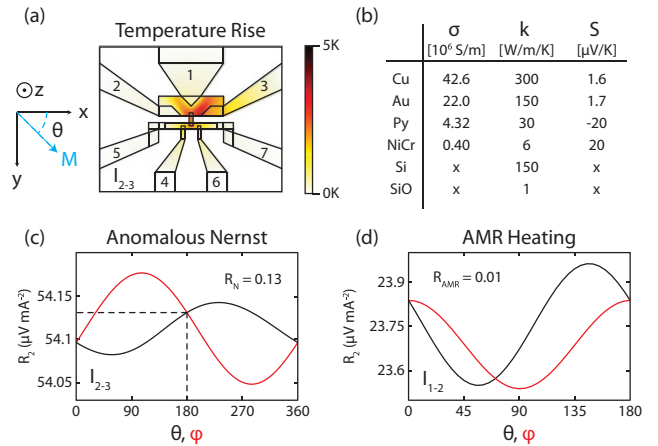
FIG. 5. (Color online) Simulated results of the three-dimensional thermoelectric model. (a) The temperature distribution of the device with a current of 1 mA sent parallel ( I_{2-3} ) to the alignment of the magnetization. (b) Input parameters used for the model. The electrical conductivities \sigma are measured while the others are taken from literature (Refs. 10 and 11). (c) The simulated anomalous Nernst voltage from the thermocouples 4–5 and 6–7 as a function of the magnetization angles \theta on the x - y axis and \phi between the x - y plane and the z axis of \text{FM}_2 . (d) The simulated AMR heating as a function of the magnetization direction of \text{FM}_1 .
