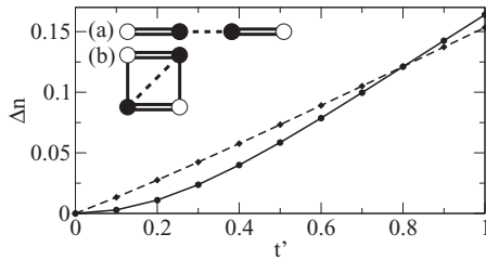
FIG. 1. Charge difference \Delta n between members of the same dimer as a function of the hopping integral t' corresponding to the dotted bonds for the two molecules (a) and (b) given as inserts. Each four-atom molecule contains two electrons. The intradimer double bonds have strength t_1 = 1.5 and the single bonds in (b) are t_2 = 0.5 . The results shown are for U = 4 and V = 0 . Solid (dashed) curves show \Delta n for the linear (square) molecules. Lines are guides to the eye. Filled and empty circles of the molecules correspond to sites with charge densities 0.5 + \Delta n/2 and 0.5 - \Delta n/2 , respectively.
