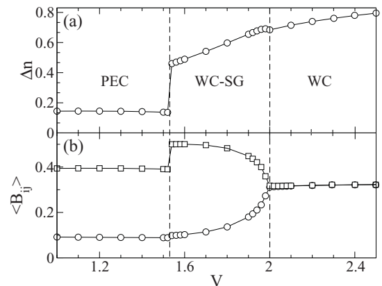
FIG. 5. Variation of order parameters with V = V_x = V_y ( V' = 0 ) for U = 6 , t' = 0.8 , \alpha = 1.1 , K_\alpha = K_\beta = 2 , \beta = 0.1 . (a) Charge disproportionation \Delta n and (b) bond orders along two successive t' bonds. In PEC region, these correspond to bonds between sites with “1–1” (squares) and “1–0” (circles) occupancy. In the WC-SG and WC regions, both bonds are between “1–1” sites. Lines are guides to the eye.
