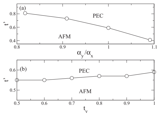
FIG. 7. Phase diagram variation on hopping and electron-phonon interaction anisotropy. In both (a) and (b) U = 6 , V_x = V_y = 1 , V' = 0 , \beta = 0.1 , and K_\alpha = K_\beta = 2 . In (a) t_x = t_y = 1 and \alpha_x = 1.1 , but \alpha_y is varied. In (b) t_x = 1 and t_y is varied, with identical \alpha_x = \alpha_y = 1.1 . Lines are guides to the eye.
