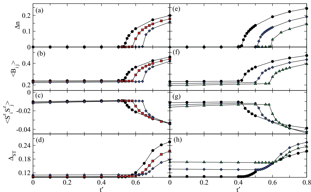
FIG. 3. (Color online) Order parameters for the 4 \times 4 lattice versus t' . Parameters are \alpha = 1.1, \beta = 0.1 , and K_\alpha = K_\beta = 2 . Circles, squares, diamonds, and triangles are for U = 2, 3, 4 , and 6 , respectively. V_x = V_y = V' = 0 for (a)–(d), and V_x = V_y = 1 and V' = 0 for (e)–(h). (a) and (e) show the charge disproportionation \Delta n , (b) and (f) the bond order B_{i,j} between charge-rich sites i and j connected by t' [see Fig. 2(c)], (c) and (g) spin-spin correlations between these sites, and (d) and (h) the singlet-triplet gap \Delta_{ST} . In all cases the CO pattern is as shown in Fig. 2(c). For all plots lines are guides to the eye.
