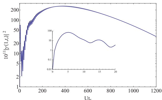
FIG. 11. (Color online) The inset shows that \gamma(1, t_r) goes to zero at early times since there is no mechanism to hop at small times. On a longer time scale, we see the development of an exponential decay. The small magnitude of the correlation is due to fact that the UHB is largely k independent.
