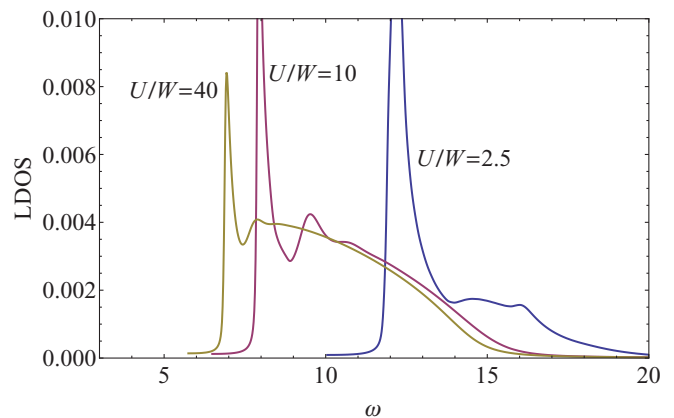
FIG. 2. (Color online) High-frequency (UHB) density of states in two dimensions, n = 1/20 . As the hopping is decreased from t = \frac{1}{2}, \frac{1}{8}, \frac{1}{32} at a fixed U = 10 , the UHB consists of a sharp peak and a broad k -independent background that maintains a width of O(U) . The sharp k -dependent peak does narrow as the hopping decreases. In Fig. 3, the broad UHB of the full band can be seen with the G_1 from Eq. (3) superimposed. Here, the UHB feature is broadened by \eta and the LHB is suppressed for clarity.
