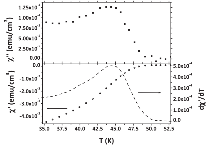
FIG. 2. Temperature dependence of the real and imaginary components of ac susceptibility \chi' and \chi'' (bottom and top panels, respectively). The alternating field amplitude H_{ac} = 1.5 \times 10^{-4} T at the frequency \nu_m = 37 Hz is superimposed to a larger static field H = 1.5 T. The dashed line in the bottom panel represents the first derivative of \chi' with respect to temperature.
