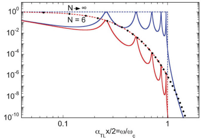
FIG. 5. (Color online) Case of a coupling through a transmission line. Spectrum of the thermal noise power density x^2/\sinh^2 x (black dots), the spectral transmission factor \mathcal{T}_M(x) (dotted blue line), and of the photonic heat (thin red full line) as a function of the frequency for values of the parameter \gamma = 0.01, 0.1, \text{ and } 1 . The frequency is plotted in units of the cut-off frequency \omega_c . We consider a temperature T so that \alpha_{TL} = 0.2 and the case of perfect resistance matching R_1 = R_2 with R = 0.1\sqrt{L/C} .
