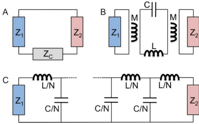
FIG. 1. (Color online) Top left panel circuit A: two impedances Z_1 and Z_2 are coupled by a purely reactive coupling impedance Z_c . Top right panel circuit B: two impedances Z_1 and Z_2 are coupled via mutual inductances to a purely reactive central circuit of total impedance Z_c (here an LC resonator). Bottom panel circuit C: two impedances Z_1 and Z_2 are coupled via a transmission line.
