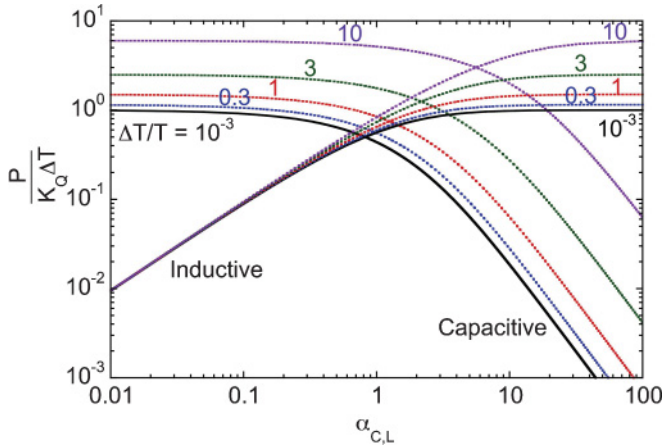
FIG. 6. (Color online) Dependence of the photonic power through a capacitive or inductive coupling impedance on the parameters \alpha_C or \alpha_L for different values of the relative temperature difference \Delta T/T in units of K_Q \Delta T , the maximum photonic power in the case of a linear response.
