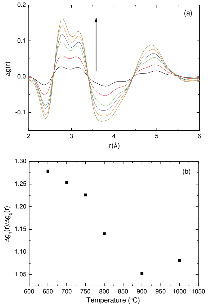
FIG. 4. (Color online) (a) The differences in the pair distribution functions \Delta g(r) = g_T(r) - g_{1100^\circ\text{C}}(r) for \text{Cu}_{46}\text{Zr}_{54} at T = 1000, 900, 800, 750, 700, and 650^\circ\text{C} , showing a splitting of the first peak that becomes more distinct as the temperature is reduced. The curve with the lowest magnitude at the first peak corresponds to the highest temperature ( T = 1000^\circ\text{C} ), and the arrow indicates the increasing magnitude of \Delta g(r) with supercooling. (b) The ratio of the heights of the two distinct components of the first peak in \Delta g(r) , with supercooling (error bars are smaller than the symbols), showing a rapid increase near 850 °C (1123 K).
