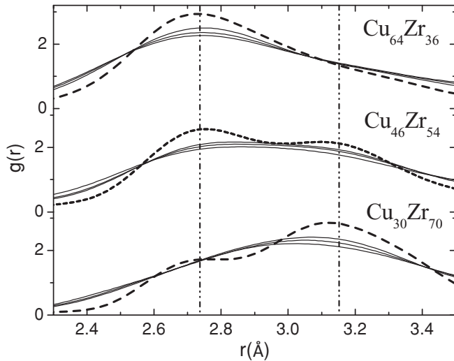
FIG. 3. The first peak in g(r) for \text{Cu}_{(100-x)}\text{Zr}_x liquids for (top) x=36 at 777, 927, and 1127 °C, (middle) x=54 at 650, 900, and 1100 °C, and (bottom) x=70 at 777, 1027, and 1327 °C; in all cases the lowest magnitude corresponds to the highest temperature. For each composition, the dashed curve is the g(r) obtained from the rapidly quenched glass. The vertical lines indicate the positions of the partial pair separation distances at room temperature, taken from EXAFS and neutron-scattering data (Refs. 34 and 35) and MD simulations (Ref. 36).
