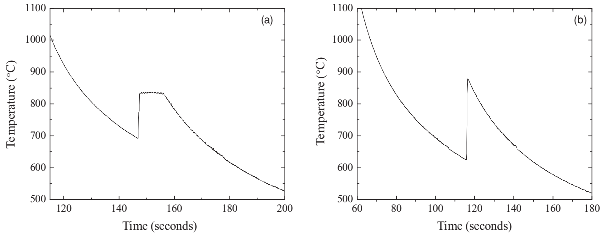
FIG. 1. Temperature measured as a function of time for \text{Cu}_{(100-x)}\text{Zr}_x liquids during free cooling for (a) x=36 and (b) x=54 . Note the different scales on the time (abscissa) axes; the temperature (ordinate) axes are of the same scale.
