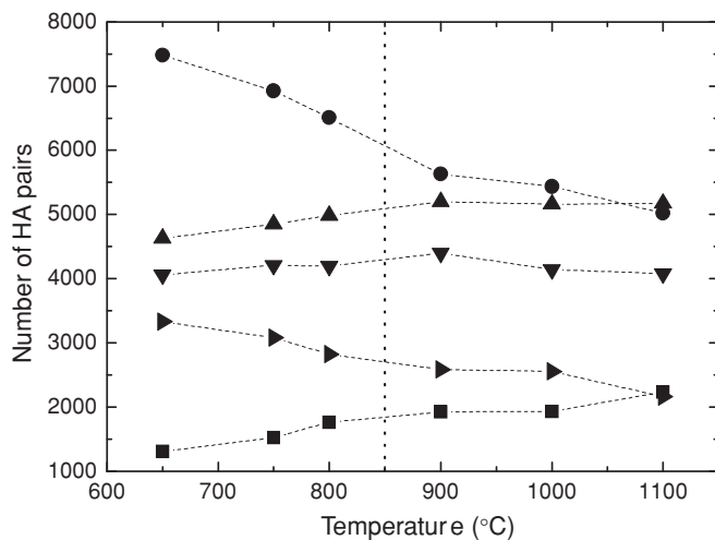
FIG. 6. The numbers of HA pairs with various local symmetries for \text{Cu}_{46}\text{Zr}_{54} liquids as a function of temperature; the ICOS (1551 ●) is the dominant order, and both it and the DICOS (1431 ▲, 1541 ▼) show sharp changes near the transition temperature at 850 °C (dashed vertical line), while hcp-fcc (1421-1422 ■) and bcc (1661 ►) change more gradually.
