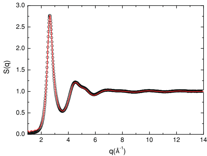
FIG. 5. (Color online) An example of the quality of the RMC fits to the measured S(q) data for supercooled liquid \text{Cu}_{46}\text{Zr}_{54} ; the data at 650 °C are shown by the solid circles and the fit is indicated by the red line.
