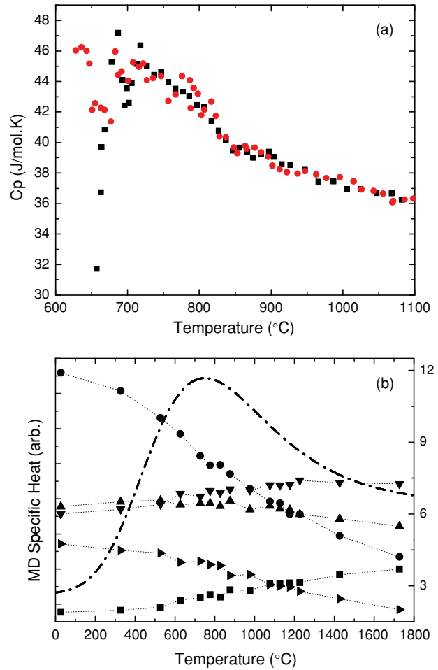
FIG. 7. (Color online) (a) The specific heat for liquid \text{Cu}_{46}\text{Zr}_{54} as a function of temperature [ C_p(T) ] for two cooling cycles [symbols: red filled circle (●) and ■]. The scatter between the two data sets reflects the experimental uncertainty; (b) The C_p(T) of a \text{Cu}_{50}\text{Zr}_{50} liquid and glass calculated from an MD simulation using an embedded atom potential (dash-dot line), and the results of an HA index analysis of the resulting MD configurations (ICOS (1551 ●), DICOS (1431 ▲, 1541 ▼), HCP/FCC (1421/1422 ■) and BCC (1661 ►)).
