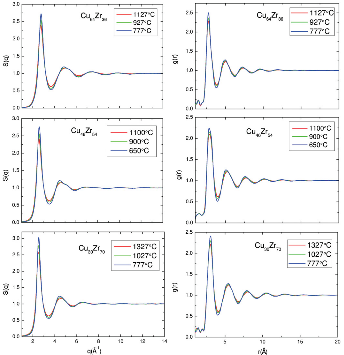
FIG. 2. (Color online) Total static structure factors (left-hand side) and pair distribution functions (right-hand side), with changing temperature, for \text{Cu}_{100-x}\text{Zr}_x liquids with x=36 (top), 54 (middle), and 70 (bottom).
