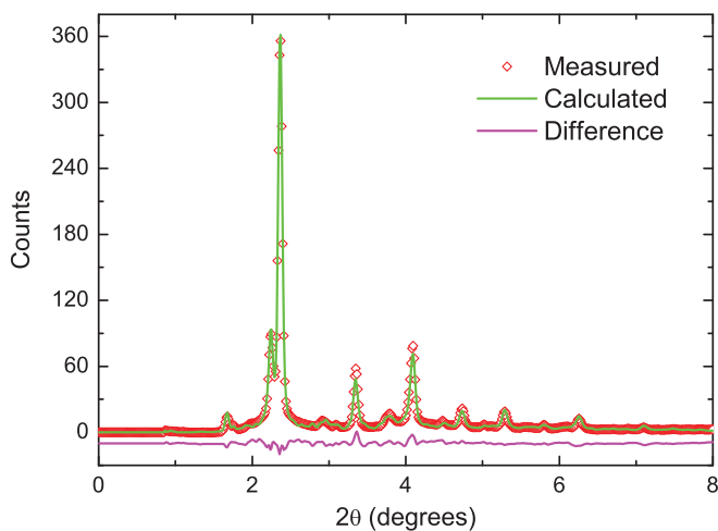
FIG. 9. (Color online) A Rietveld refinement of the diffraction data for \text{Cu}_{46}\text{Zr}_{54} after liquid solidification. The fits indicate a mixture of \text{Cu}_{10}\text{Zr}_7 and \text{Zr}_2\text{Cu} ; the input data are shown with red symbols (○), the prediction from the refined structure in a green line, and the difference in a purple line.
