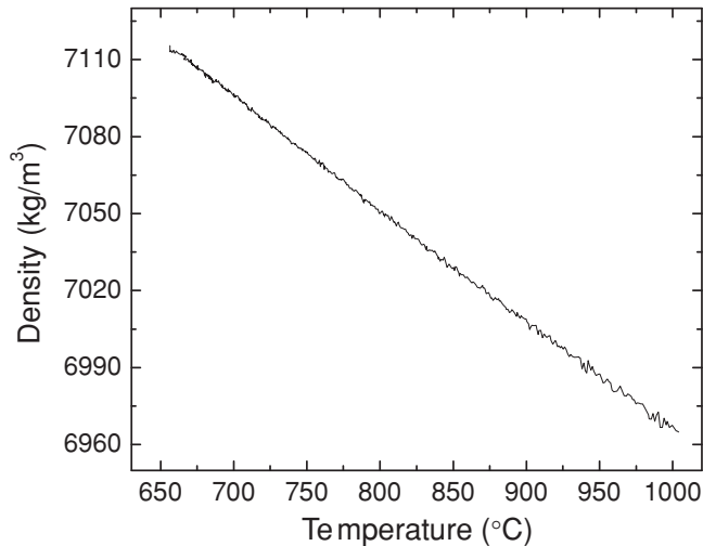
FIG. 8. The measured density for liquid \text{Cu}_{46}\text{Zr}_{54} ; no sudden changes can be seen across the temperature range studied.
