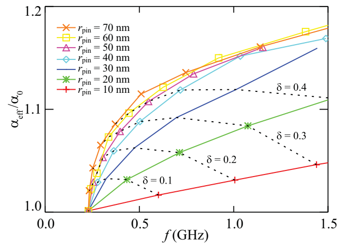
FIG. 6. (Color online) Frequency dependence of the effective damping for fixed A and various pinning potential radii r_{\text{pin}} = 10, 20, \dots, 70 nm and depth ratios \delta = 0, 0.1, 0.2, 0.3, 0.4 . Solid lines indicate values for constant r_{\text{pin}} and dashed lines constant \delta .
