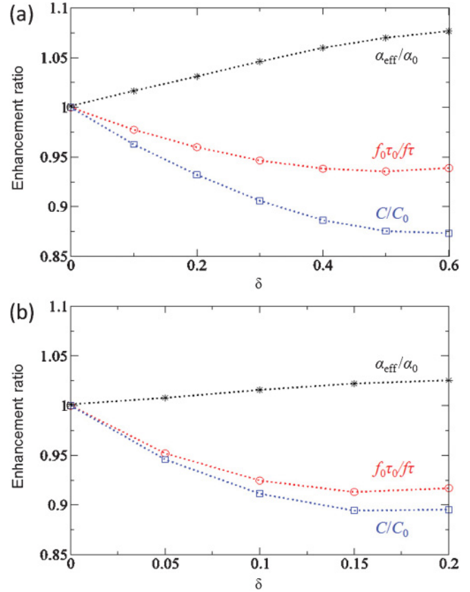
FIG. 5. (Color online) Enhancement ratio of f\tau , C , and \alpha_{\text{eff}} as a function of depth ratio \delta for (a) fixed A and (b) fixed l_{\text{ex}} . Subscript 0 indicates values in the free region before trapping.
