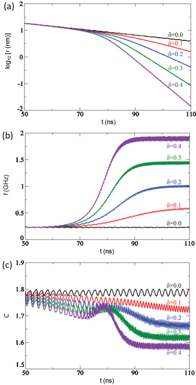
FIG. 4. (Color online) Time evolution of (a) gyration radius r , (b) gyration frequency f and (c) deformation factor C in a single pinning potential of the radius 10 nm for the depth ratio \delta = 0, 0.1, 0.2, 0.3 and 0.4 with fixed A . The gyration is excited by a 1 ns pulse of 20 mT.
