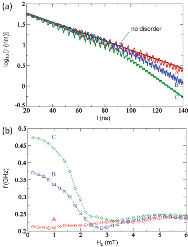
FIG. 3. (Color online) (a) Time evolution of gyration radius r for the disordered sample in Fig. 2 at points A, B, and C for \mathcal{D} = 0.05 with fixed A . To excite a vortex state, a Gaussian-type field pulse of 20 mT with 1 ns of the full width at half maximum along the y direction is applied. The black line is for the case without disorder. The small amplitude oscillations are due to the excitation procedure, which does not produce purely circular precession. (b) The gyration frequency averaged from t = 2 ns to 12 ns as a function of field-pulse amplitude at the points A, B, and C.
