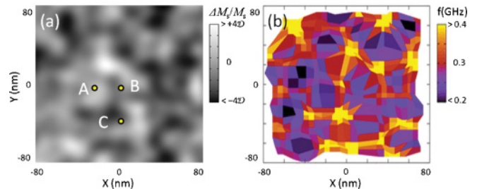
FIG. 2. (Color online) (a) A typical disorder image with 10-nm spatial correlation length and (b) contour maps of the gyration frequency as a function of position. (a) Part of the saturation magnetization within a \text{Ni}_{80}\text{Fe}_{20} disk with a 400-nm diameter and a 10-nm thickness. White indicates maxima in the magnetization and black minima. These results are based on a model of the disorder with \mathcal{D} = 0.05 and a fixed exchange stiffness constant A . (b) The gyration frequency according to the color scale on the right. To move the vortex positions, in-plane static magnetic fields from -10 mT to +10 mT along the x and y directions were applied. The gyration frequency is obtained by applying a field pulse of 0.1 mT for 200 ps along the y direction. The final location of the vortex core determines the real space position used in the figure.
