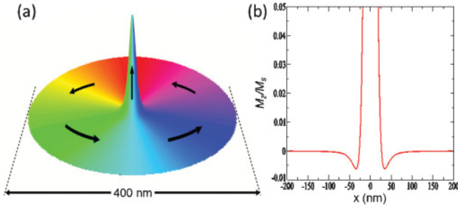
FIG. 1. (Color online) (a) A typical vortex structure in a \text{Ni}_{80}\text{Fe}_{20} disk with 400-nm diameter and 10-nm thickness calculated as described in Sec. II B. The color indicates the in-plane angle of the magnetization, and the arrows indicate the approximate magnetization direction. (b) Cross section of the z -component magnetization along the center of the vortex core in (a).
