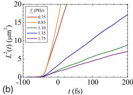
FIG. 2. (Color online) Diffusion length L(t) for both polarizations for various f_c [(a) TM polarization, (b) TE polarization]. The inset of (a) displays L(t) at f_c=f_1 and f_2 .
