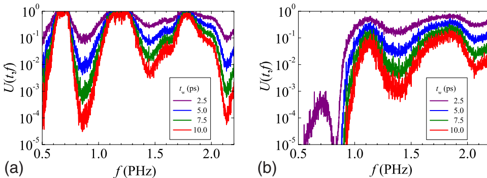
FIG. 6. (Color online) Time dependence of normalized internal energy spectra U(t, f) within the sample system for both polarizations [(a) TM polarization, (b) TE polarization]. Each spectrum was obtained by normalizing a spectrum with several time windows by a spectrum with time window (0, 2 ps).
