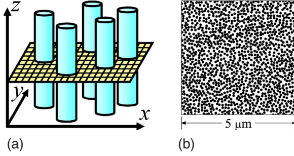
FIG. 1. (Color online) (a) Schematic view of the 2D FDTD model. (b) Top view of column configuration of a 5 \mu\text{m} square. In our simulation, the height of the columns is set to be infinity.
