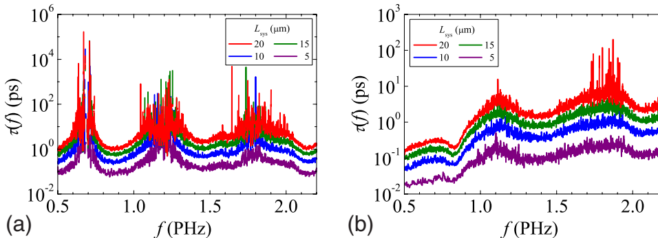
FIG. 8. (Color online) Frequency dependence of the photon lifetime \tau(f) of both polarizations for several system sizes [(a) TM polarization, (b) TE polarization].
