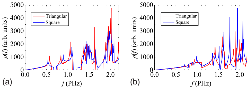
FIG. 12. (Color online) Frequency dependence of the density of states \rho(f) in the case of triangular and square lattice photonic crystals for both polarization [(a) TM polarization, (b) TE polarization].
