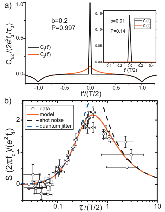
FIG. 3. (Color) (a) Contributions C_1(t') (black) and C_2(t') (red) to the current correlations C(t') in units of 2e^2 f_d / \tau_0 and as a function of t' for P=0.997 ( b=0.2 ). Inset: C_1(t') (black) and C_2(t') (red) for b=0.01 , P=0.14 . (b) Current noise spectrum S(2\pi f_d) at the center of the diamonds plotted as a function of the average escape time \tau . The experimental data are compared to our theoretical predictions without any adjustable parameter. The asymptotic limits of quantum jitter and phase noise are plotted in dashed blue and black lines.
