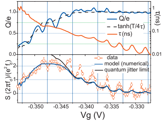
FIG. 2. (Color) (a) Average emitted charge Q and escape time \tau for 2eV_{exc} = \Delta as a function of V_g . The black dashed line is the Q(\tau) dependence expected for an exponential relaxation: Q = e \times \tanh \frac{T}{4\tau} . (b) Experimental current noise spectrum S as a function of V_g for 2eV_{exc} = \Delta (red points). The quantum jitter limit S = 4e^2 f_d \frac{(2\pi f_d \tau)^2}{1 + (2\pi f_d \tau)^2} , with \tau given by the experimental data of figure (a), has been plotted in black. The blue trace corresponds to the predictions of our model.
