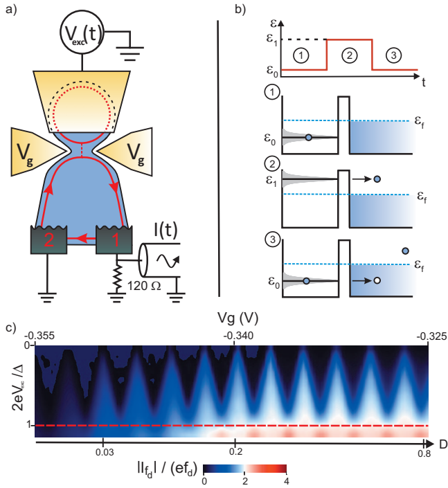
FIG. 1. (Color) (a) Sketch of the circuit. A single edge state is transmitted between the dot and the leads with transmission probability D controlled by the QPC gate voltage V_g . Charges emitted by the dot submitted to the excitation V_{exc}(t) are collected through contact 1. (b) Sketch of single-electron emission as described in the text. (c) Modulus of the average current first harmonic |I_{f_1}| in color scale as a function of the excitation amplitude and QPC gate voltage.
