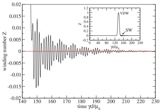
FIG. 6. (Color online) Spin wave behind a current driven VDW: winding number as function of time (at the cross section of 550th layer of the wire). Inset: the peak highlights the moment when a VDW passes the chosen layer (550th layer), the small oscillations correspond to the spin waves. These oscillations are shown in the main figure. ( u=0.4, \alpha=0.02, \beta=0.1 )
