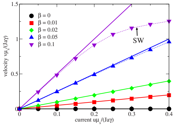
FIG. 5. (Color online) Domain wall velocity of a VDW as a function of u for different values of \beta . The label “SW” marks the region in which spin waves behind the domain wall occur.
