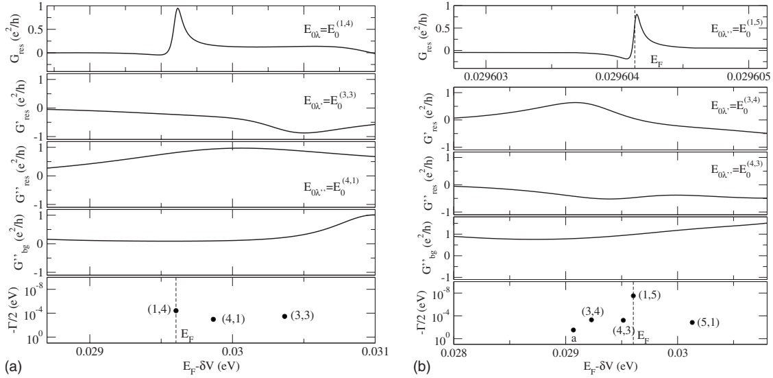
FIG. 12. Conductance peaks associated with isolated resonances: (a) \lambda=(1,4) , \lambda'=(3,3) , and \lambda''=(4,1) ; (b) \lambda=(1,5) , \lambda'=(3,4) , and \lambda''=(4,3) . Upper parts: resonant parts of the conductance G_{res} , G'_{res} , and G''_{res} and background part G''_{bg} ; Lower part: poles and position of the Fermi level in the complex energy plane. The potential energy in the dot region is constant, V_d=V_{0\lambda} .
