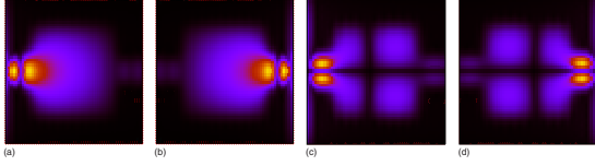
FIG. 9. (Color online) Electron probability distribution densities: (a) |\psi_1^{(1)}(x,y)|^2 and (b) |\psi_1^{(2)}(x,y)|^2 for the mode associated with the resonance a in Fig. 8(a); (c) |\psi_2^{(1)}(x,y)|^2 , and (d) |\psi_2^{(2)}(x,y)|^2 for the mode associated with the resonance a in Fig. 8(b).
