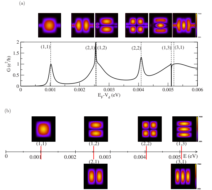
FIG. 5. (Color online) (a) Conductance as a function of the potential energy in the dot region. The maps represent the electron probability distribution density inside the dot, |\psi_n^{(s)}(E_F; x, y)|^2 for V_d = V_0^{(n_x, n_y)} (vertical dashed lines) for which E_0^{(n_x, n_y)} \approx E_F ; The incident scattering channel is n=1 for the odd modes in the lateral direction and n=2 for the even ones. (b) The eigenenergies \tilde{E}_{n_x, n_y} and the maps of the eigenstates, |\tilde{\psi}_{n_x, n_y}(x, y)|^2 , for the isolated dot. Bright corresponds to high values and dark corresponds to low values.
