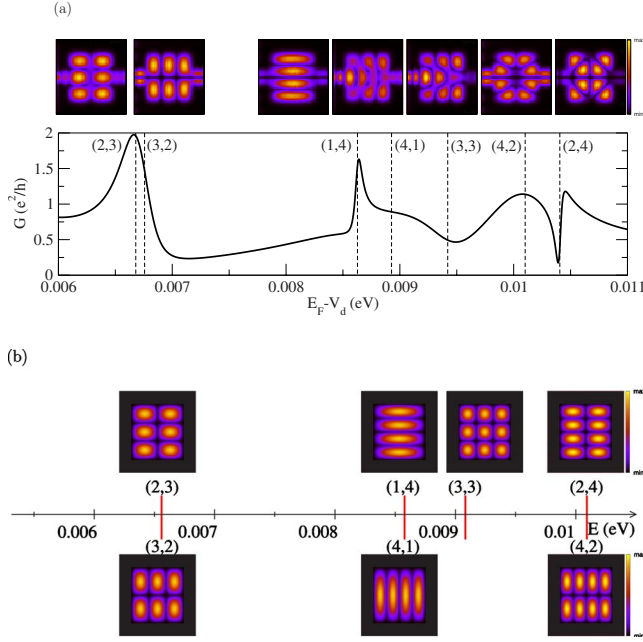
FIG. 6. (Color online) (a) Conductance as a function of the potential energy in the dot region. The maps represent the electron probability distribution density inside the dot, |\psi_n^{(s)}(E_F; x, y)|^2 for V_d = V_0^{(n_x, n_y)} (vertical dashed lines) for which E_0^{(n_x, n_y)} \approx E_F ; The incident scattering channel is n=1 for the odd modes in the lateral direction and n=2 for the even ones. For E_F - V_d \in [0.008, 0.011] eV, the conductance calculated in the frame of our model approximates qualitatively very well the experimental data given in Ref. 6, Fig. 2(a). (b) The eigenenergies \tilde{E}_{n_x, n_y} and the maps of the eigenstates, |\tilde{\psi}_{n_x, n_y}(x, y)|^2 , for the isolated dot. Bright corresponds to high values and dark corresponds to low values.
