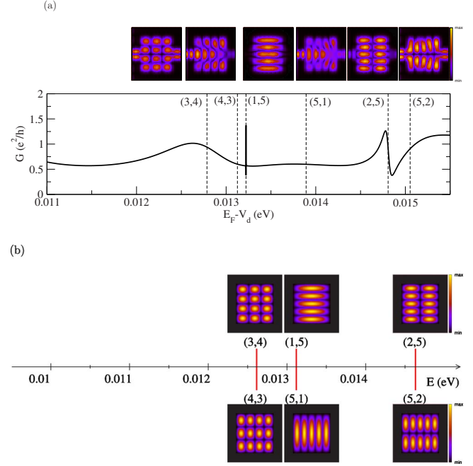
FIG. 7. (Color online) (a) Conductance as a function of the potential energy in the dot region. The maps represent the electron probability distribution density inside the dot, |\psi_n^{(s)}(E_F; x, y)|^2 for V_d = V_0^{(n_x, n_y)} (vertical dashed lines) for which E_0^{(n_x, n_y)} \approx E_F ; The incident scattering channel is n=1 for the odd modes in the lateral direction and n=2 for the even ones. (b) The eigenenergies \tilde{E}_{n_x, n_y} and the maps of the eigenstates, |\tilde{\psi}_{n_x, n_y}(x, y)|^2 , for the isolated dot. Bright corresponds to high values and dark corresponds to low values.
