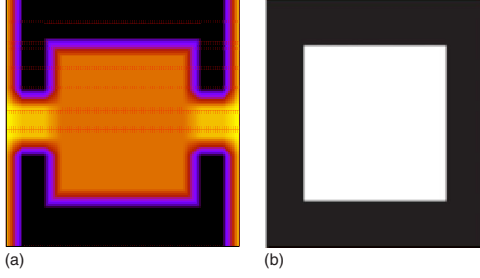
FIG. 2. (Color online) (a) Closed quantum dot by means of Neumann boundary conditions at the dot-contact interfaces. This is the potential energy for the Wigner-Eisenbud problem. (b) Isolated counterpart of the considered open quantum dot ( V_{b0}=V_{b1}=V_{b2} \rightarrow \infty ). Dark corresponds to high values and bright corresponds to low values.
