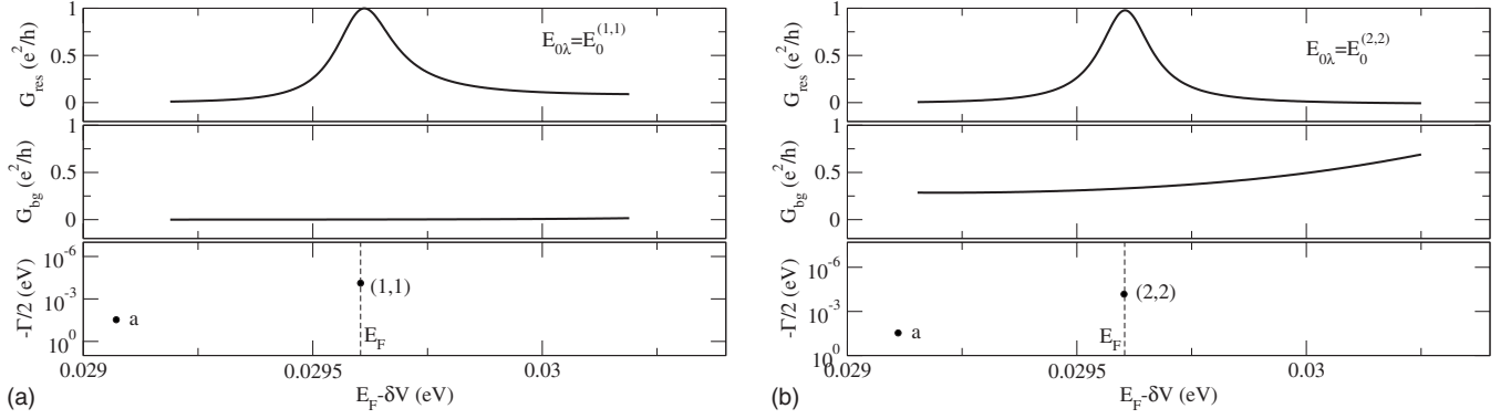
FIG. 8. Conductance peaks associated with isolated resonances: (a) \lambda=(1,1) and (b) \lambda=(2,2) . Upper part: resonant part of the conductance G_{res} ; middle part: background part of the conductance G_{bg} . Lower part: poles and position of the Fermi level in the complex energy plane. The potential energy in the dot region is constant, V_d=V_{0\lambda} .
