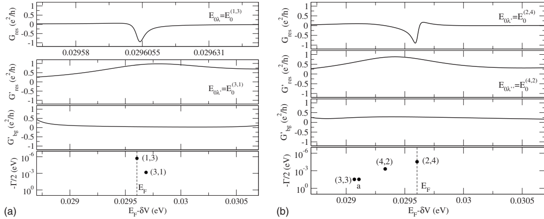
FIG. 11. Conductance peaks associated with isolated resonances: (a) \lambda=(1,3) , \lambda'=(3,1) ; (b) \lambda=(2,4) , \lambda'=(4,2) . Upper parts: resonant parts of the conductance G_{res} and G'_{res} and background part G'_{bg} ; Lower part: poles and position of the Fermi level in the complex energy plane. The potential energy in the dot region is constant, V_d=V_{0\lambda} .
