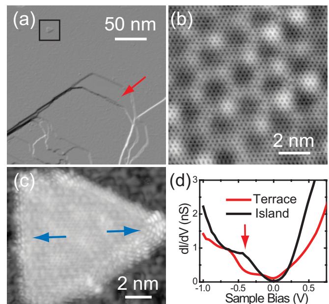
FIG. 2. (Color) STS measurements of graphene islands. (a) 0.25 \times 0.25 \mu\text{m}^2 gradient STM topograph (tunneling conditions are 1.0 V and 0.1 nA) showing a graphene island (black square) and a graphene terrace (red arrow). (b) Atomic-resolution ( 10 \times 10 \text{ nm}^2 ) STM topograph clearly shows the graphene lattice structure of the terrace seen in (a) (tunneling conditions are 0.3 V and 0.1 nA). (c) STM topograph ( 10 \times 8.7 \text{ nm}^2 ) of the triangular armchair graphene island in (a) (tunneling conditions are 0.3 V and 0.1 nA). (d) Spatially averaged STS taken from the graphene island of (c) (black curve) and the graphene terrace of (b) (red curve). The conditions for spectra are 0.3 V and 0.1 nA. The local minimum observed on the terrace STS (indicated by the red arrow) is believed to be the location of the Dirac point.
