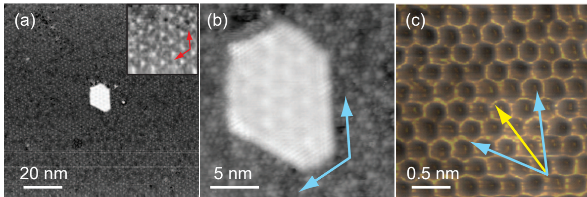
FIG. 1. (Color) Epitaxial graphene islands have preferred armchair edges. (a) 100 \times 100 \text{ nm}^2 STM topograph showing a small graphene island (white) surrounded by SiC reconstruction (tunneling conditions are 0.5 V and 0.1 nA). Inset: high-resolution STM topograph ( 12.5 \times 12.5 \text{ nm}^2 ) of the SiC reconstruction. The red arrows indicate the directions of the SiC lattice vectors. (b) Higher resolution STM image ( 20 \times 20 \text{ nm}^2 ) of the same graphene island (tunneling conditions are 0.5 V and 0.1 nA). The 6-sided island has edges aligned with the SiC lattice vectors. (c) 2.5 \times 2.5 \text{ nm}^2 rendered STM topograph showing the graphene lattice of the island (tunneling conditions are 0.3 V and 0.1 nA). Overlaid on this image are the two lowest energy edge directions: zigzag (yellow arrow) or armchair (blue arrows). Blue arrows match the directions of the island edges, meaning the island is entirely made up of armchair edges.
