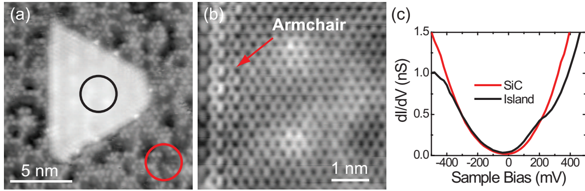
FIG. 3. (Color) Differences in STS between a graphene island and SiC reconstruction. (a) 15 \times 15 \text{ nm}^2 STM topograph (tunneling conditions are 0.3 V and 0.1 nA) showing another triangular armchair graphene island. (b) High-resolution STM image ( 5 \times 5 \text{ nm}^2 ) showing the armchair edge of the graphene island. (c) Spatially averaged STS from the center of the graphene island in (a) (black curve) and SiC reconstruction from the bottom right area of (a) (red curve). The two spectra are very similar at low bias. The conditions for spectra are 0.3 V and 0.1 nA.
