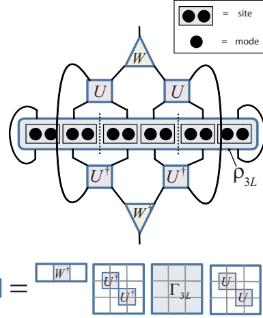
FIG. 1. (Color online) Top: a block of two sites (four modes) is coarse grained into an effective site by first applying disentangers U across the boundary of the block and then using isometry W to project out two modes. Bottom: same RG transformation written in the language of correlation matrices, Eq. (7).
