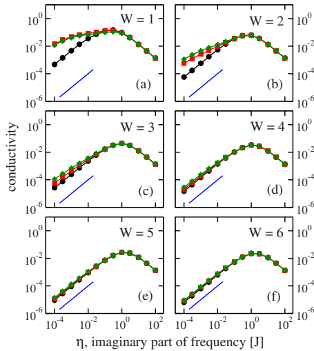
FIG. 2. (Color online) The dc conductivity as a function of the imaginary frequency, \eta , for the disordered XXZ chain ( J=1 ) with W=1-6 [(a)–(f)] for the noninteracting case, \Delta=0.0 (black line, circles) and for two interacting cases, \Delta=0.5 (red line, squares) and \Delta=1.0 (green line, diamonds). Error bars are smaller than the symbols. The blue line shows linear slope.
