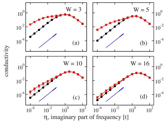
FIG. 4. (Color online) The same as in Fig. 2 but for the disordered t-t'-V model ( t=t'=1 ) with (a) W=3 , (b) W=5 , (c) W=10 , and (d) W=16 , for the noninteracting case, V=0 (black line, circles) and for the interacting case, V=2 (red line, squares). Where not shown, error bars are smaller than the symbols. The blue line shows linear slope.
