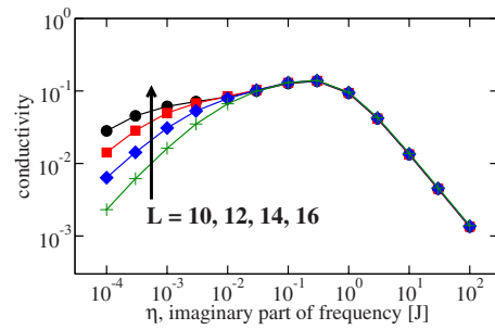
FIG. 3. (Color online) System-size dependence of the dc conductivity as a function of the imaginary frequency, \eta , for the disordered XXZ chain ( J=1 ) with \Delta=0.5 and W=1 . Conductivities are presented for L=10 (green line, plus signs), 12 (blue line, diamonds), 14 (red line, squares), and 16 (black line, circles), showing the development of the dc conductivity plateau in the L \rightarrow \infty limit.
