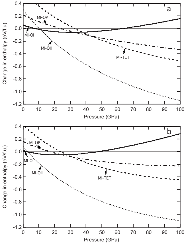
FIG. 3. Change in enthalpy with respect to MI versus pressure for various \text{ZrO}_2 phases for (a) GGA and (b) LDA. The difference in enthalpy curves with respect to MI is shown as MI-OI (solid), MI-OII (dotted), MI-OP (dashed-dotted), and MI-TET (dashed). Note the transition pressures for GGA: MI \rightarrow OI at 7.5 GPa, OI \rightarrow OII at 10.3 GPa. Likewise, the transition pressures for LDA: MI \rightarrow OI at 2.5 GPa, OI \rightarrow OII at 2.8 GPa. In both cases, the TET and OP phases have higher enthalpies.
