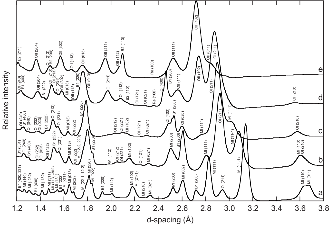
FIG. 1. X-ray diffraction patterns at various pressures during compression up to 42 GPa (run 2, unheated) taken at the CALIPSO beamline at the ALS show baddeleyite (MI), orthorhombic I (OI), orthorhombic II (OII), low-pressure phase NaCl (B1), and high-pressure NaCl (B2) corresponding Miller indices. A rhenium reflection from the gasket is marked with Re. Patterns shown are taken at the following pressures: (a) at 4.6 GPa, (b) at 11.8 GPa, (c) at 18 GPa, (d) at 26.2 GPa, and (e) at 42 GPa.
