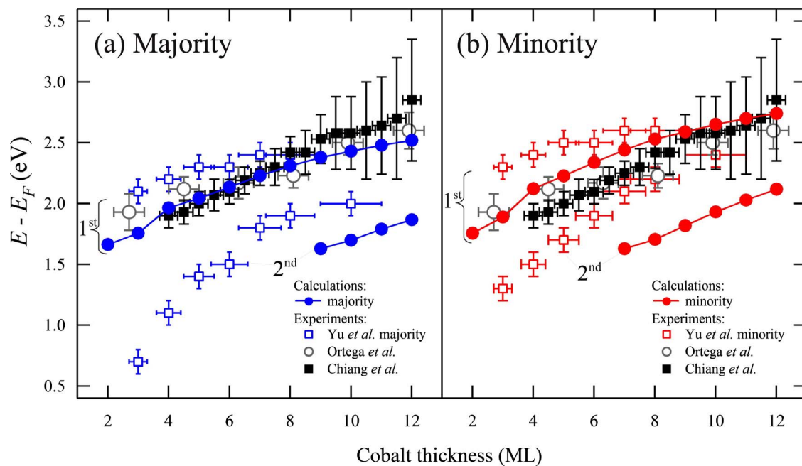
FIG. 5. (Color online) Dispersions of the unoccupied majority (a) and minority (b) quantum well states in Co/Cu(001). Experimental data are extracted from inverse photoemission [Yu et al. (Ref. 22) and Ortega et al. (Ref. 36)] and 2PPE (Chiang et al. , Ref. 21). Theoretical data are taken from Fig. 2(c). The two sets of quantum well states are labeled by 1 st and 2 nd .
