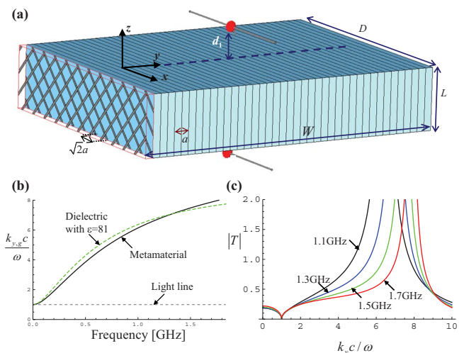
FIG. 1. (Color online) (a) Geometry of the metamaterial lens: a stack of dielectric slabs imprinted with an ultradense array of metallic strips with width w_s and tilted by \pm 45^\circ with respect to the interfaces. (b) Dispersion characteristic of the TE-guided modes supported by a metamaterial slab with parameters a/2=0.79 mm, L=11.7 mm, and w_s=0.247 mm (solid black line). The electric field is along the x direction and the direction of propagation is along y . (c) Amplitude of the transmission coefficient as a function of the normalized transverse wave vector component k_y for different frequencies of operation. The curves of panels (b) and (c) were calculated using the full wave electromagnetic simulator CST Microwave Studio TM (Ref. 12).
