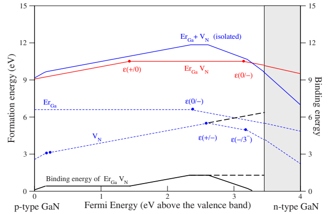
FIG. 5. (Color online) Formation energy and binding energy of the \text{Er}_{\text{Ga}}V_{\text{N}} pair as a function of the Fermi energy in hexagonal GaN. Dotted lines are the calculated formation energies of the isolated \text{Er}_{\text{Ga}} and V_{\text{N}} , the solid lines are their sum (blue), the formation energy of the \text{Er}_{\text{Ga}}V_{\text{N}} pair (red) and its binding energy (black), given as difference of the two curves.
