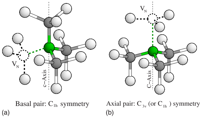
FIG. 4. (Color online) Defect pairs formed by \text{Er}_{\text{Ga}} substitutionals and V_{\text{N}} in hexagonal GaN. Because of the inequivalent N sites in hexagonal GaN (the Er-N bond along the c axis is longer than the other three), the complexes can be formed in two configurations. The basal configuration (left-hand side) has C_{1h} symmetry, whereas the ideal axial configuration (right-hand side) has the C_{3v} symmetry, or the C_{1h} if a Jahn-Teller distortion occurs.
