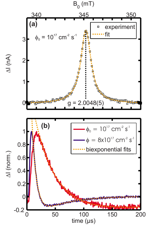
FIG. 3. (Color online) Results of a pEDMR experiment carried out at T = 10 \text{ K} using a photocurrent of I_{\text{ph}} = -1 \mu\text{A} . (a) Current change at t = 10 \mu\text{s} after a 320-ns-long mw pulse (pEDMR spectrum). The spectrum reveals a single Lorentzian line at g = 2.0048(5) (dashed line) which in accordance with the g value of conduction-band tail states in amorphous silicon. The linewidth is dominated by power broadening resulting from the high mw power ( B_1 \approx 70 \mu\text{T} ) used in the experiment. (b) Current relaxation as a function of time after the mw excitation (pEDMR transient) on the resonance position at g = 2.0048(5) measured at two different light intensity levels as indicated in the legend. The dashed lines represent fits to the experimental data assuming a combination of two exponential functions for each transient. The respective time constants are given in the text.
