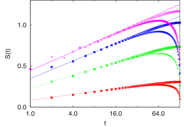
FIG. 4. (Color online) Time evolution of the entropy after a quench from two disconnected chains into an open chain with one defect having different strengths \Delta=1.0 (homogeneous), \Delta=0.75 , \Delta=0.5 , and \Delta=0.25 , from the top to the bottom. In the \log t scale the initial part of the curves for L=128 and L=256 are close to the indicated straight lines having the slope c_{\text{eff}}(\Delta)/3 , which is calculated from the scaling of the equilibrium entropy (see Fig. 2).
