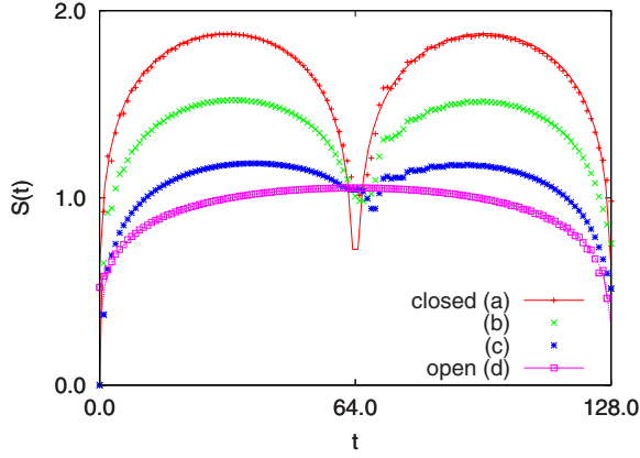
FIG. 3. (Color online) Time evolution of the entropy after a quench from two disconnected chains. The final system is closed and homogeneous (a) or contains one (b) or two (c) defects of strength \Delta=1/2 . The quench to a homogeneous open chain is given by (d). The analytical formulae for the homogeneous closed Eq. (15) and open Eq. (16) chains are also shown by full lines.
