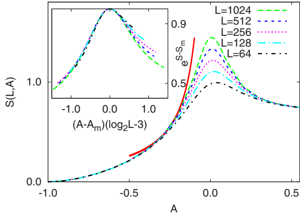
FIG. 5. (Color online) The entanglement entropy of the quantum Ising chain with two symmetrically placed extended defects as a function of the strength of the defect, A , for different finite systems. The conjectured asymptotic behavior in Eq. (20) is indicated by the full red curve. Inset: Scaling plot of the entanglement entropy around its maxima [ \exp(S - S_m) ] in terms of the combination (A - A_m)/(\log_2 L - 3) , see the text.
