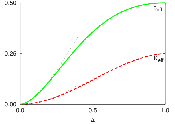
FIG. 2. (Color online) Effective central charge, c_{\text{eff}}(\Delta) (full line green), and the parameter, \kappa_{\text{eff}}(\Delta) (broken line red), of the single-copy entanglement of the quantum Ising chain as a function of the strength of the localized defect, \Delta . For small \Delta the leading behaviors obtained by perturbational calculation are indicated by dotted lines.
