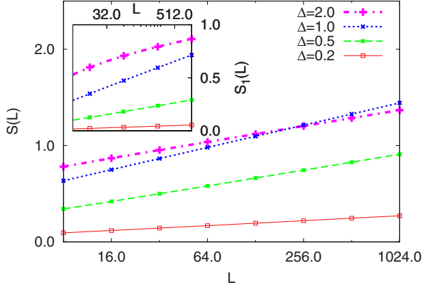
FIG. 1. (Color online) Entanglement entropy of the quantum Ising chain with different strength of the defect as a function of the logarithm of the length. The calculated values at discrete L 's are denoted by symbols, the lines connecting these points are guide to the eye. Inset: the same for the single-copy entanglement.
