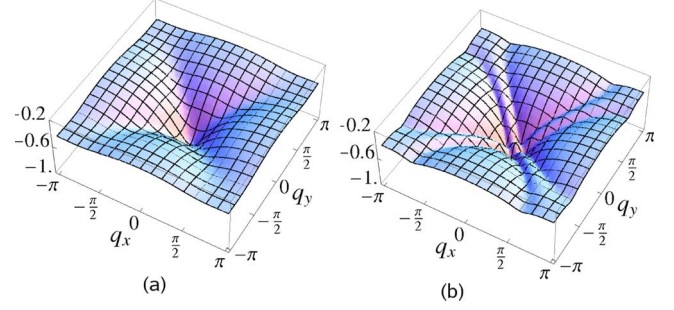
FIG. 1. (Color online) Mean-field kinetic term P_a(0, \mathbf{q})/t of the \mathbf{a} -boson as a function of spacelike momenta for U/t=3 and t'=0 . In Fig. 1(a) \mu=0 and T/t=0.205 , in Fig. 1(b) \mu/t=-0.27 and T/t=0.0435 . Both temperatures are mean-field critical temperatures.
