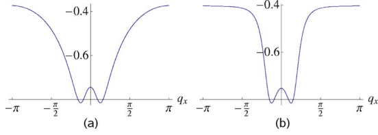
FIG. 3. (Color online) In (a) the mean-field approximation for bosonic kinetic term P_a(0, q_x, 0)/t is shown as a function of the x component of spatial momenta. Parameters are U/t=3 , \mu/t=-0.35 , t'=0 , and T/t=0.1 . Figure 3(b) shows the same quantity according to our approximation given by Eqs. (11) and (16) with the values of A_a , \hat{q} , and D drawn from the mean-field computation.
