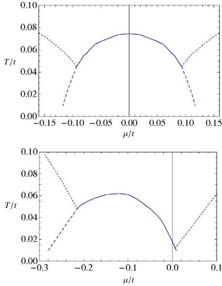
FIG. 5. (Color online) Renormalization group results for the pseudocritical temperature T_{pc}/t as a function of \mu/t , given by the solid (commensurate) and dashed (incommensurate) lines. Results are displayed for U/t=3 , t'=0 (upper panel) and t'/t=-0.05 (lower panel).
