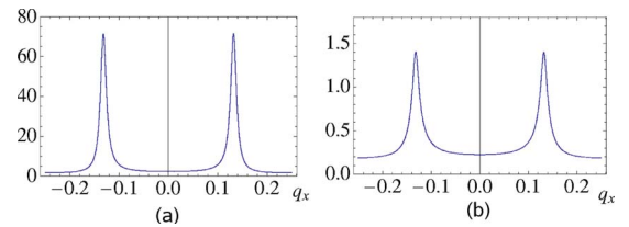
FIG. 7. (Color online) Figure 7(a) shows the spin susceptibility [P_a(0, q_x, 0)/t]^{-1} and Fig. 7(b) the bosonic occupation number n_a(q_x, 0) for \mu/t=-0.12 , T/t=0.01 , U/t=3 , and t'=0 according to the renormalization group computations. Both curves are given as a function of spatial momentum in x direction. A peak at q_x=0 would signal the dominance of commensurate antiferromagnetism. The actual peaks, located at \hat{q} = \pm 0.132 , indicate incommensurate antiferromagnetism.
