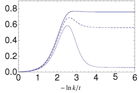
FIG. 2. (Color online) Renormalization flow of the gradient coefficient A_{a,k} for U/t=3 and \mu/t=-0.12 according to Eq. (18) in the parameter regime where we have commensurate antiferromagnetism and therefore \partial_k \hat{q} = 0 . The solid line corresponds to T/t=0.08 , the long-dashed line to T/t=0.07 , and the short-dashed line to T/t=0.058 .
