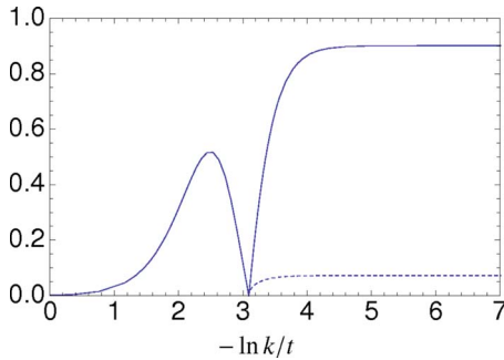
FIG. 4. (Color online) Renormalization flow of the gradient coefficient A_{a,k} and the incommensurability \hat{q} according to Eqs. (18) and (20) at \mu/t=-0.12 and T/t=0.05 , where incommensurate antiferromagnetism dominates. The solid line shows A_a decreasing to zero at -\ln k/t=3.09 and increasing again when the incommensurability \hat{q} (short-dashed line) sets in.
