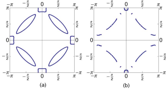
FIG. 8. (Color online) Mean-field effective Fermi surfaces for \mu/t = -0.6 , t'/t = -0.2 , and gap parameter A/t = 0.1 . Figure 8(a) shows the commensurate case \hat{q} = 0 where the Fermi surface exhibits hole- and particle pockets at the magnetic Brillouin zone boundary. In Fig. 8(b), the remainders of the effective Fermi surface are shown for a nonzero incommensurability \hat{q} = 0.3 along the x axis.
