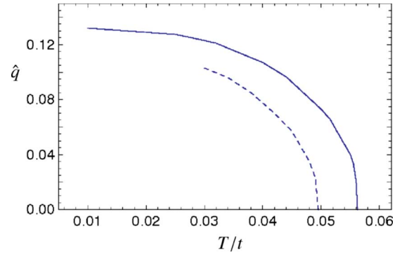
FIG. 6. (Color online) Renormalization group results for the incommensurability \hat{q} as a function of T for U/t=3 , t'=0 , and \mu/t=-0.12 (solid line) and \mu/t=-0.105 (dashed line).
