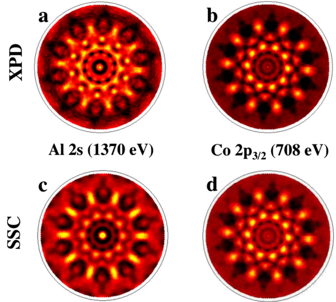
FIG. 5. (Color online) Experimental XPD patterns of (a) Al 2s and (b) Co 2p_{3/2} core levels measured on the Al 13 Co 4 (100) surface with an Al K_{\alpha} (1486.7 eV) x-ray source. (c) and (d) Single scattering cluster simulations for Al 2s ( E_{kin}=1370 eV) and (d) Co 2p_{3/2} ( E_{kin}=708 eV) emission based on a cluster of 3016 atoms derived from the bulk model (Ref. 12) described in Fig. 1.
