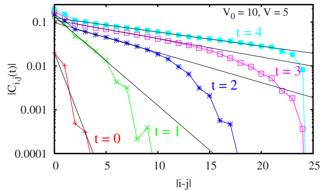
FIG. 5. (Color online) Equal-time density correlation function as a function of distance |i-j| at different times for the quench from V_0=10 to V=5 . The black lines are fits to exponential decays.
