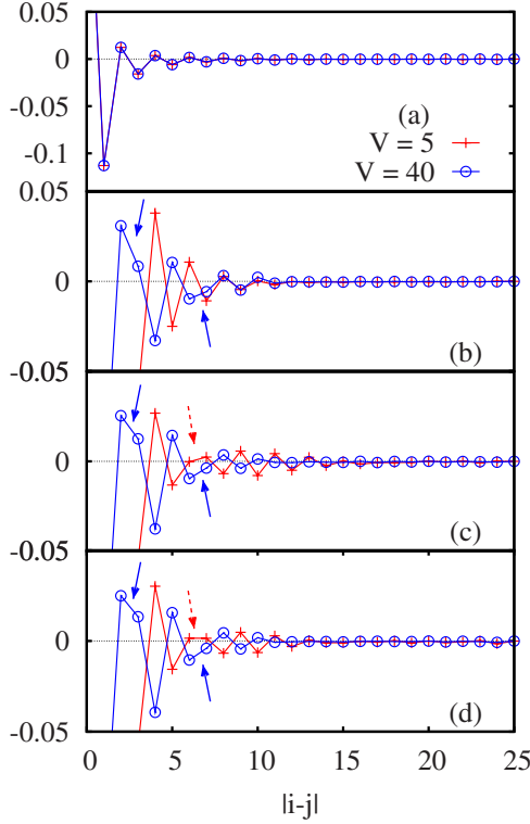
FIG. 8. (Color online) Equal-time density correlation function C_{i,j}(t) of spinless fermions after a quench from the Luttinger-liquid ground state of H(V_0) with V_0=0.5 , evolved by the Hamiltonian H(V) , with V=5 and V=40 , at fixed times (a) t=0 , (b) t=1.4 , (c) t=2.8 , and (d) t=4.2 as functions of the separation |i-j| . The blue (solid) arrows highlight the position of the phase slips obtained for V=40 , the red (dashed) ones point to the phase slips for the case V=5 .
