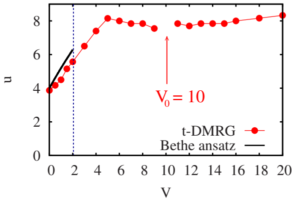
FIG. 6. (Color online) Velocity of the horizon in the time evolution of the equal-time density correlation function C_{i,j}(t) of spinless fermions after a quench from the CDW ground state of H(V_0) with V_0=10 , evolved by the Hamiltonian H(V) as a function of V . The estimated error is of the order of the point size. The dashed vertical line indicates the quantum phase transition from the Luttinger liquid to the CDW regime.
