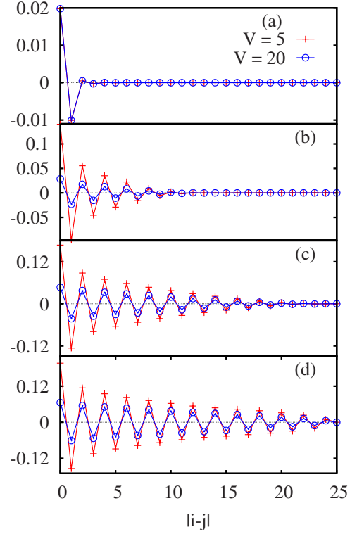
FIG. 4. (Color online) Equal-time density correlation function C_{i,j}(t) after a quench from the CDW ground state of H(V_0) with V_0=10 , evolved by the Hamiltonian H(V) , with V=5 and V=20 , at fixed times (a) t=0 , (b) t=1.4 , (c) t=2.8 , and (d) t=4.2 as functions of the separation |i-j| .
