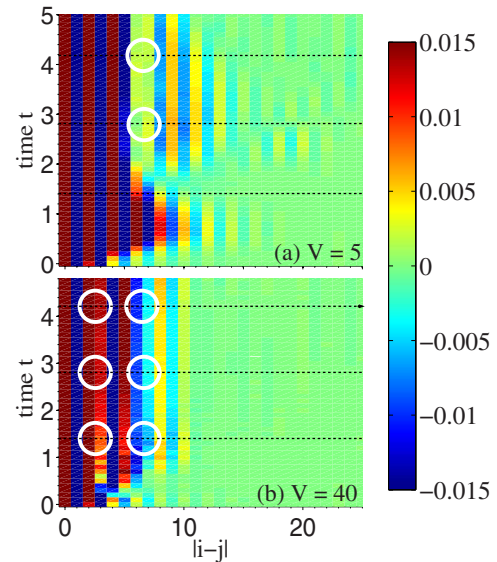
FIG. 7. (Color online) Time evolution of the equal-time density correlation function C_{i,j}(t) after a quench from the Luttinger-liquid ground state of H(V_0) with V_0=0.5 , evolved by the Hamiltonian H(V) , with (a) V=5 and (b) V=40 . The dashed horizontal lines indicate the time steps shown in Figs. 8(b)–8(d); the white circles highlight the phase slips visible there.
