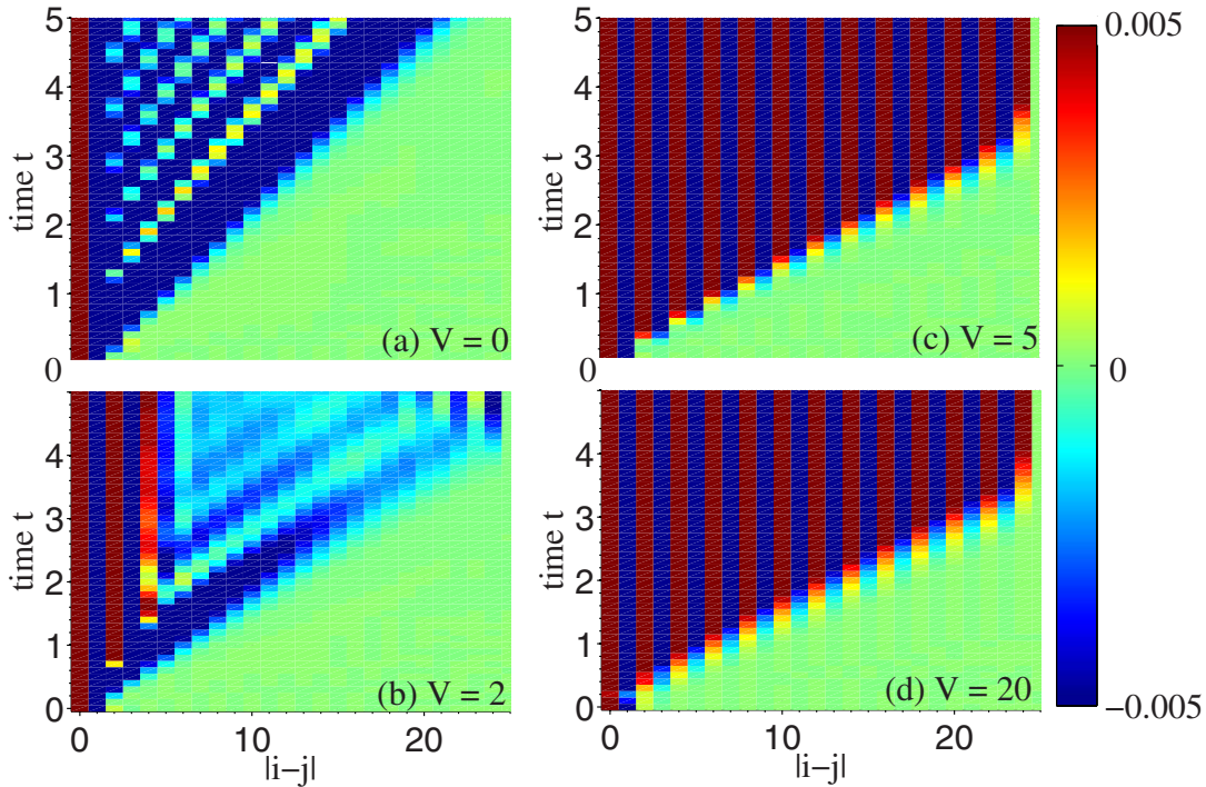
FIG. 1. (Color online) Time evolution of the equal-time density correlation function C_{i,j}(t) of spinless fermions after a quench from the CDW ground state of H(V_0) with V_0=10 , evolved by the Hamiltonian H(V) , with (a) V=0 , (b) V=2 , (c) V=5 , (d) and V=20 .
