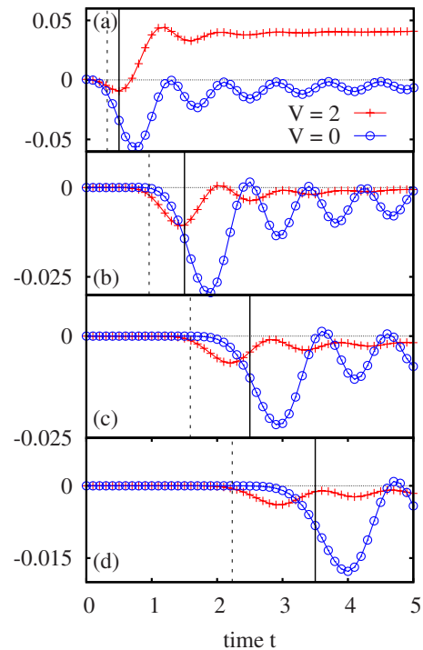
FIG. 2. (Color online) Equal-time density correlation function C_{i,j}(t) of spinless fermions after a quench from the CDW ground state of H(V_0) with V_0=10 , evolved by the Hamiltonian H(V) , with V=0 and V=2 , at fixed separations (a) |i-j|=2 , (b) 6, (c) 10, and (d) 14 as functions of time t . The black vertical lines indicate the position of the horizon for V=0 , which moves with velocity u=4 , and the dashed vertical lines a horizon moving with velocity u=2v(V=2)=2\pi .
