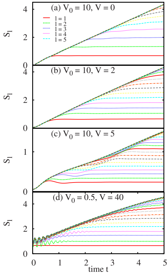
FIG. 10. (Color online) Time evolution of the von Neumann entropy S_l(t) for subsystems of different sizes l=1, 2, \dots, 25 , after quenches with (a) V_0=10 \rightarrow V=0 , (b) V_0=10 \rightarrow V=2 , (c) V_0=10 \rightarrow V=5 , and (d) V_0=0.5 \rightarrow V=40 . The lowest line corresponds to l=1 , the next to l=2 and so on; for clarity, the curves for l \leq 5 are labeled.
