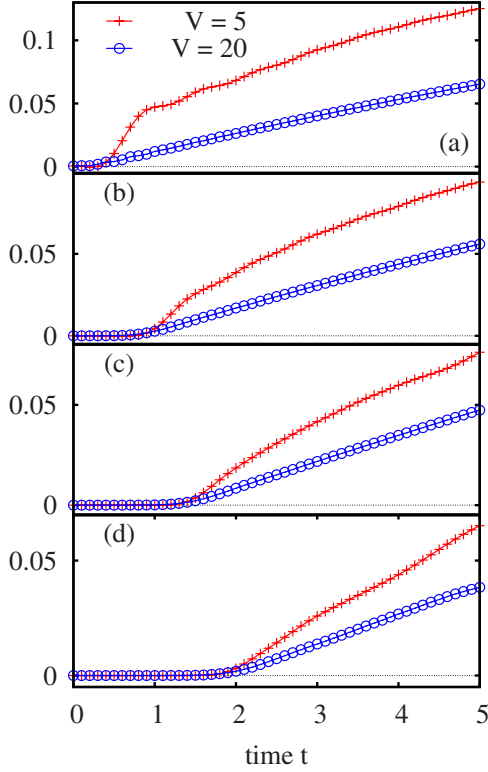
FIG. 3. (Color online) Equal-time density correlation function C_{i,j}(t) of spinless fermions after a quench from the CDW ground state of H(V_0) with V_0=10 , evolved by the Hamiltonian H(V) , with V=5 and V=20 , at fixed separations |i-j|=2 (a), 6 (b), 10 (c), and 14 (d) as functions of time t after the quench.
