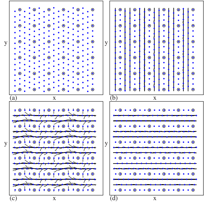
FIG. 21. (Color online) The vortex positions (black dots), pinning site locations (open circles), and vortex trajectories (black lines) for the system in Fig. 18 at B/B_\phi=12 . (a) The partially ordered vortex configuration at F_D=0 . The vortex structure has a smecticlike ordering in which all of the topological defects are aligned in the same direction. (b) The vortex trajectories just above depinning for driving in the y direction, showing two columns of interstitial vortices moving between each pair of pinning columns and two interstitial vortices trapped between adjacent pinning sites. (c) The vortex trajectories just above depinning for driving in the x direction. A portion of the interstitial vortices shift in the y direction in order to create ordered rows of flowing vortices and pairs of trapped interstitial vortices between adjacent pinning sites. (d) The steady-state channels that form for the y -direction driving. The general structural rearrangement of the interstitial vortices for depinning in the x direction is similar to that seen at B/B_\phi=4 in Figs. 19(c) and 19(d).
