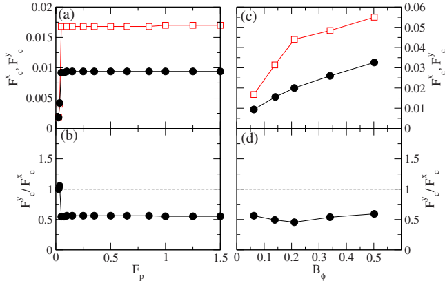
FIG. 20. (Color online) (a) F_c^x (open squares) and F_c^y (filled circles) vs F_p for the system in Fig. 18 at B/B_\phi=4 with the starting configuration shown in Fig. 19 that produces a higher depinning threshold in the x direction. (b) The corresponding anisotropy ratio F_c^y/F_c^x vs F_p . For small F_p the system depins elastically. (c) F_c^x (open squares) and F_c^y (filled circles) vs B_\phi for the same system at B/B_\phi=4 and F_p=0.85 . (d) The corresponding F_c^y/F_c^x vs F_p .
