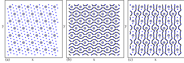
FIG. 8. (Color online) Vortex positions (black dots), pinning site locations (open circles), and vortex trajectories (black lines) for the triangular pinning lattice system in Fig. 2 at B/B_\phi=7 . (a) At F_D=0 , a triangular vortex lattice forms that is not aligned with the x or y axis but is tilted at an angle \theta \approx -78^\circ to the x axis. This ground state is twofold degenerate since the vortex lattice could have been tilted at the opposite angle, \theta \approx +78^\circ , to the x axis. (b) The vortex trajectories just above depinning for driving in the x direction. All of the interstitial vortices are moving. (c) The vortex trajectories just above depinning for driving in the y direction. In this case a portion of the interstitial vortices remains pinned.
