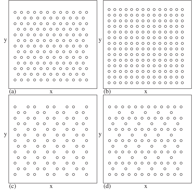
FIG. 1. The pinning site locations (open circles) for (a) a triangular pinning array, (b) a square pinning array, (c) a honeycomb pinning array, and (d) a kagomé pinning array. The driving force is applied along \hat{y} to determine the depinning force F_c^y and along \hat{x} to determine F_c^x .
