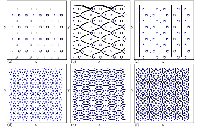
FIG. 23. (Color online) Vortex positions (black dots), pinning site locations (open circles), and vortex trajectories (black lines) for the honeycomb pinning array in Fig. 22. (a) At B/B_\phi^H=1.5 and F_D=0 there is one vortex per large interstitial site. (b) Vortex trajectories just above depinning for driving in the y direction at B/B_\phi^H=1.5 , showing one-dimensional paths between the pinning sites. At this field, F_c^y/F_c^x < 1 . (c) Vortex trajectories just above depinning for driving in the x direction at B/B_\phi^H=1.5 . The interstitial vortices flow in winding paths around the occupied pinning sites. (d) The vortex configurations at B/B_\phi^H=4 for F_D=0 . Here a portion of the interstitial vortices align in the x direction. (e) Vortex trajectories just above depinning for driving in the x direction at B/B_\phi^H=4 . In addition to moving channels of interstitial vortices, there are some interstitial vortices that remain pinned between adjacent occupied pinning sites. (f) Vortex trajectories just above depinning for driving in the y direction at B/B_\phi^H=4 show a complex periodic pattern with all of the interstitial vortices moving.
