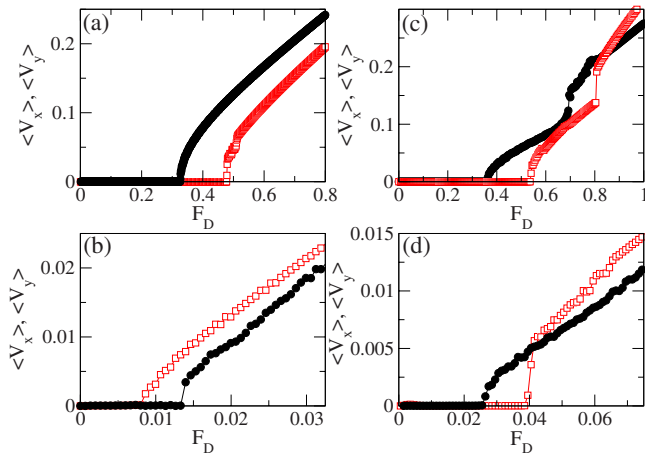
FIG. 24. (Color online) The velocity-force curves from the system in Fig. 22. Open squares: \langle V_x \rangle vs F_D ; filled circles: \langle V_y \rangle vs F_D . (a) The honeycomb pinning array at B/B_\phi^H=1.5 where F_c^y/F_c^x < 1 . (b) The honeycomb pinning array at B/B_\phi^H=4 , showing that the anisotropy has reversed and F_c^y/F_c^x > 1 . (c) The kagomé pinning array at B/B_\phi^K=4/3 . (d) The kagomé pinning array at B/B_\phi^K=10/3 . Here dV_y/dF_D < dV_x/dF_D , so there is a crossing of the velocity-force curves.
