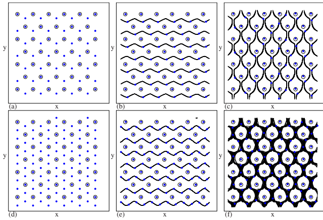
FIG. 5. (Color online) Vortex positions (black dots), pinning site locations (open circles), and vortex trajectories (black lines) for the triangular pinning lattice system in Fig. 2. (a) The vortices form a honeycomb configuration at F_D=0 and B/B_\phi=2 . (b) The vortex trajectories just above depinning for driving in the x direction at B/B_\phi=2 . The vortices channel between the pinning rows. (c) Vortex trajectories just above depinning for driving in the y direction at B/B_\phi=2 . The moving interstitial vortices wind around the occupied pinning sites. (d) The vortices form a triangular configuration at F_D=0 and B/B_\phi=3 . (e) The vortex trajectories just above depinning for driving in the x direction at B/B_\phi=3 show an ordered interstitial flow of vortices between the pinning sites. (f) Vortex trajectories just above depinning for driving in the y direction at B/B_\phi=3 . Here the flow is disordered.
