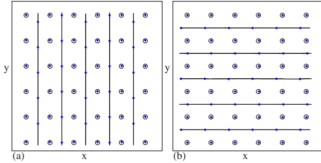
FIG. 17. (Color online) Vortex positions (black dots), pinning site locations (open circles), and vortex trajectories (black lines) just above depinning for a system with a square pinning array at F_p = 0.86 , R_p = 0.35\lambda , and B_\phi = 0.0625\phi_0/\lambda^2 at B/B_\phi = 2 . (a) The y -direction driving. (b) The x -direction driving. The same type of vortex motion occurs for both directions of drive.
