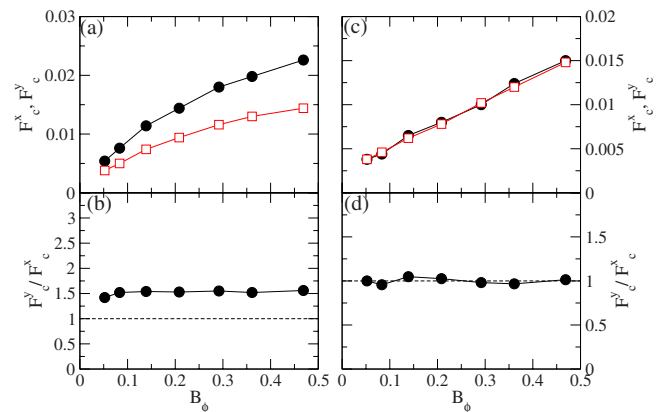
FIG. 14. (Color online) (a) The depinning thresholds F_c^x (open squares) and F_c^y (filled circles) vs B_\phi for a triangular pinning lattice system with F_p=0.85 and R_p=0.35\lambda at B/B_\phi=4 . (b) The corresponding F_c^y/F_c^x vs B_\phi . (c) F_c^x (open squares) and F_c^y (filled circles) vs B_\phi for the same system at B/B_\phi=5 . (d) The corresponding F_c^y/F_c^x vs B_\phi showing that the depinning is isotropic.
