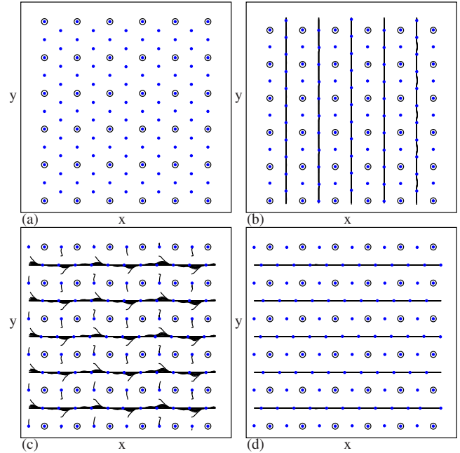
FIG. 19. (Color online) The vortex positions (black dots), pinning site locations (open circles), and vortex trajectories (black lines) for the square pinning lattice system in Fig. 18 at B/B_\phi = 4 . (a) The F_D = 0 state where a triangular vortex lattice forms that is aligned in the y direction. (b) The vortex trajectories just above depinning for driving in the y direction, showing one-dimensional channels of vortices moving between adjacent columns of pinning sites. (c) The vortex trajectories just above depinning for driving in the x direction. Here, every other column of vortices shifts in the y direction so that every other vortex can join one-dimensional rows of vortices flowing between adjacent pinning site rows, while the remaining interstitial vortices are trapped between neighboring pinning sites. (d) The same as panel (c) but at a later time when the system has reached steady-state flow.
