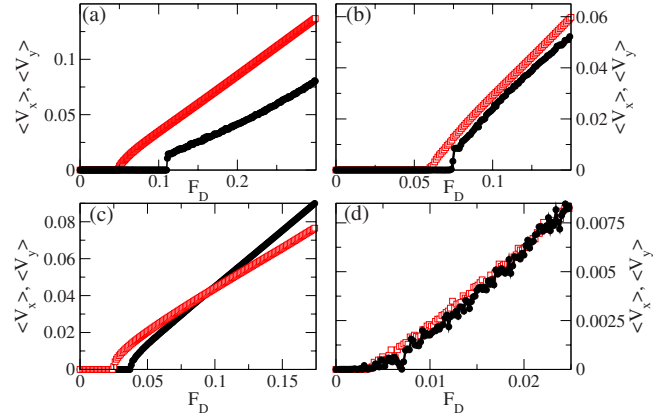
FIG. 3. (Color online) Velocity-force curves for driving in the x direction, \langle V_x \rangle (open squares), and in the y direction, \langle V_y \rangle (filled circles) for the triangular pinning lattice system in Fig. 2. (a) At B/B_\phi = 2 , the slope dV_y/dF_D < dV_x/dF_D . (b) At B/B_\phi = 3 , dV_y/dF_D = dV_x/dF_D . (c) At B/B_\phi = 4 , dV_x/dF_D < dV_y/dF_D , resulting in a crossing in the velocity-force curves near F_D = 0.1 . (d) At B/B_\phi = 5 , the depinning is isotropic.
