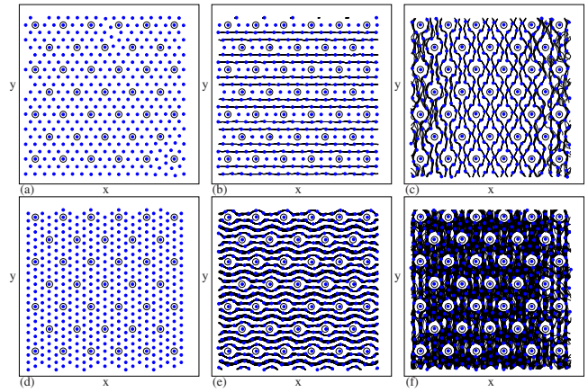
FIG. 7. (Color online) Vortex positions (black dots), pinning site locations (open circles), and vortex trajectories (black lines) for the triangular pinning lattice system in Fig. 2. (a) At F_D=0 and B/B_\phi=9 , a triangular vortex lattice forms. (b) The vortex trajectories just above depinning for driving in the x direction at B/B_\phi=9 . Two rows of interstitial vortices move in one-dimensional paths between the rows of pinning sites while a portion of the interstitial vortices remain pinned. (c) The vortex trajectories just above depinning for driving in the y direction at B/B_\phi=9 . A combination of ordered and disordered flows occurs. (d) At F_D=0 and B/B_\phi=12 , a triangular vortex lattice forms which is aligned with the y direction. (e) The vortex trajectories just above depinning for driving in the x direction at B/B_\phi=12 . Three rows of interstitial vortices move between the rows of pinning sites. (f) Vortex trajectories just above depinning for driving in the y direction at B/B_\phi=12 show the existence of disordered flow.
