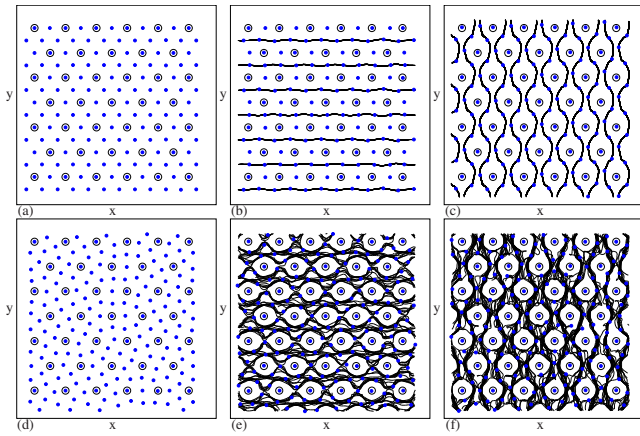
FIG. 6. (Color online) Vortex positions (black dots), pinning site locations (open circles), and vortex trajectories (black lines) for the triangular pinning lattice system in Fig. 2. (a) At F_D=0 and B/B_\phi=4 a triangular vortex lattice forms. (b) The vortex trajectories just above depinning for driving in the x direction at B/B_\phi=4 . A portion of the interstitial vortices moves in one-dimensional channels between the rows of pinning sites. (c) The vortex trajectories just above depinning for driving in the y direction at B/B_\phi=4 . The interstitial vortices flow in winding channels around the pinning sites. (d) At F_D=0 and B/B_\phi=5 , the vortex lattice is disordered. (e) The vortex trajectories just above depinning for driving in the x direction at B/B_\phi=5 . The vortex flow pattern is disordered. (f) Vortex trajectories just above depinning for driving in the y direction at B/B_\phi=5 . The same type of disordered flow pattern seen for the x -direction driving appears for the y -direction driving.
