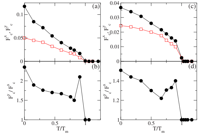
FIG. 16. (Color online) (a) The depinning thresholds F_c^x (open squares) and F_c^y (filled circles) vs T/T_m for a triangular pinning lattice system with F_p=1.25 and B/B_\phi=2 . Here T_m is the temperature associated with the onset of vortex diffusion at F_D=0 . (b) The corresponding anisotropy ratio F_c^y/F_c^x vs T/T_m . (c) F_c^x (open squares) and F_c^y (filled circles) vs T/T_m for the same system at B/B_\phi=4 . (d) The corresponding F_c^y/F_c^x vs T/T_m .
