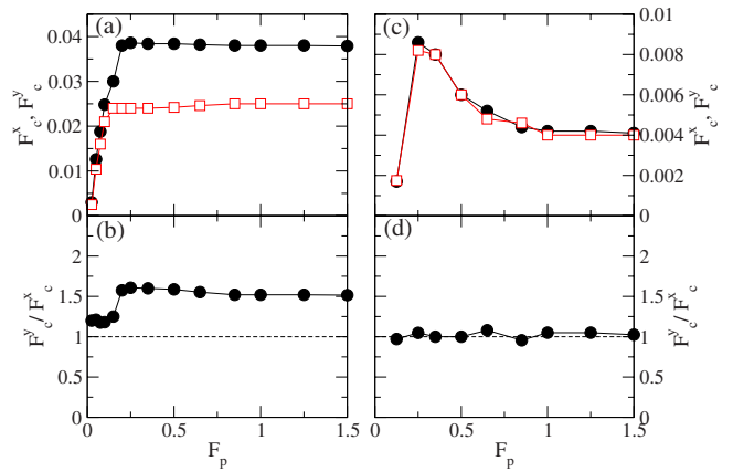
FIG. 12. (Color online) (a) The depinning threshold in the x direction, F_c^x (open squares), and y direction, F_c^y (filled circles), vs F_p for the triangular pinning lattice system in Fig. 2 at B/B_\phi=4 . (b) The corresponding anisotropy ratio F_c^y/F_c^x vs F_p . (c) F_c^x and F_c^y vs F_p for the same system at B/B_\phi=5 . (d) The corresponding anisotropy ratio F_c^y/F_c^x vs F_p . Here the depinning is isotropic and a peak in the depinning thresholds occurs near the transition from the plastic to the elastic depinning regime.
