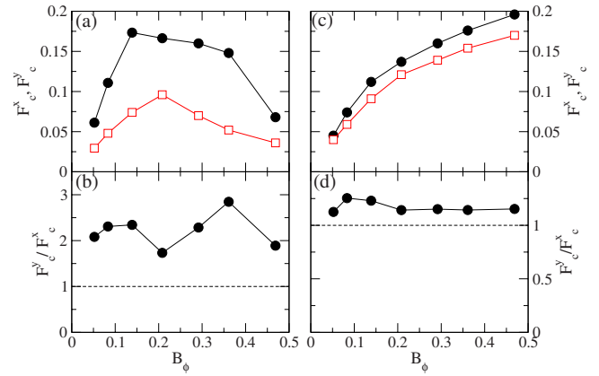
FIG. 13. (Color online) (a) The depinning threshold in the x direction, F_c^x (open squares), and y direction, F_c^y (filled circles), vs B_\phi for a triangular pinning lattice system with F_p=0.85 and R_p=0.35\lambda at B/B_\phi=2 . The vortex lattice has honeycomb ordering at low B_\phi , but as B_\phi increases, the increasing strength of the vortex-vortex interactions causes some of the vortices to shift out of the pinning sites. (b) The corresponding anisotropy ratio F_c^y/F_c^x vs B_\phi . (c) F_c^x (open squares) and F_c^y (filled circles) vs B_\phi for the same system at B/B_\phi=3 . Here the vortex lattice is triangular, as seen in Fig. 5(d), so as B_\phi increases the vortex-vortex interactions become stronger and increase the value of the interstitial vortex depinning threshold. (d) The corresponding anisotropy ratio F_c^y/F_c^x vs B_\phi .
