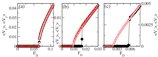
FIG. 18. (Color online) Velocity-force curves \langle V_x \rangle vs F_D for the x -direction depinning (open squares) and \langle V_y \rangle vs F_D for the y -direction depinning (filled circles) in the square pinning lattice system from Fig. 17. (a) B/B_\phi = 2 , where the depinning is isotropic. (b) B/B_\phi = 4 with anisotropic depinning. (c) B/B_\phi = 12 with anisotropic depinning.
