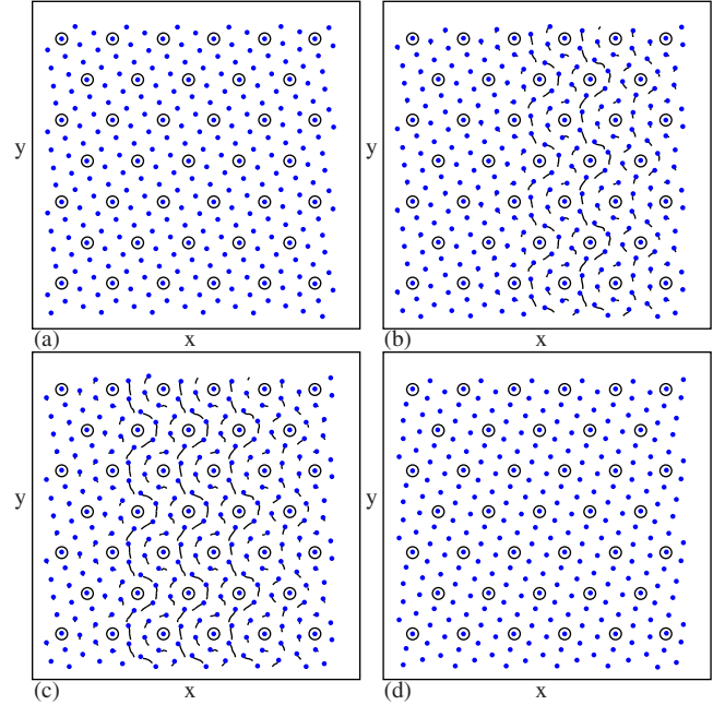
FIG. 9. (Color online) Vortex positions (black dots), pinning site locations (open circles), and vortex trajectories (black lines) for the triangular pinning lattice system in Fig. 2 at B/B_\phi=7 . A weak external driving force is applied at an angle in the positive x - y plane that induces a structural transformation in the vortex lattice between the two ground states, -78^\circ shown in panel (a) and +78^\circ shown in panel (d). During the transformation, illustrated in panels (b) and (c), the interstitial vortices shift in the positive y direction by approximately one lattice constant and a domain wall traverses the system.
