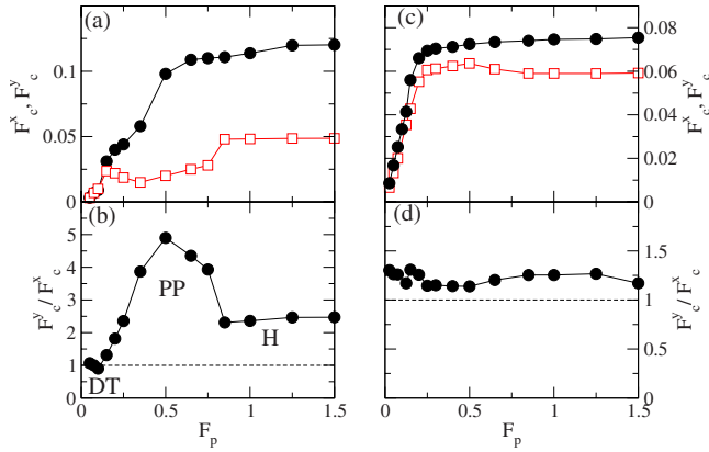
FIG. 10. (Color online) (a) Depinning threshold in the x direction, F_c^x (open squares), and y direction, F_c^y (filled circles), vs F_p for the triangular pinning lattice system in Fig. 2 at B/B_\phi=2 . (b) The corresponding anisotropy ratio F_c^y/F_c^x vs F_p . H: the honeycomb ordering illustrated in Fig. 11(a); PP: the partially pinned phase shown in Fig. 11(b) where a portion of the pinning sites are unoccupied and the depinning is plastic; DT: the distorted triangular phase seen in Fig. 11(c) where most pinning sites are unoccupied and the depinning is elastic. The three different phases are visible as features in the anisotropy. (c) The depinning thresholds F_c^x and F_c^y vs F_p for the same system at B/B_\phi=3 . (d) The corresponding anisotropy ratio F_c^y/F_c^x vs F_p .
