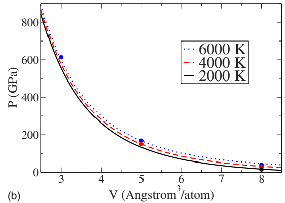
FIG. 8. (Color online) Internal energy and pressure isotherms in the liquid. Lines are the results of the liquid free energy model; dots are the results from ab initio MD.
