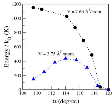
FIG. 3. (Color online) Ground-state energy difference (neglecting zero-point motion) of Be along a 1D slice through the two-dimensional Burgers path for V=7.63 and 3.75 \text{ \AA}^3/\text{atom} .
