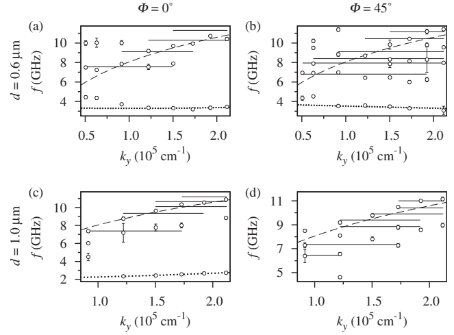
FIG. 5. Spin-wave dispersions in antidot structures at H_{\text{ext}} = 0 \text{ Oe} . (a) and (b) are dispersion data from antidot patterns of d = 0.6 \mu\text{m} at \Phi = 0^\circ and 45^\circ , respectively. (c) and (d) are dispersion data from antidot patterns of d = 1.0 \mu\text{m} at \Phi = 0^\circ and 45^\circ , respectively. (---) is the dispersion curve calculated for a continuous film using Eq. (4). (—) are standing-wave frequencies as observed in micromagnetic simulations. These lines cover the range of k_y in which these fixed-frequency modes are found in simulations. ( \cdots ) are fitted dispersion curves for dipole-exchange backward volume modes using Eq. (6).
