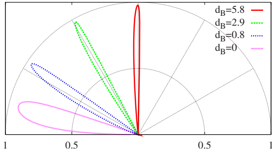
FIG. 9. (Color online) Angular dependence of the transmission probability at E=6 through a structure consisting of one magnetic barrier of width d_B and one magnetic well of width d_{-B} . We fix d_{-B}=11.7 \approx 2E and vary d_B from 0 to 5.8 \approx E .
