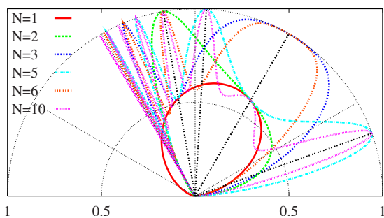
FIG. 10. (Color online) Angular dependence of the transmission probability at E=1 and d_B=d_{-B}=1 for several values of N . The black dashed lines correspond to the angles for recursive transmission of multiplicity 2 (at \phi \approx \pi/18 ), 3 (at \phi = -\pi/6 ), and 5 (at \phi \approx -\pi/54 and \phi \approx -7\pi/18 ).
