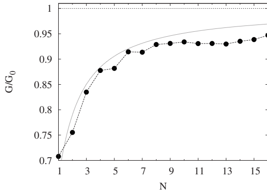
FIG. 4. The conductance G/G_0 at E=1 for several values of N with d_B = 1/N , such that \Phi = 1 , and d_0 = 10 (black dots linked by long-dashed line, which is a guide for the eyes only). The upper bound (dashed line) corresponds to the classical value G_s/G_0 = 1 [see Eq. (16)] while the dotted line is the curve given by Eq. (26) as a function of N .
