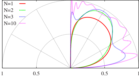
FIG. 3. (Color online) Angular dependence of the transmission probability at E=1 , through N=1, 2, 3, 10 barriers of width d_B = 1/N (keeping in this way constant the flux \Phi = Nd_B = 1 ) and spaced by d_0 = 10 .
