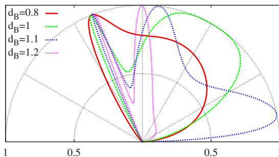
FIG. 14. (Color online) Angular dependence of the transmission probability for several values of d_B=d_{-B} with N=3 and E=1 .
