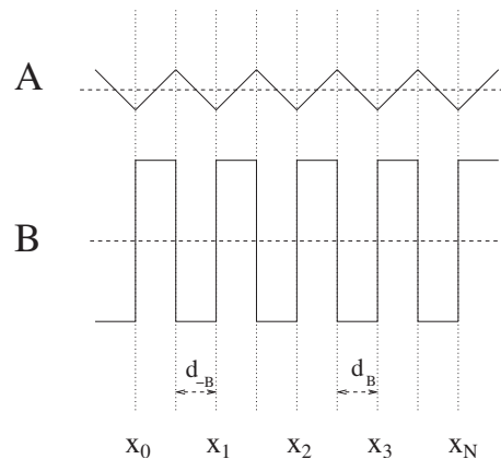
FIG. 16. Periodic superlattice of alternating magnetic barriers and wells with d_B=d_{-B} .
