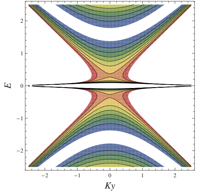
FIG. 18. (Color online) The allowed spectrum, |\text{Tr } \Omega| \leq 2 , varying E and k_y , at d_B=d_{-B}=1 . The contour lines correspond to the values of \text{Tr } \Omega in the interval [-2, 2] at steps of 0.5, increasing from blue (inner dark gray) to red (outer dark gray).
