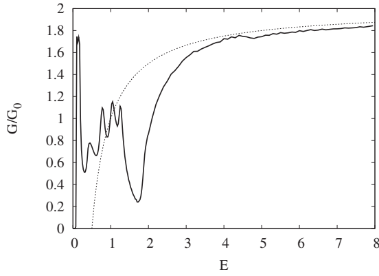
FIG. 13. The conductance G/G_0 as a function of the energy E for N=6 with d_B=d_{-B}=1 (solid line). The dashed line is the classical limit, i.e., (2-d_B/E)\theta(2E-d_B) .
