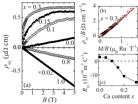
FIG. 3. (Color online) (a) Field dependence of the Hall resistivity \rho_{xy}(B) of various compositions at T=2 K. (b) \rho_{xy}/B vs M/B plot for the sample with x=0.3 , which is a typical sample showing AHE. The solid line represents the least-squares fitting to Eq. (1). (c) Normal Hall coefficient R_0 as a function of x . R_0 is determined by fitting the data to Eq. (1) for 0.1 \leq x < 0.4 .
