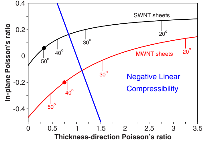
FIG. 8. (Color online) The relationships between in-plane and thickness-direction Poisson's ratios as a function of indicated average nanotube orientation angle \gamma for SWNT and MWNT sheets having the force constant ratios r that yield the measured Poisson's ratios (circles). The straight (blue) line represents the equation 1 - \nu_1 - \nu_3 = 0 . Values of \gamma on the right side of this line are predicted to produce negative linear compressibilities for SWNT and MWNT sheets.
