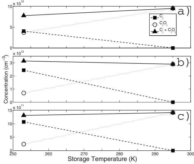
FIG. 4. Concentrations of C_i and C_iO_i (dotted lines), and their sum (solid line) measured after the -20 °C and RT storages for the highest irradiated dose in (a) 2 \times 10^{15} , (b) 2 \times 10^{14} , and (c) 6 \times 10^{13} B\text{ cm}^{-3} epitaxial samples. The time elapsed from the start of the irradiations at RT to the -20 °C storage was less than 1 h.
