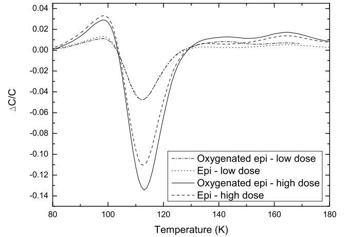
FIG. 6. MCTS spectra of oxygenated and nonoxygenated epitaxial samples ( [B_s] \approx 2 \times 10^{15} \text{ cm}^{-3} ) irradiated by protons with low ( 2 \times 10^{12} \text{ cm}^{-2} ) and high ( 4 \times 10^{12} \text{ cm}^{-2} ) doses.
