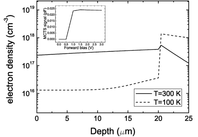
FIG. 1. Simulations of the steady-state electron density during the filling pulse in the MCTS measurements using a boron concentration of 2 \times 10^{15} \text{ cm}^{-3} and a forward bias of 3 V. The inset shows the measured MCTS intensity of the E_c - 0.25 \text{ eV} level versus forward bias pulse, illustrating the saturation of the MCTS signal.
