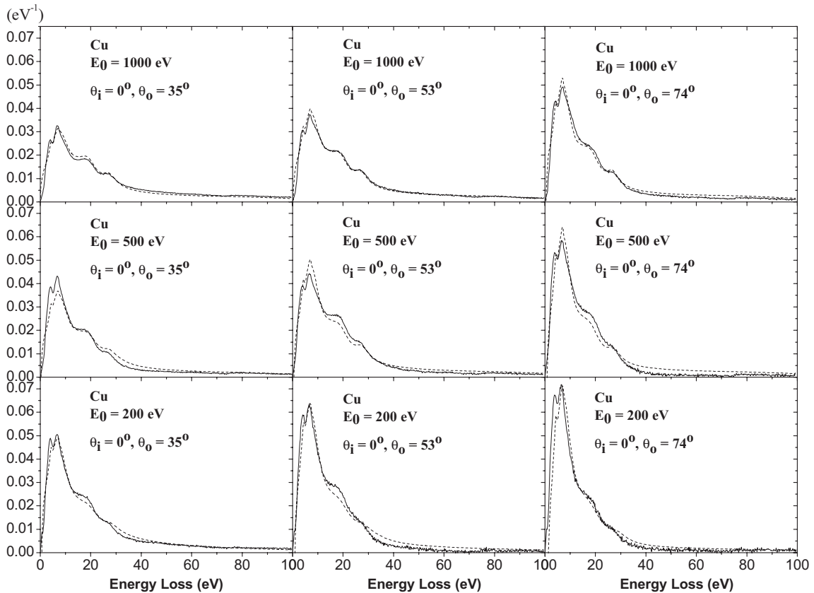
FIG. 7. \lambda^*K_{\text{exp}} (solid line) and \lambda^*K_{\text{th}} (dashed line).
