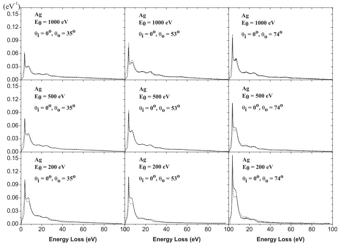
FIG. 5. \lambda^*K_{exp} (solid line) and \lambda^*K_{th} (dashed line).
