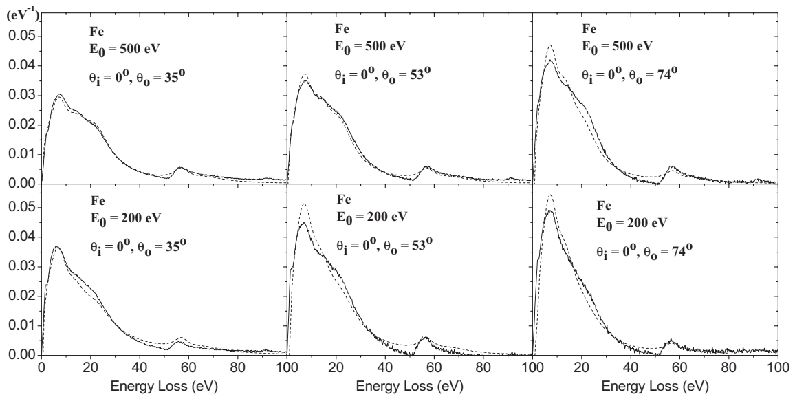
FIG. 8. \lambda^*K_{\text{exp}} (solid line) and \lambda^*K_{\text{th}} (dashed line).
