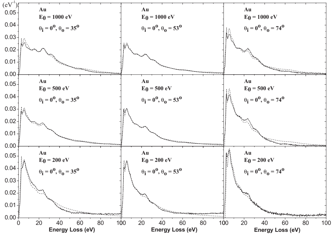
FIG. 6. \lambda^*K_{\text{exp}} (solid line) and \lambda^*K_{\text{th}} (dashed line).
